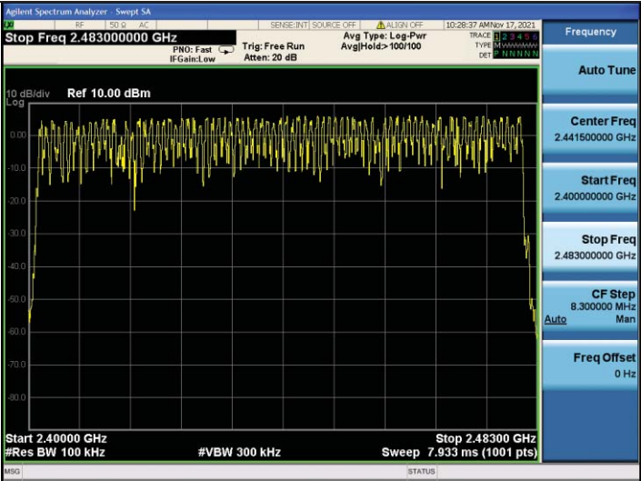
8DPSK Modulation
