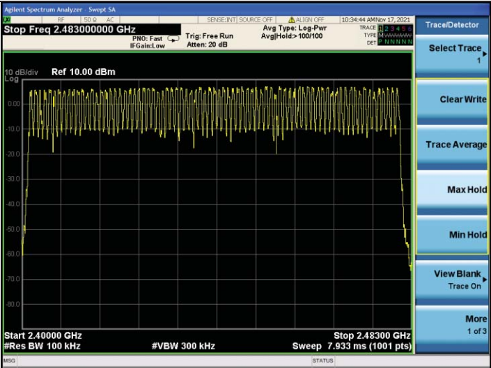
GFSK Modulation
