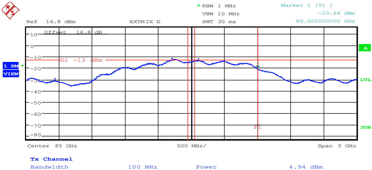
Figure 8.5-1: PSD sample plot
