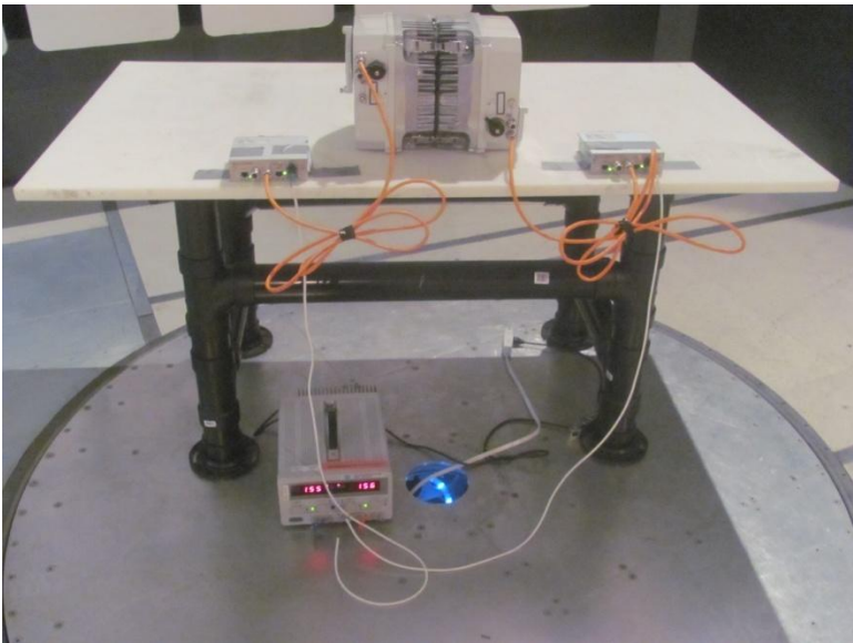
Figure 3.6-1: Setup diagram
