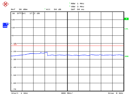
LTE Band 5 1.4MHz CH-High 1GHz~9GHz
