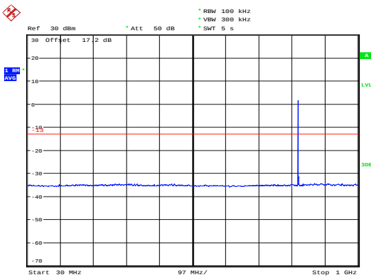
LTE Band 5 1.4MHz CH-Low 30MHz~1GHz
