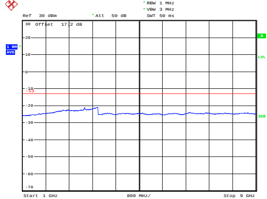
LTE Band 5 1.4MHz CH-Low 1GHz~9GHz
