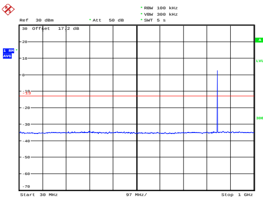
LTE Band 5 1.4MHz CH-High 30MHz~1GHz
