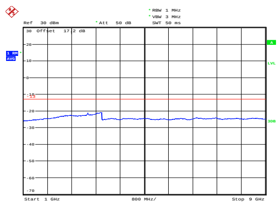
LTE Band 5 1.4MHz CH-Middle 1GHz~9GHz
