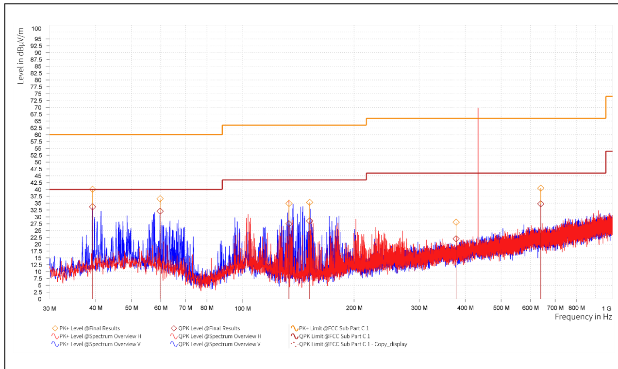
30 MHz – 1 GHz
