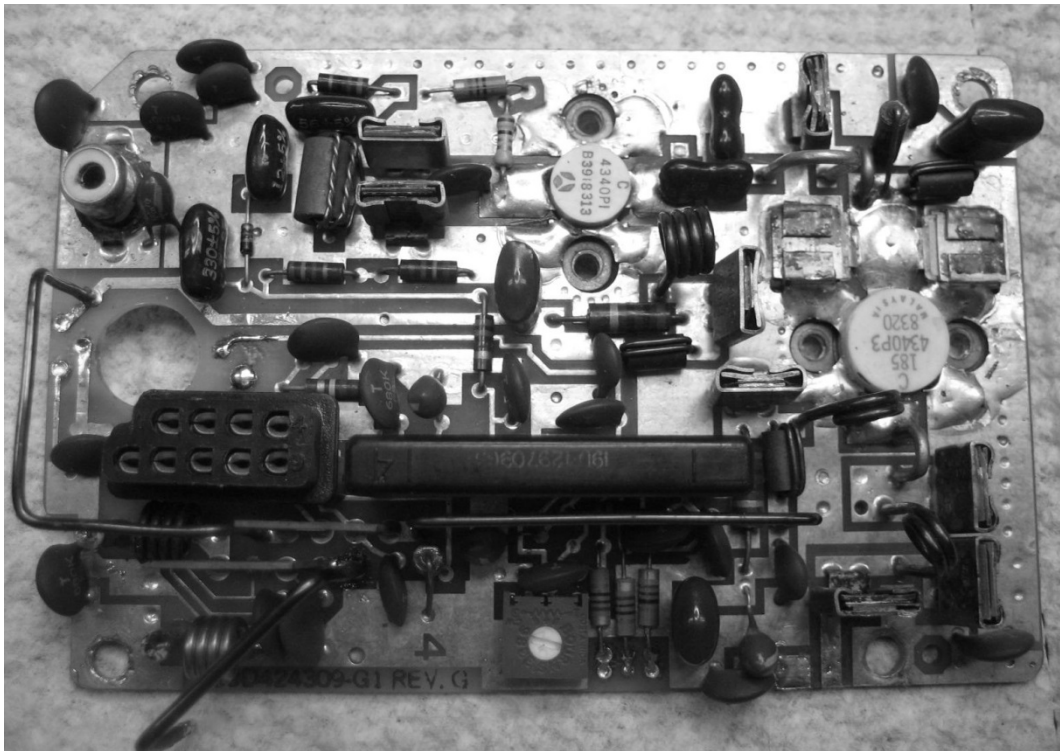
BOTTOM VIEW
