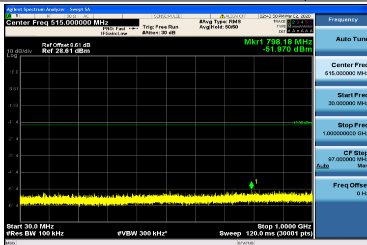
Band2-10MHz-16QAM-18650-1RB#0-30~1000MHz
