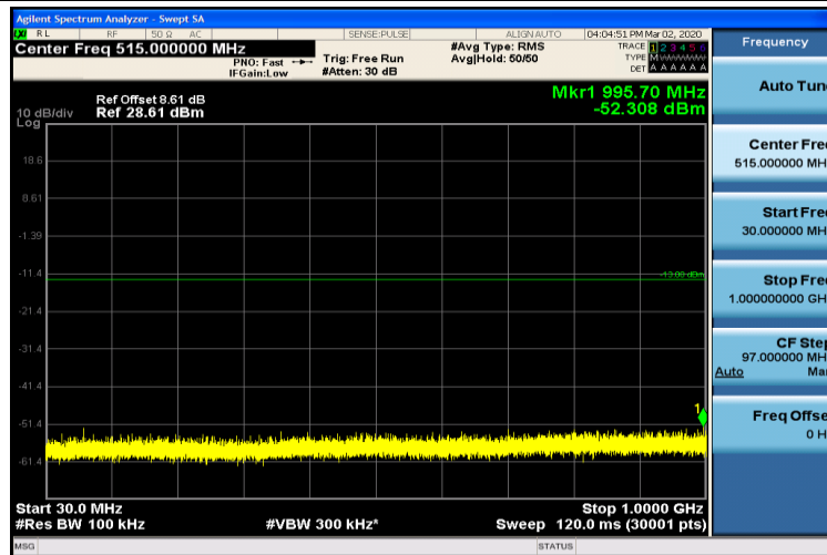
Band4-10MHz-16QAM-20000-1RB#0-30~1000MHz
