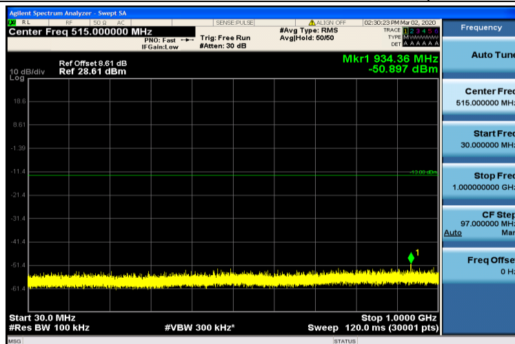
Band2-5MHz-16QAM-18625-1RB#0-30~1000MHz
