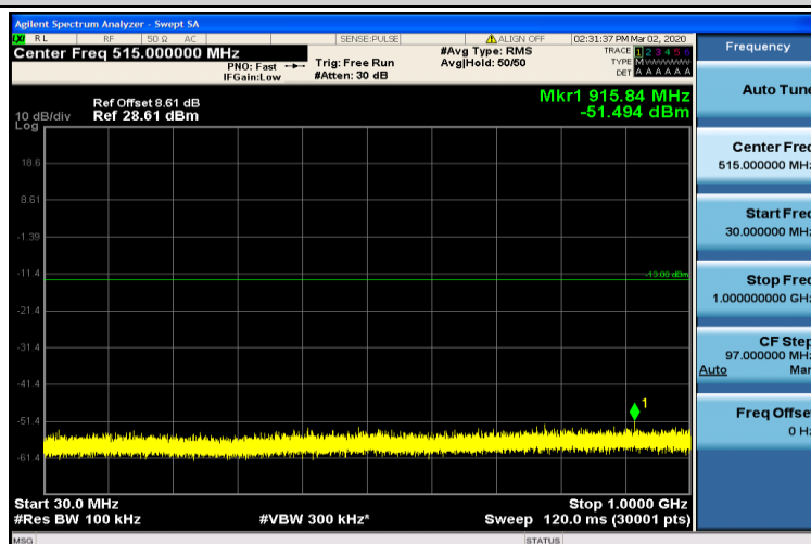
Band2-5MHz-16QAM-18900-1RB#0-30~1000MHz
