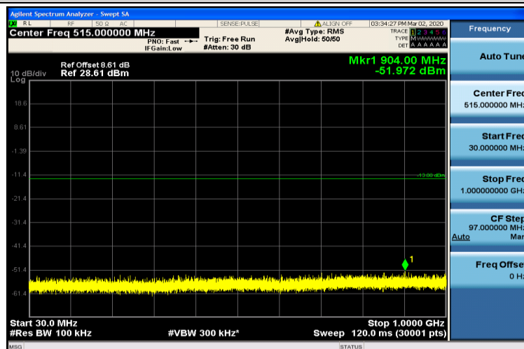
Band4-5MHz-QPSK-20175-1RB#0-30~1000MHz
