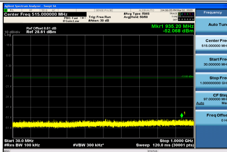
Band4-10MHz-16QAM-20175-1RB#0-30~1000MHz
