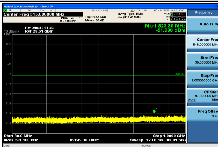
Band2-10MHz-16QAM-19150-1RB#0-30~1000MHz
