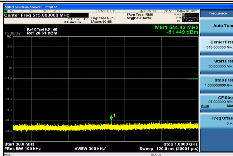
Band4-1.4MHz-16QAM-20393-1RB#0-30~1000MHz
