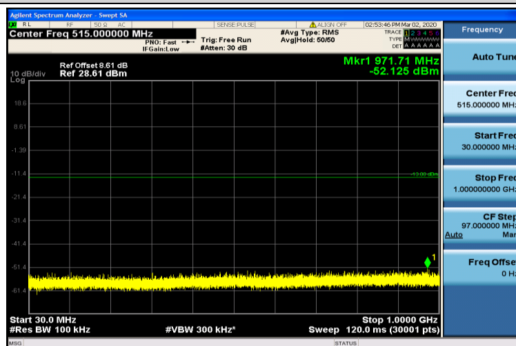
Band2-15MHz-16QAM-19125-1RB#0-30~1000MHz
