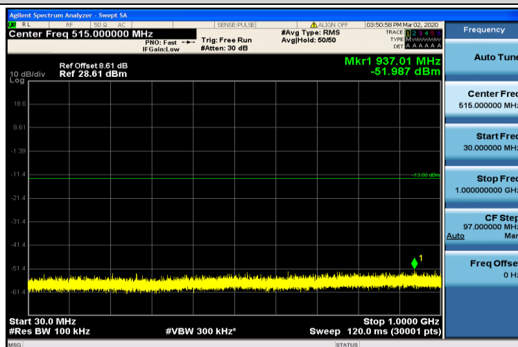
Band4-1.4MHz-16QAM-20175-1RB#0-30~1000MHz
