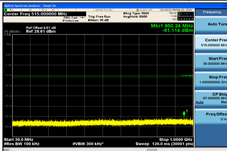
Band4-1.4MHz-16QAM-19957-1RB#0-30~1000MHz
