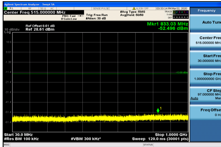
Band4-5MHz-QPSK-19975-1RB#0-30~1000MHz
