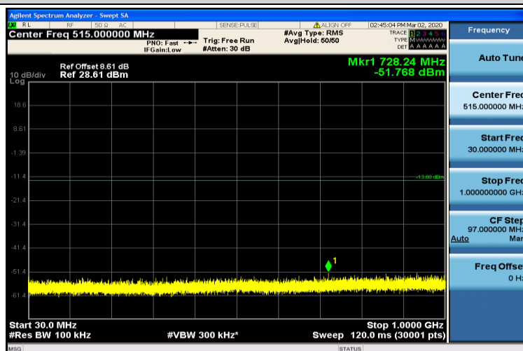
Band2-10MHz-16QAM-18900-1RB#0-30~1000MHz
