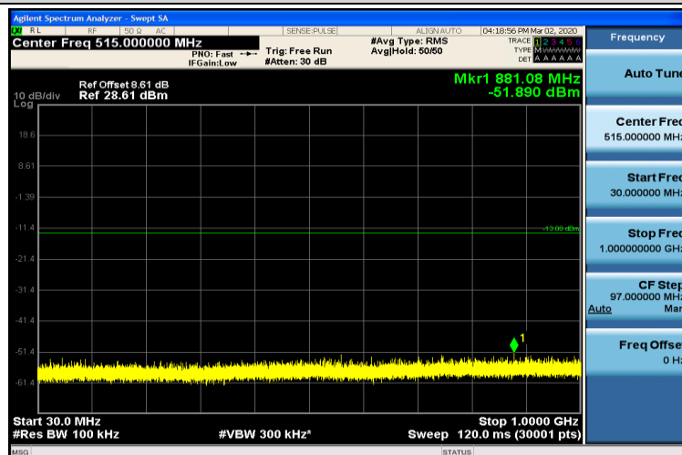
Band4-3MHz-QPSK-20175-1RB#0-30~1000MHz
