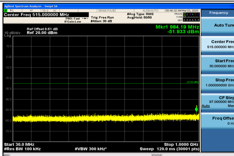
Band7-10MHz-QPSK-21100-1RB#0-30~1000MHz
