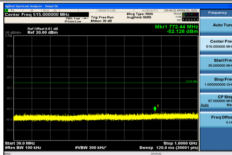
Band7-10MHz-16QAM-21400-1RB#0-30~1000MHz
