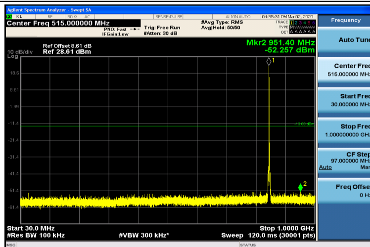
Band5-1.4MHz-QPSK-20643-1RB#0-30~1000MHz
