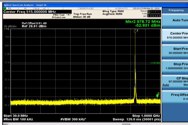
Band5-3MHz-16QAM-20525-1RB#0-30~1000MHz
