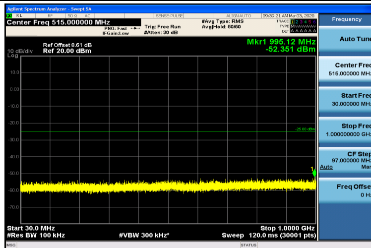
Band7-5MHz-QPSK-21425-1RB#0-30~1000MHz
