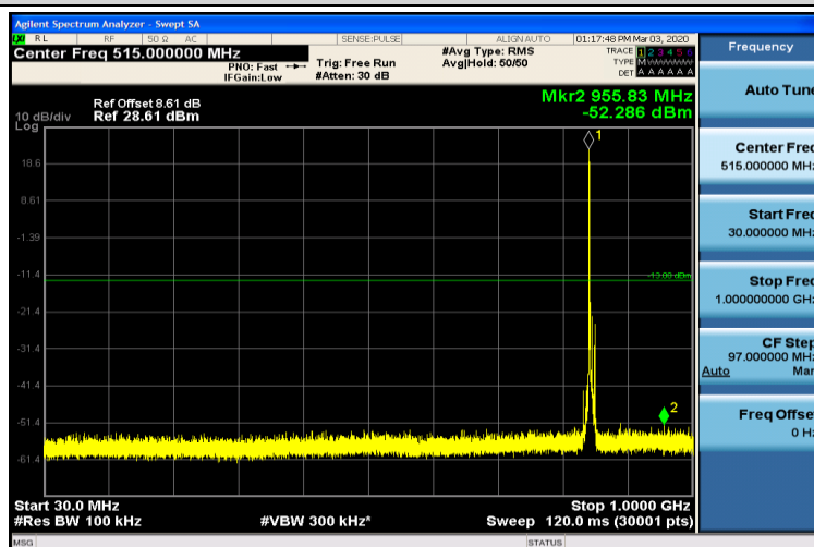
Band5-5MHz-QPSK-20625-1RB#0-30~1000MHz
