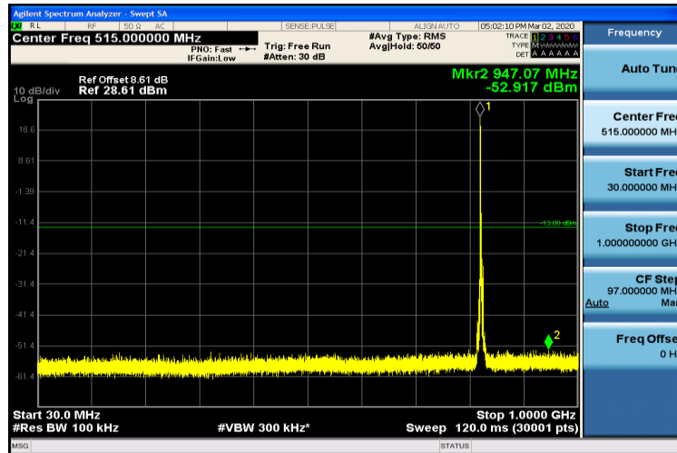
Band5-3MHz-16QAM-20415-1RB#0-30~1000MHz
