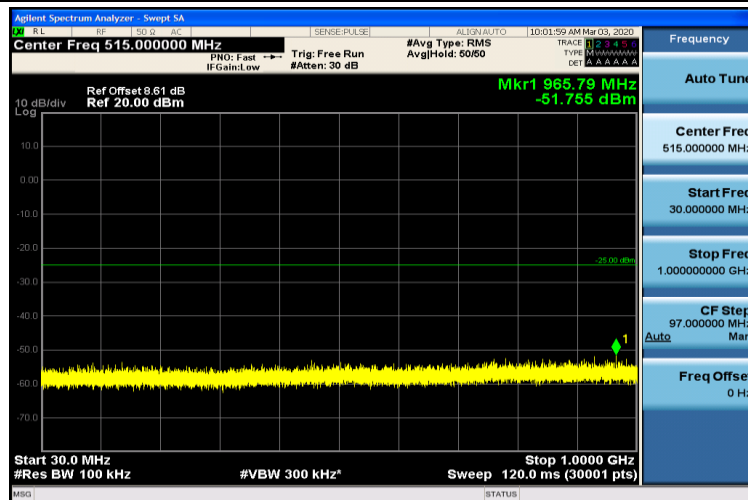
Band7-15MHz-16QAM-21375-1RB#0-30~1000MHz
