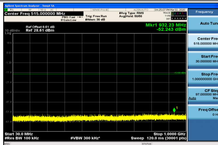
Band4-20MHz-16QAM-20300-1RB#0-30~1000MHz
