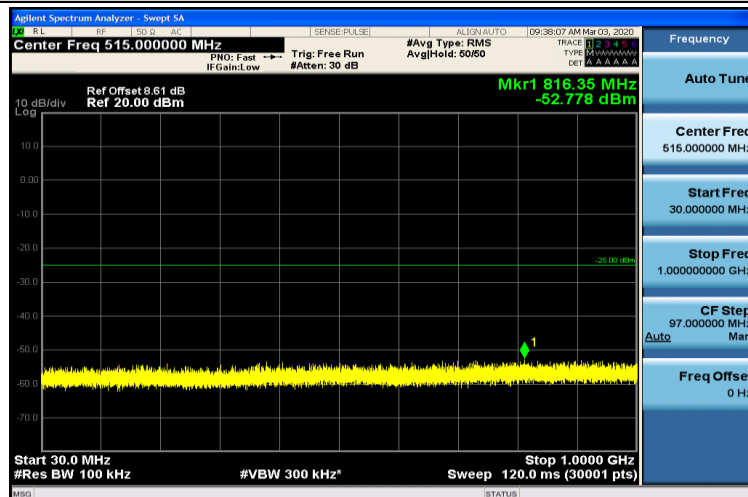
Band7-5MHz-QPSK-21100-1RB#0-30~1000MHz
