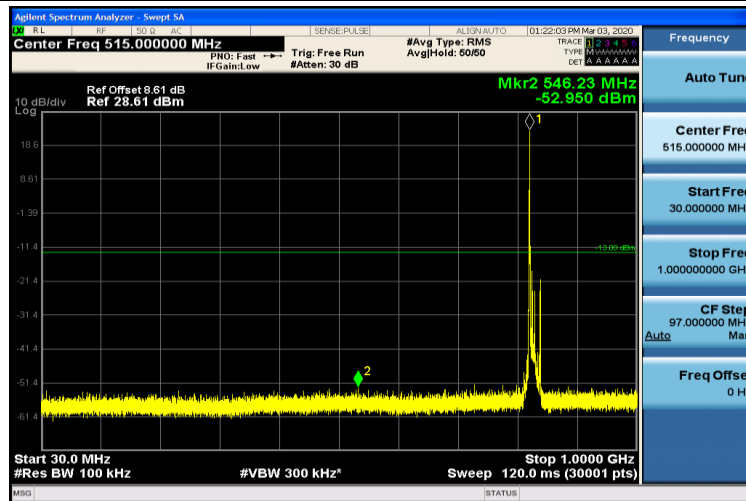
Band5-10MHz-16QAM-20450-1RB#0-30~1000MHz
