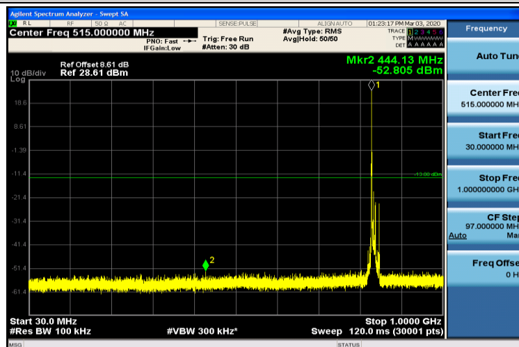
Band5-10MHz-16QAM-20525-1RB#0-30~1000MHz
