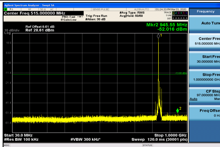
Band5-10MHz-16QAM-20600-1RB#0-30~1000MHz
