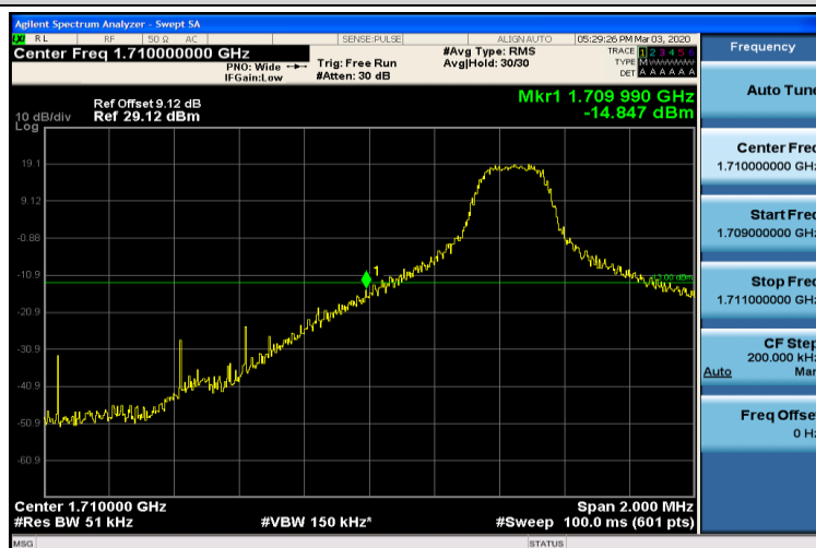
Band4-5MHz-QPSK-19975-1RB#0
