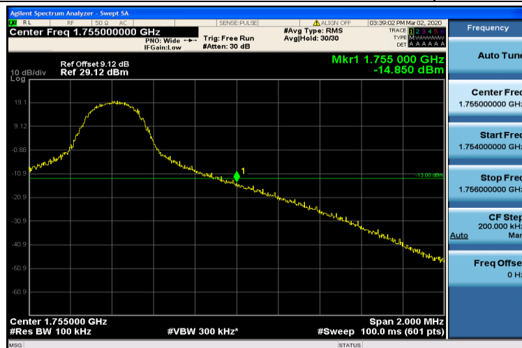
Band4-10MHz-16QAM-20350-1RB#49
