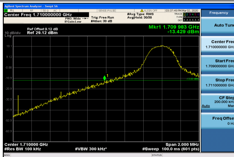
Band4-10MHz-16QAM-20000-1RB#0
