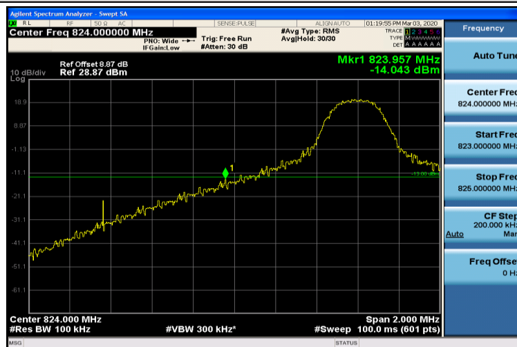
Band5-10MHz-16QAM-20450-1RB#0
