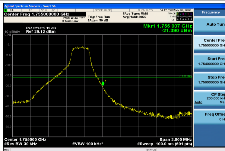
Band4-3MHz-QPSK-20385-1RB#14
