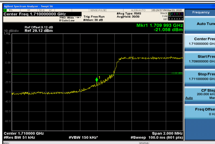
Band4-5MHz-QPSK-19975-25RB#0
