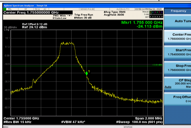
Band4-1.4MHz-16QAM-20393-1RB#5
