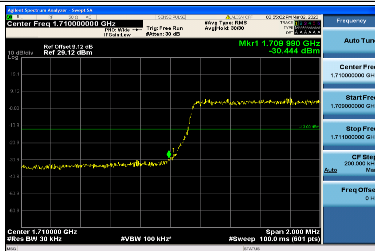
Band4-3MHz-16QAM-19965-15RB#0
