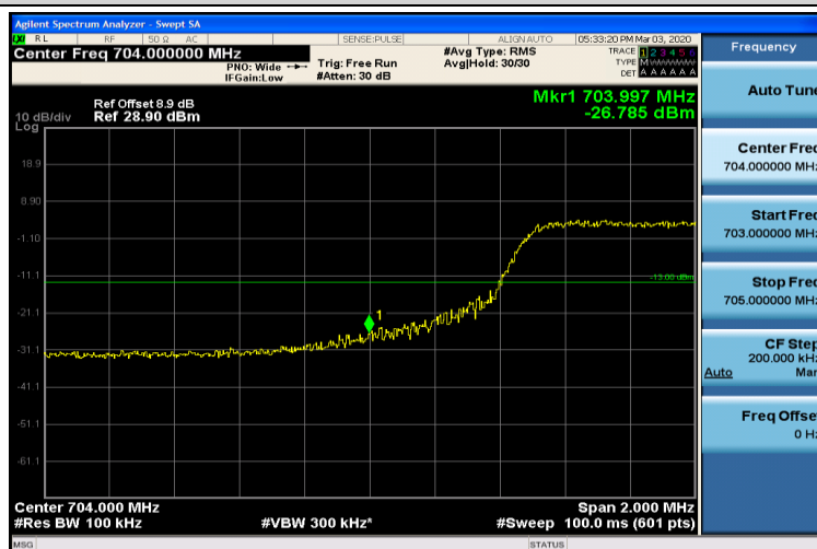
Band17-10MHz-16QAM-23780-50RB#0
