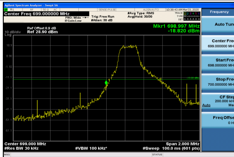
Band12-3MHz-QPSK-23025-1RB#0
