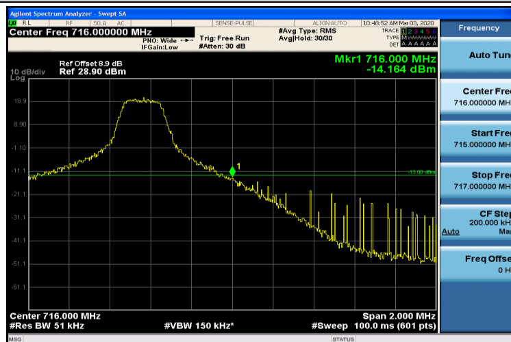
Band12-5MHz-QPSK-23155-1RB#24
