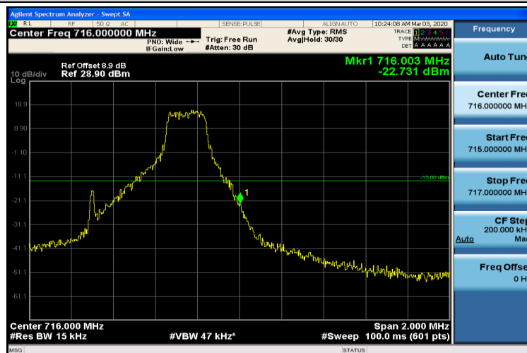
Band12-1.4MHz-16QAM-23173-1RB#5
