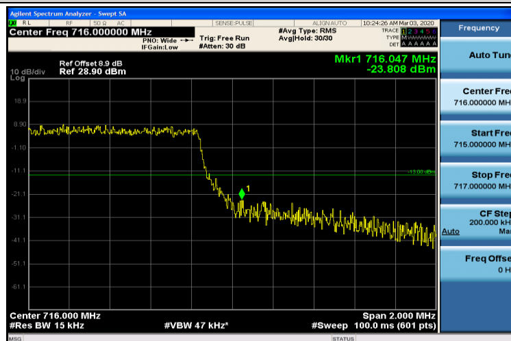
Band12-1.4MHz-16QAM-23173-6RB#0
