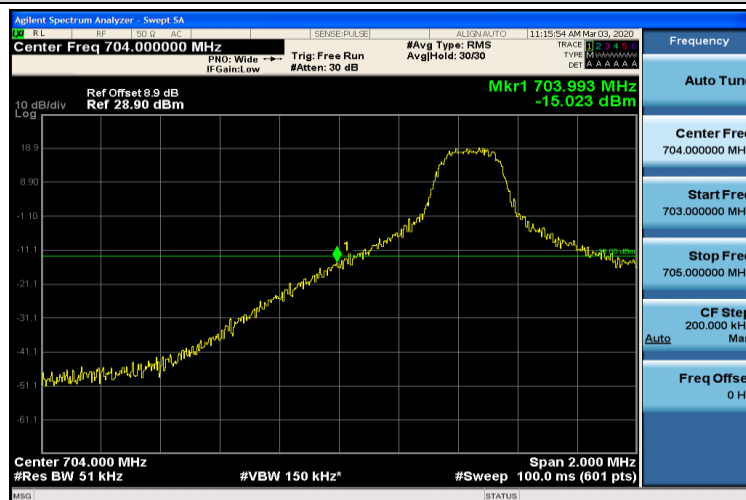
Band17-5MHz-16QAM-23755-1RB#0
