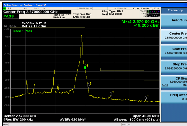
Band7-20MHz-QPSK-21350-1RB#99
