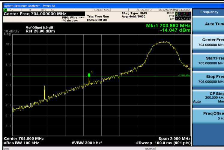
Band17-10MHz-16QAM-23780-1RB#0
