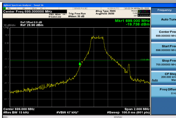
Band12-1.4MHz-QPSK-23017-1RB#0
