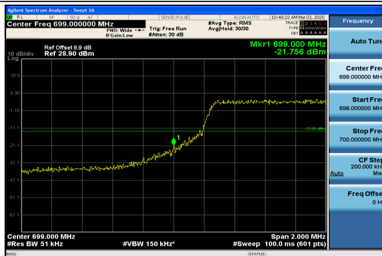
Band12-5MHz-16QAM-23035-25RB#0
