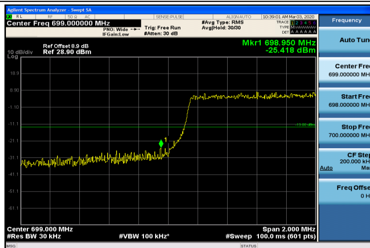
Band12-3MHz-QPSK-23025-15RB#0
