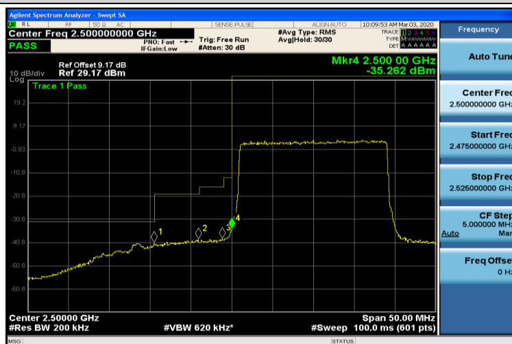
Band7-20MHz-16QAM-20850-100RB#0
