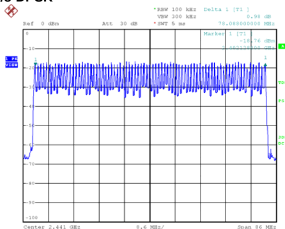
GFSK/ Pi/4DQPSK/8-DPSK
