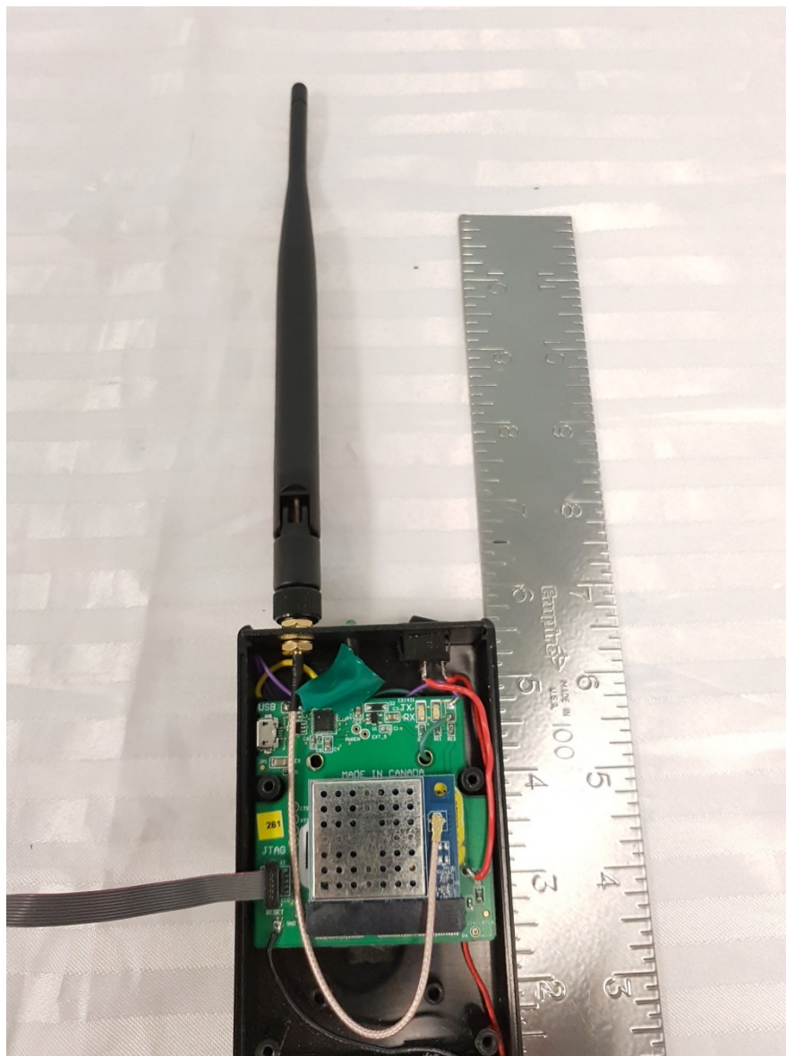
Figure 1 – EUT External Photo with Shield and Antenna (Installed on Development Board)
