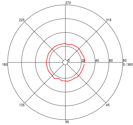
Turntable Plot ( 30.044488978 MHz )
