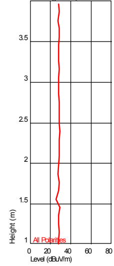
Height Plot ( 541.505611309 MHz )
