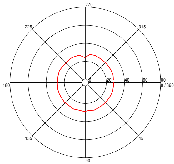
Turntable Plot ( 539.565530868 MHz )
