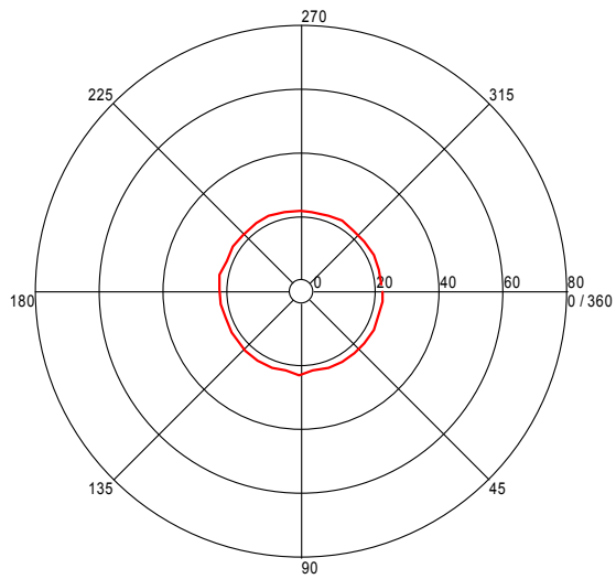
Turntable Plot ( 407.925650902 MHz )
