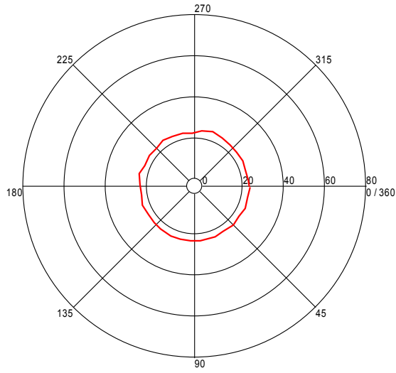
Turntable Plot ( 31.982565411 MHz )
