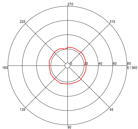
Turntable Plot ( 423.674148747 MHz )
