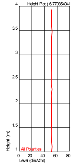
Height Plot ( 6.770354041 GHz )
