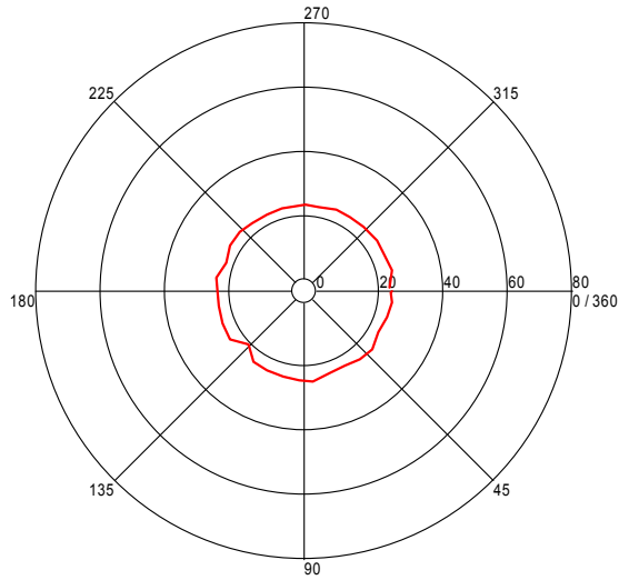
Turntable Plot ( 30.170140337 MHz )
