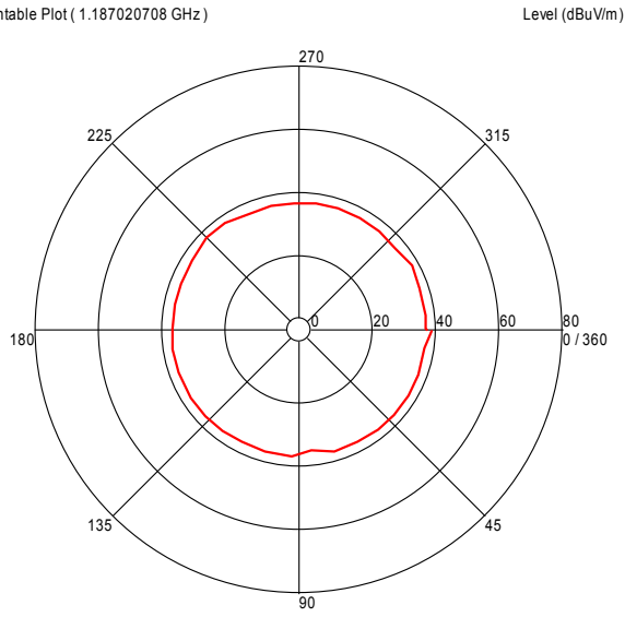
Turntable Plot ( 1.187020708 GHz )
