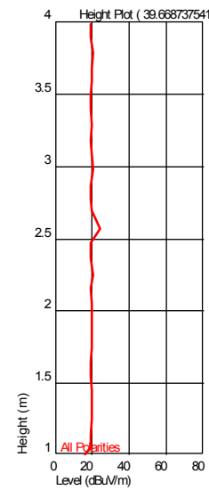
Height Plot ( 39.668737541 MHz )
