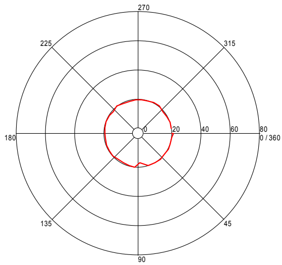
Turntable Plot ( 262.723046026 MHz )
