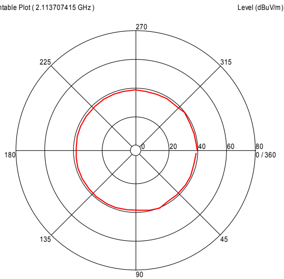
Turntable Plot ( 2.113707415 GHz )
