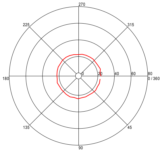
Turntable Plot ( 436.040681216 MHz )
