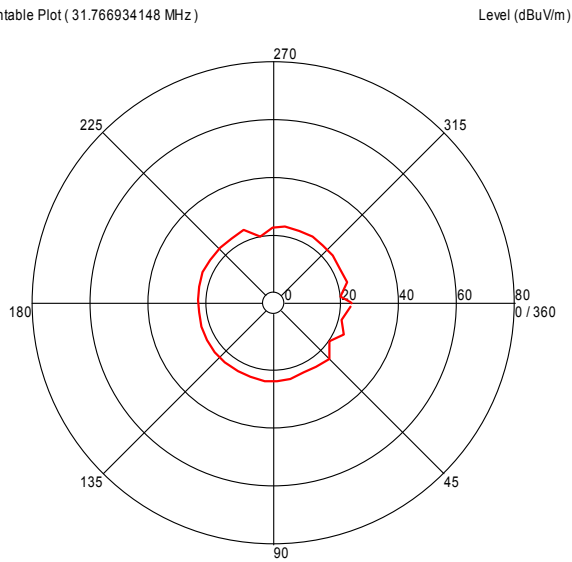
Turntable Plot ( 31.766934148 MHz )
