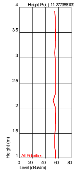
Height Plot ( 11.277388109 GHz )
