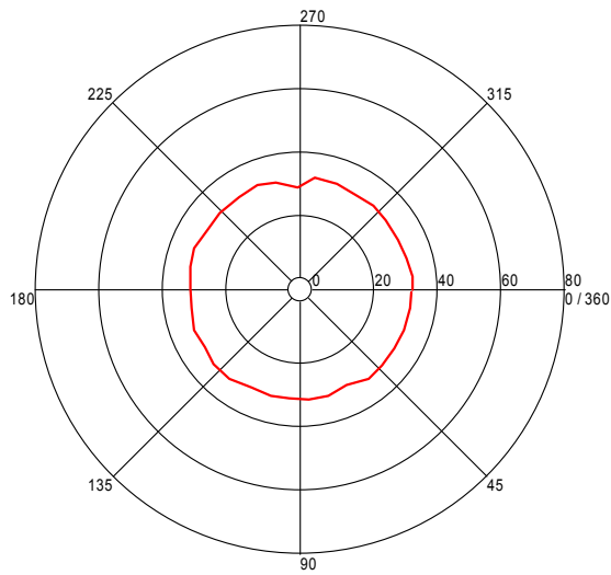
Turntable Plot ( 968.737475359 MHz )
