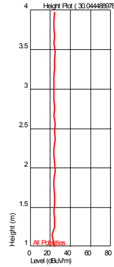
Height Plot ( 30.044488978 MHz )
