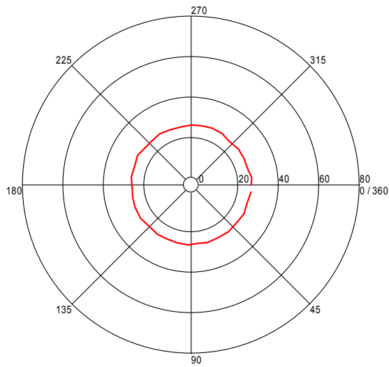
Turntable Plot ( 573.626051838 MHz )
