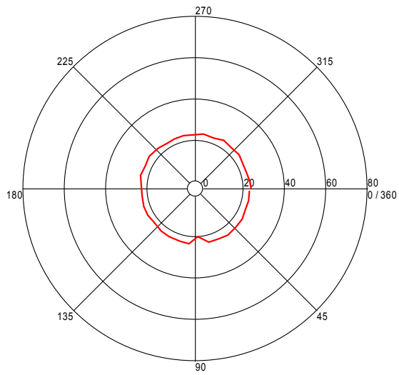
Turntable Plot ( 417.984568972 MHz )
