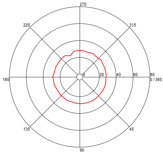
Turntable Plot ( 537.848095886 MHz )
