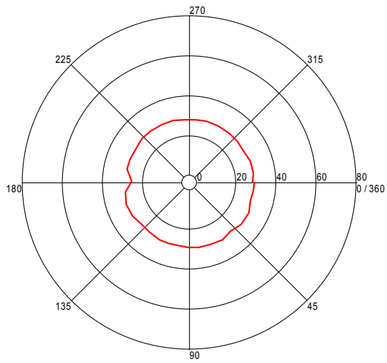
Turntable Plot ( 756.134067912 MHz )
