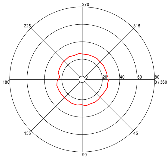
Turntable Plot ( 582.250099944 MHz )
