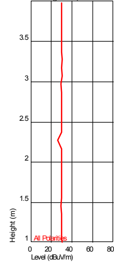
Height Plot ( 903.84108211 MHz )
