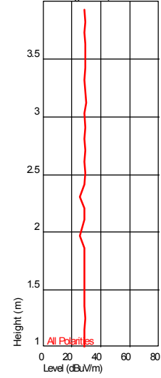
Height Plot ( 756.134067912 MHz )
