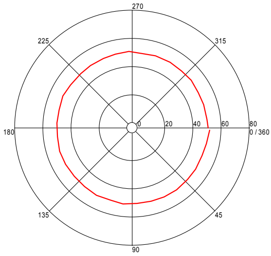
Turntable Plot ( 5.201055445 GHz )
