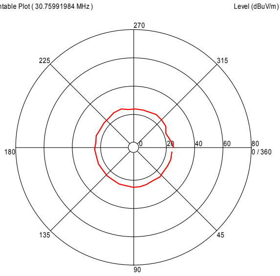
Turntable Plot ( 30.75991984 MHz )
