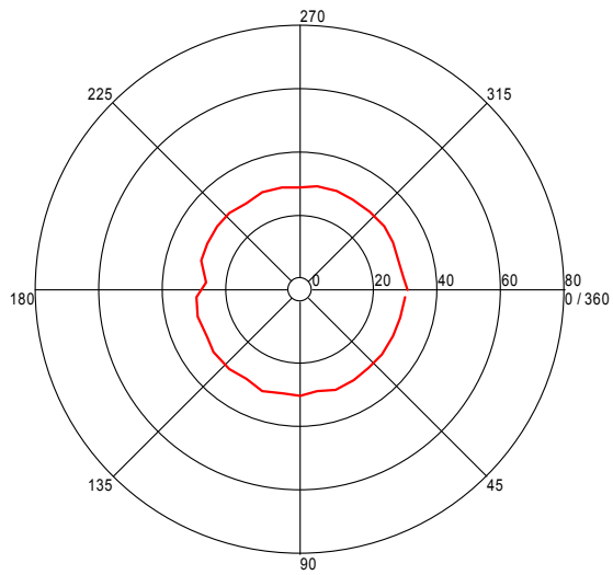
Turntable Plot ( 903.84108211 MHz )
