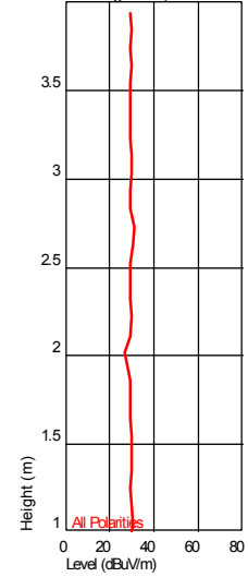
Height Plot ( 859.114428529 MHz )
