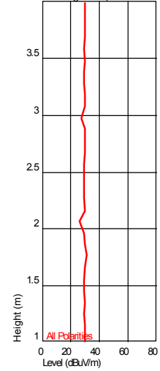
Height Plot ( 839.309419321 MHz )
