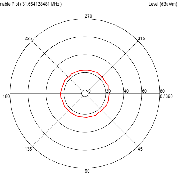
Turntable Plot ( 31.664128481 MHz )
