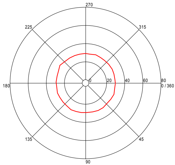
Turntable Plot ( 839.309419321 MHz )
