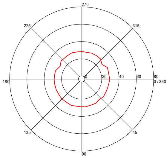
Turntable Plot ( 540.886573176 MHz )
