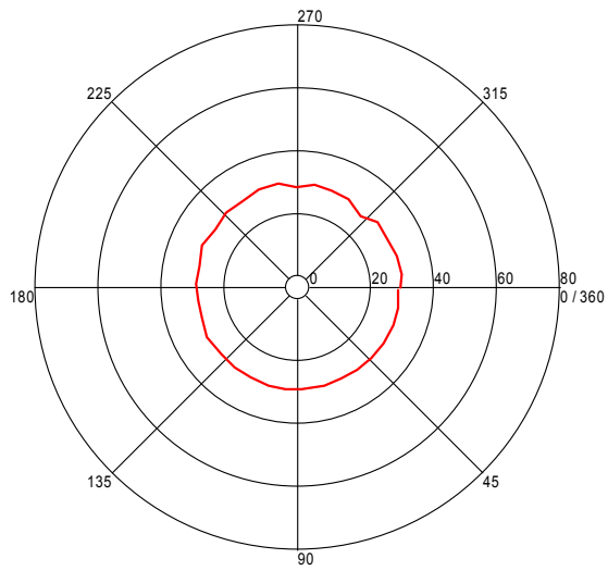
Turntable Plot ( 750.838477224 MHz )
