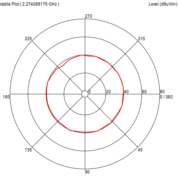
Turntable Plot ( 2.274088176 GHz )
