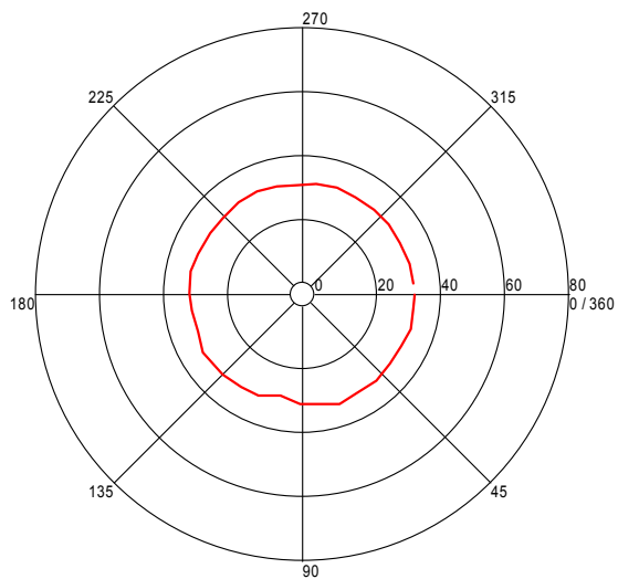
Turntable Plot ( 950.169539355 MHz )
