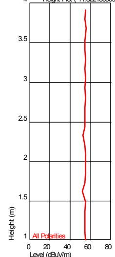
Height Plot ( 11.322150969 GHz )
