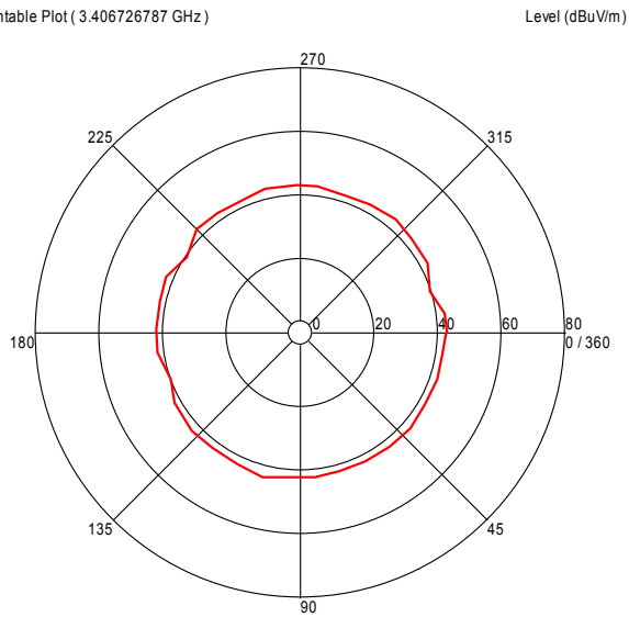
Turntable Plot ( 3.406726787 GHz )
