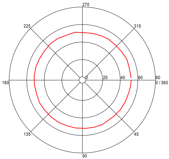
Turntable Plot ( 5.250207081 GHz )
