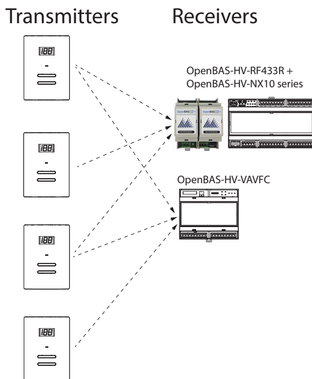
Figure 6 Wireless communication
