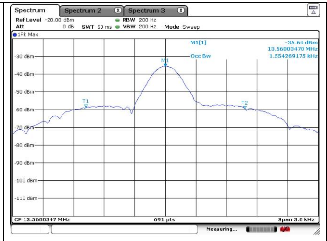
99 % Bandwidth
