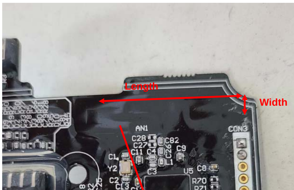
BT Printed Pattern Antenna
