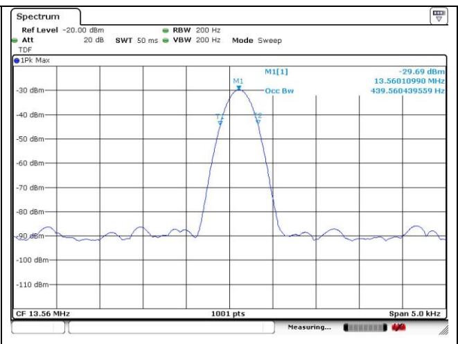
99 % Bandwidth
