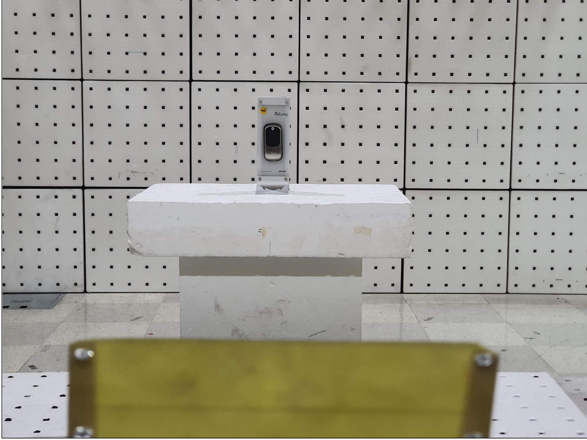
Radiated Emission (Above 1 GHz) _ Front_ (Test Model : YRD642-ACC)
