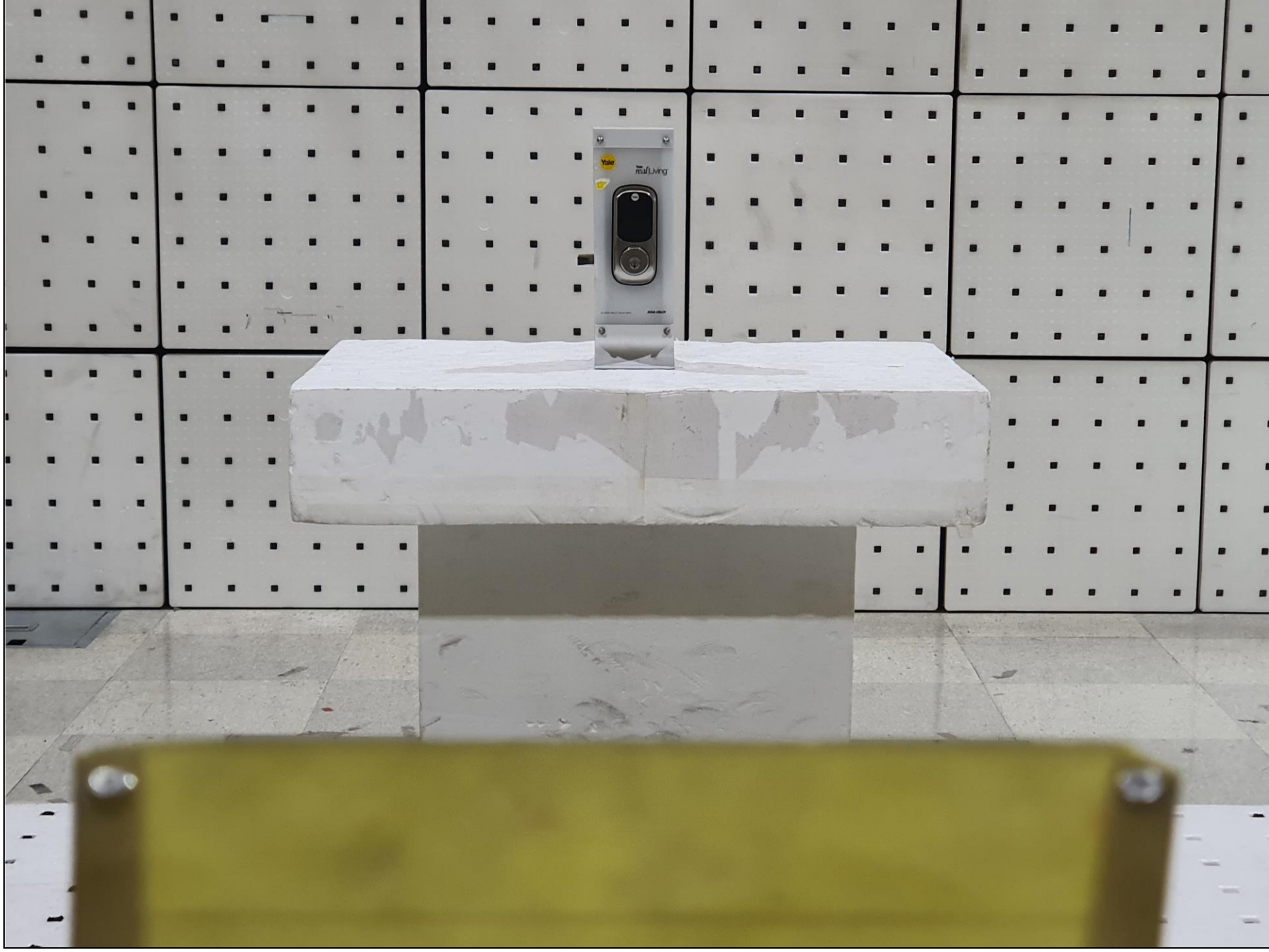
Radiated Emission (Above 1 GHz) _ Front_(Test Model : YRD622-ACC)
