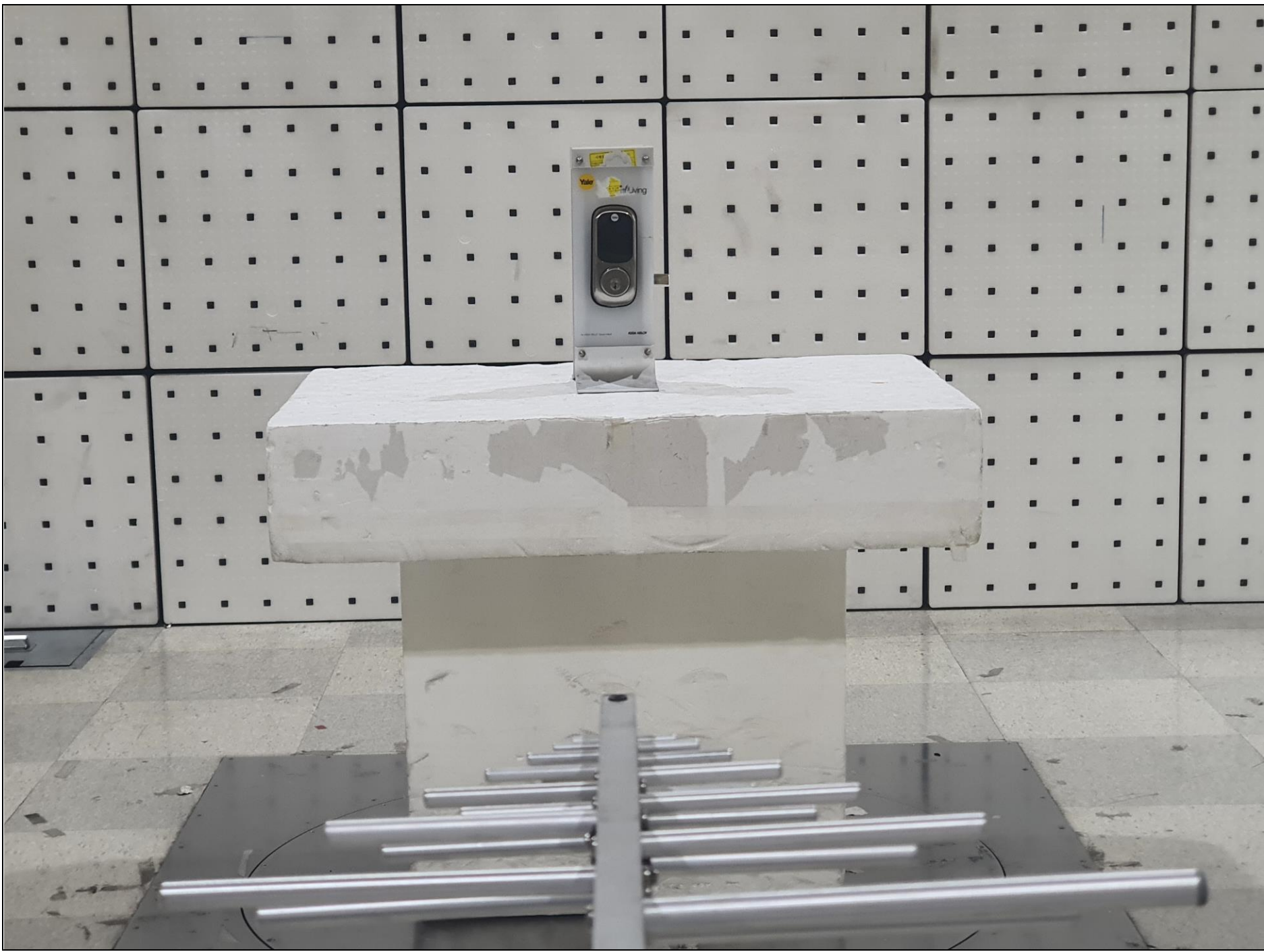
Radiated Emission (Below 1 GHz) _ Front_ (Test Model : YRD622-ACC)
