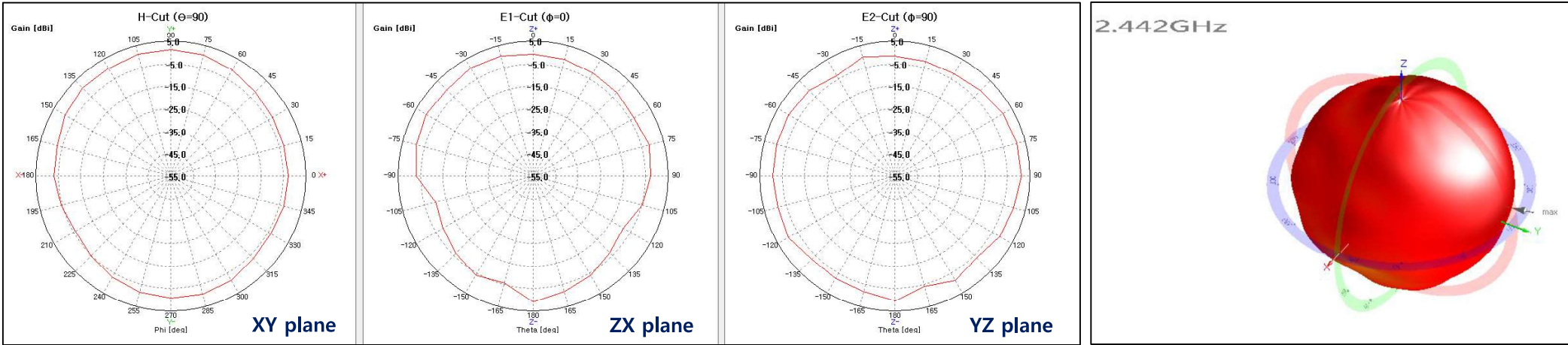
2D / 3D radiation pattern @2442MHz
