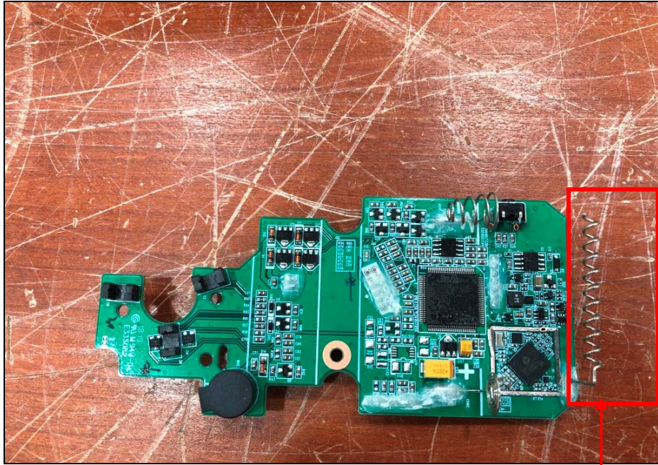
Helical Antenna
