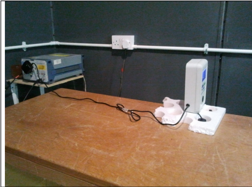
Fig 5 Test setup
