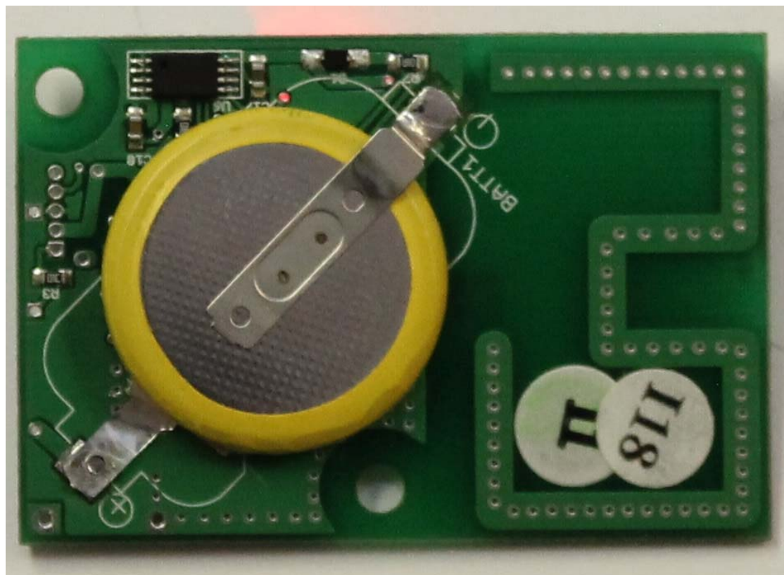
Tag pcb photo Rear
