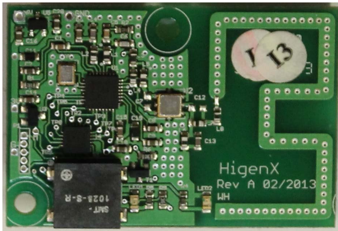
Tag pcb photo Front
