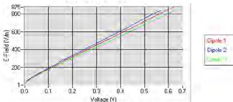
Calibration curves
