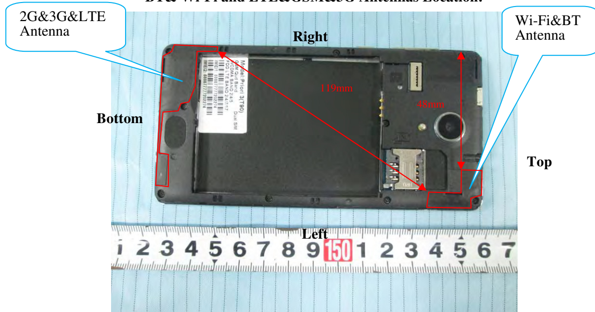
BT& Wi-Fi and LTE&GSM&3G Antennas Location:
