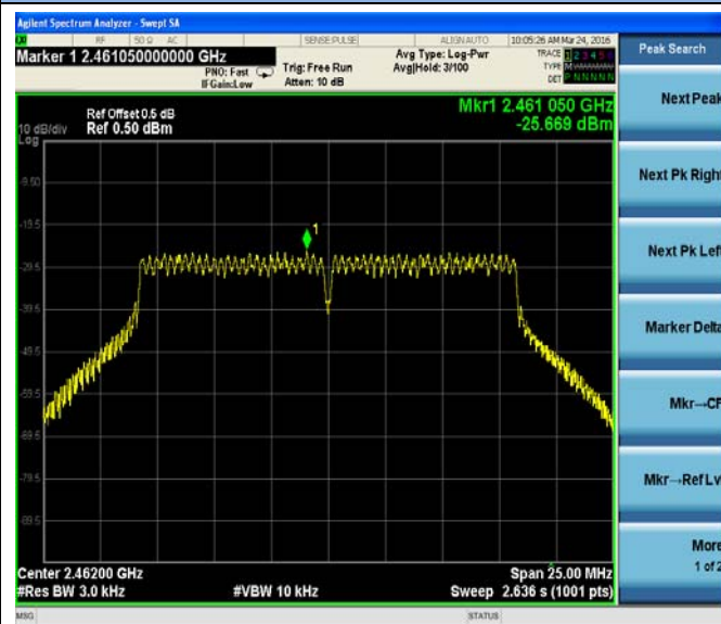
802.11g-High Channel, 2462MHz
