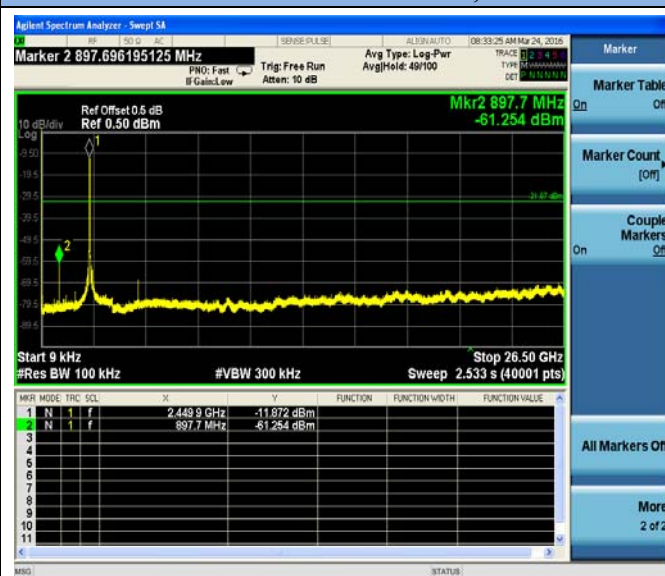
802.11n-HT40-High Channel, 2452MHz
