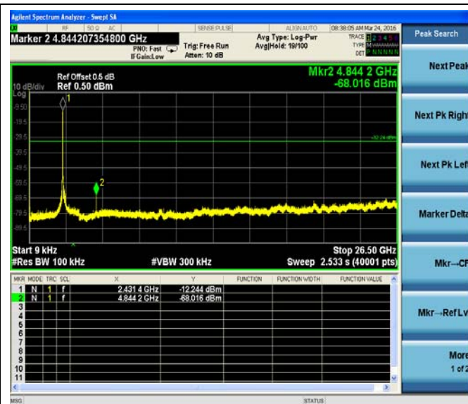
802.11n-HT40-Low Channel, 2422MHz
