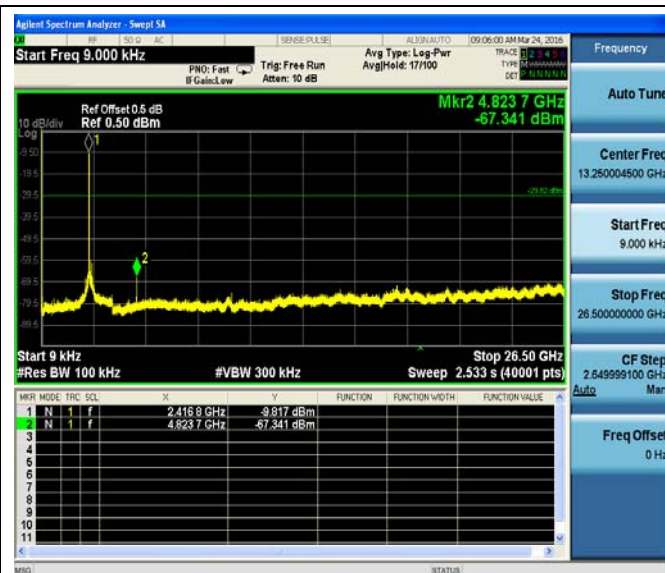
802.11g-Low Channel, 2412MHz
