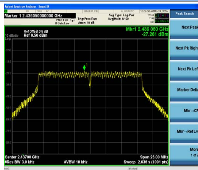
802.11g-Middle Channel, 2437MHz
