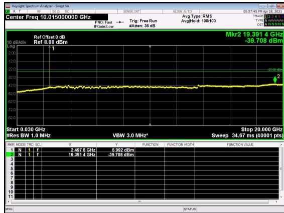
N41(60M)_DFT-s-OFDM_BPSK_Edge_1R B_Left_Low_CH
