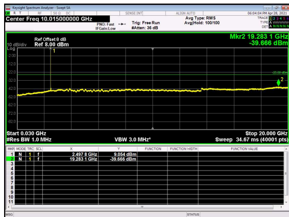
N41(60M)_DFT-s-OFDM_QPSK_Edge_1R B_Left_Low_CH
