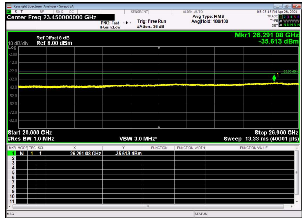
N41(60M)_DFT-s-OFDM_BPSK_Edge_1R B_Left_Low_CH
