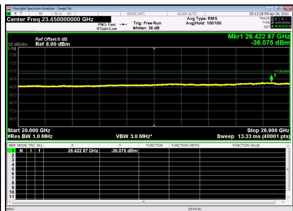
N41(60M)_DFT-s-OFDM_BPSK_Edge_1R B_Left_Mid_CH
