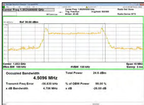
N2(5M)_DFT-s-OFDM_16QAM_Outer_Full_Low_CH
