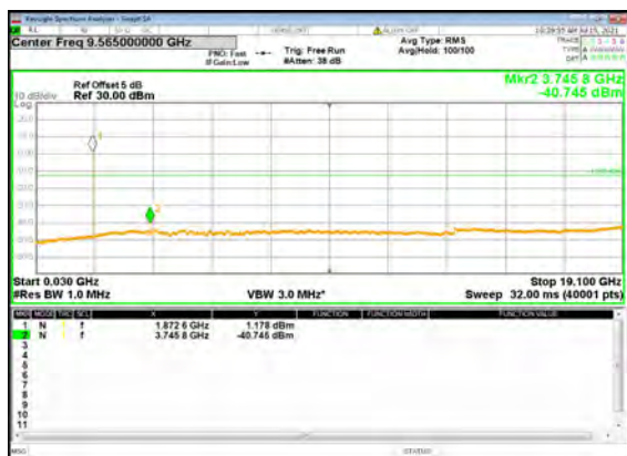
N2(15M)_DFT-s-OFDM_BPSK_Edge_1RB_ Left_Mid_CH
