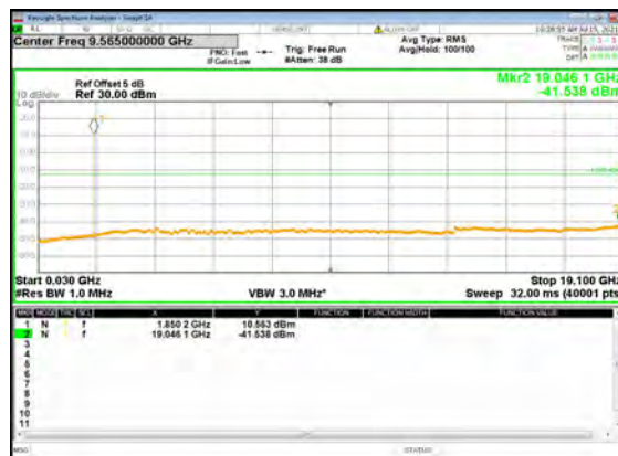
N2(15M)_DFT-s-OFDM_QPSK_Edge_1RB_ Left_Low_CH
