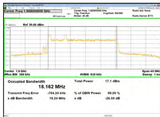
B13_N2(20M)_DFT-s-OFDM_64 QAM_Outer_Full_High_CH
