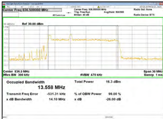
B2_N5(15M)_DFT-s-OFDM_256 QAM_Outer_Full_Mid_CH
