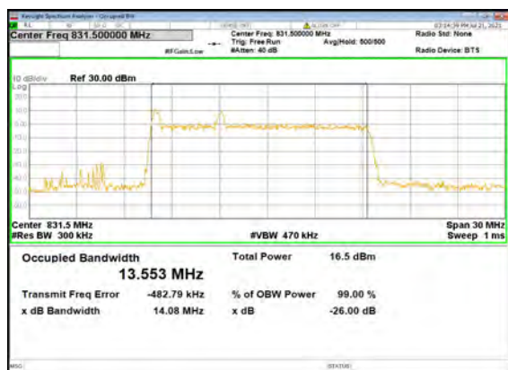
B2_N5(15M)_DFT-s-OFDM_16 QAM_Outer_Full_Low_CH
