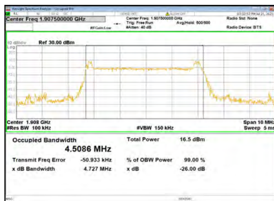
B13_N2(5M)_DFT-s-OFDM_64 QAM_Outer_Full_High_CH
