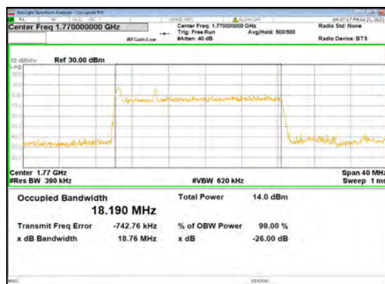
B13_N66(20M)_DFT-s-OFDM_64 QAM_Outer_Full_High_CH
