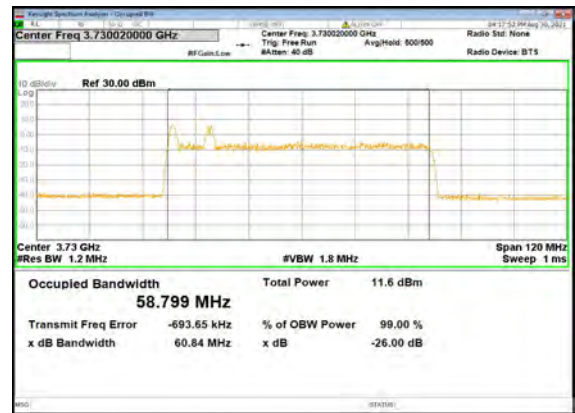
B5_N77(60M)_DFT-s-OFDM_64 QAM_Outer_Full_Low_CH
