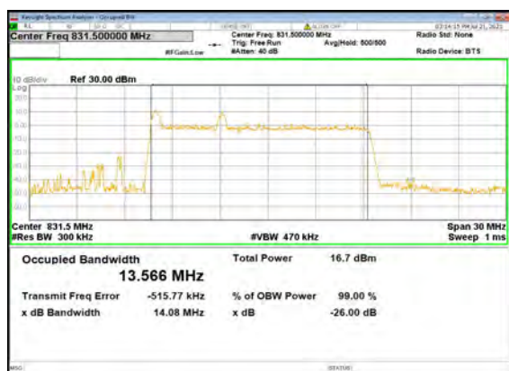
B2_N5(15M)_DFT-s-OFDM_PI_2-BPSK_Outer_Full_Low_CH
