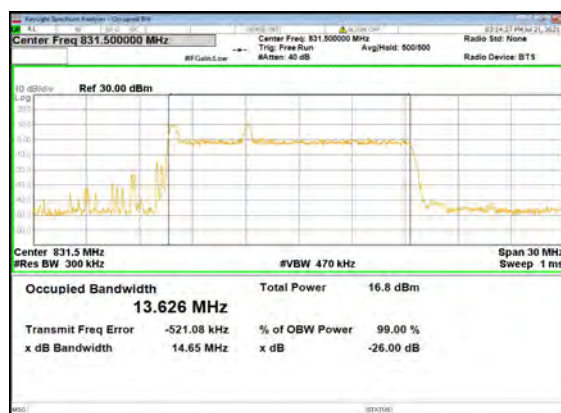
B2_N5(15M)_DFT-s-OFDM_QPSK_Outer_Full_Low_CH
