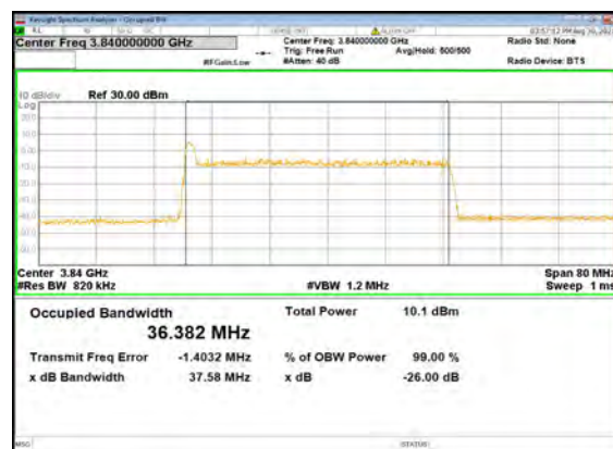
B5_N77(40M)_DFT-s-OFDM_64 QAM_Outer_Full_Mid_CH
