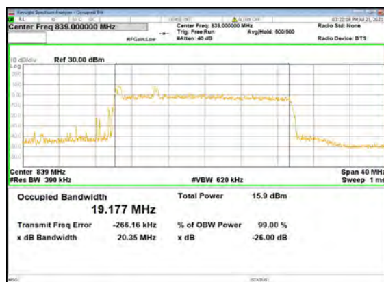
B2_N5(20M)_CP-OFDM_QPSK_Outer_Full_High_CH
