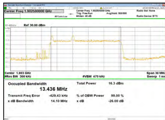
B13_N2(15M)_DFT-s-OFDM_QPSK_Outer_F ull_High_CH
