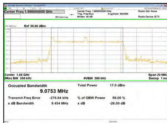
B13_N2(10M)_DFT-s-OFDM_64 QAM_Outer_Full_Mid_CH
