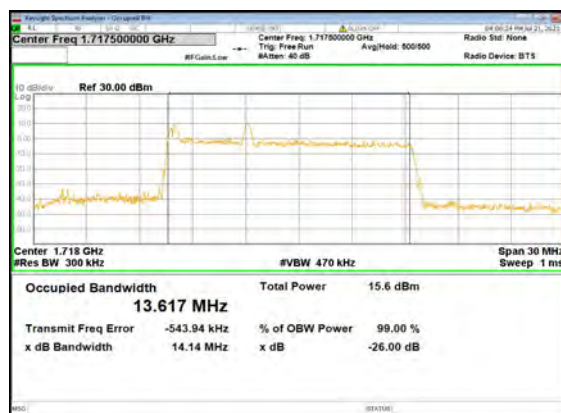
B13_N66(15M)_DFT-s-OFDM_64 QAM_Outer_Full_Low_CH
