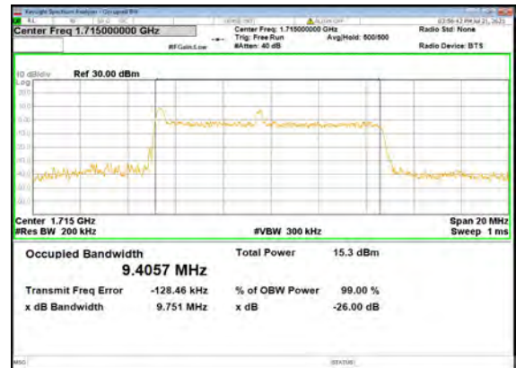
B13_N66(10M)_CP-OFDM_QPSK_Outer_Ful I_Low_CH
