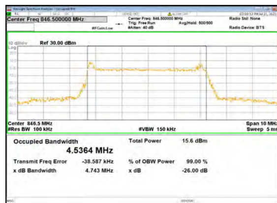
B2_N5(5M)_DFT-s-OFDM_64 QAM_Outer_Full_High_CH
