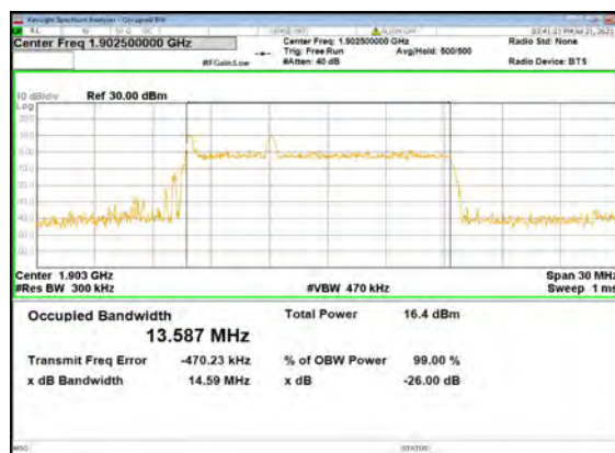
B13_N2(15M)_DFT-s-OFDM_64 QAM_Outer_Full_High_CH
