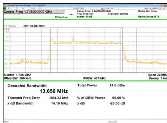
B13_N66(15M)_DFT-s-OFDM_64 QAM_Outer_Full_Mid_CH
