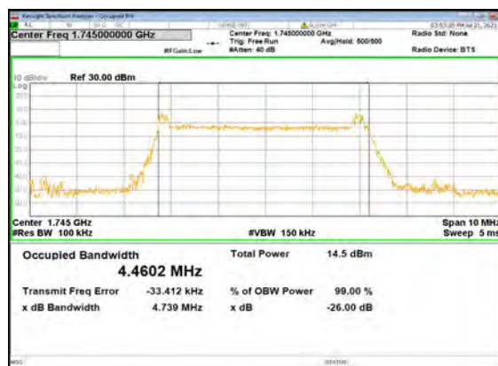
B13_N66(5M)_DFT-s-OFDM_64 QAM_Outer_Full_Mid_CH
