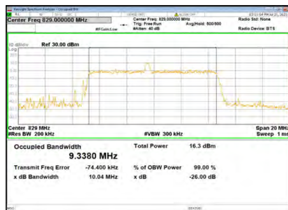
B2_N5(10M)_CP-OFDM_QPSK_Outer_Full_ Low_CH
