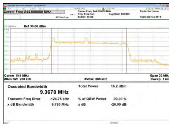
B2_N5(10M)_CP-OFDM_QPSK_Outer_Full_High_CH
