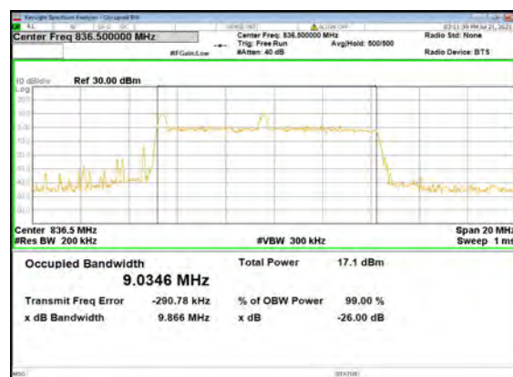
B2_N5(10M)_DFT-s-OFDM_QPSK_Outer_Fu ll_Mid_CH
