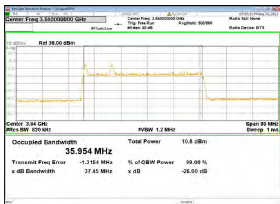
B5_N77(40M)_DFT-s-OFDM_16 QAM_Outer_Full_Mid_CH
