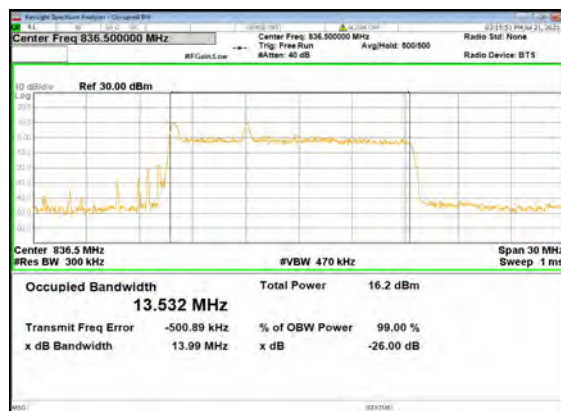
B2_N5(15M)_DFT-s-OFDM_QPSK_Outer_Fu ll_Mid_CH
