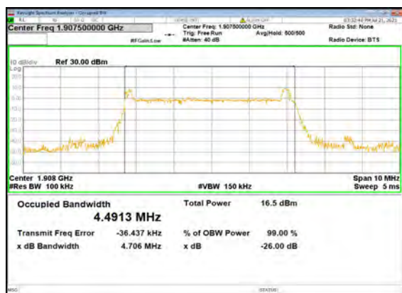
B13_N2(5M)_DFT-s-OFDM_16 QAM_Outer_Full_High_CH
