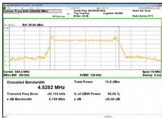
B2_N5(5M)_DFT-s-OFDM_16 QAM_Outer_Full_High_CH
