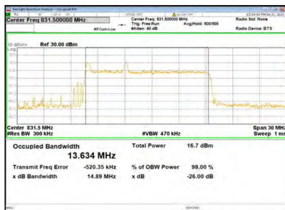
B2_N5(15M)_DFT-s-OFDM_64 QAM_Outer_Full_Low_CH
