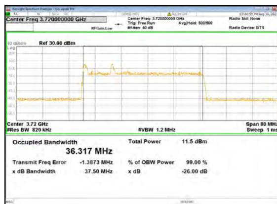
B5_N77(40M)_DFT-s-OFDM_64 QAM_Outer_Full_Low_CH
