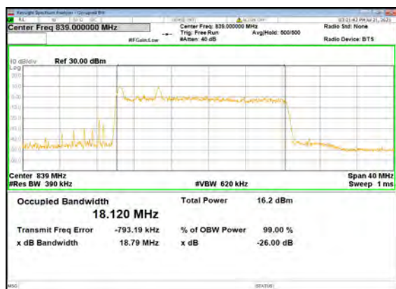
B2_N5(20M)_DFT-s-OFDM_16 QAM_Outer_Full_High_CH
