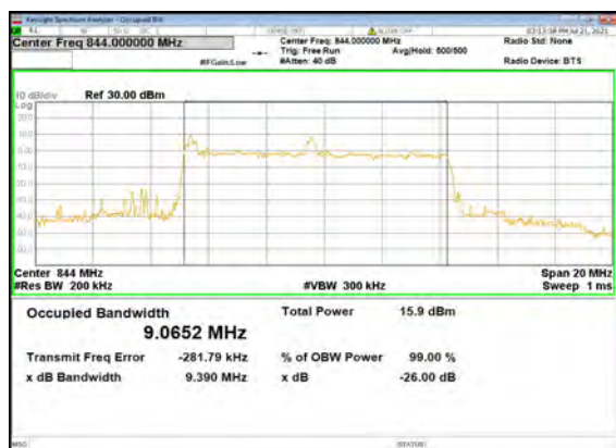
B2_N5(10M)_DFT-s-OFDM_256 QAM_Outer_Full_High_CH
