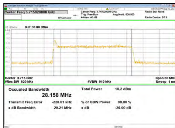
B5_N77(30M)_CP-OFDM_QPSK_Outer_Full _Low_CH
