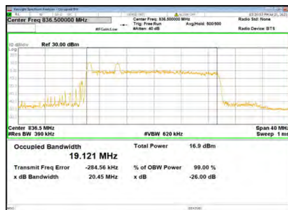
B2_N5(20M)_CP-OFDM_QPSK_Outer_Full Mid_CH
