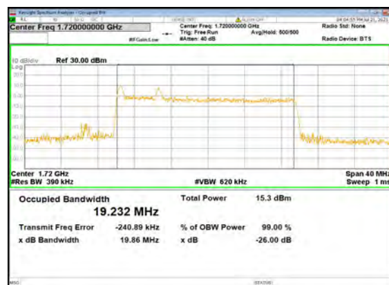
B13_N66(20M)_CP-OFDM_QPSK_Outer_Ful I_Low_CH
