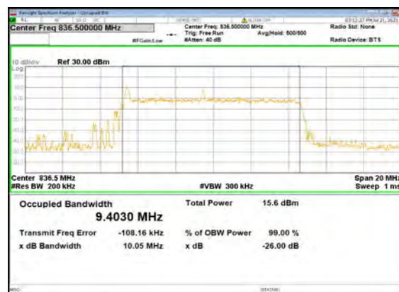
B2_N5(10M)_CP-OFDM_QPSK_Outer_Full_Mid_CH
