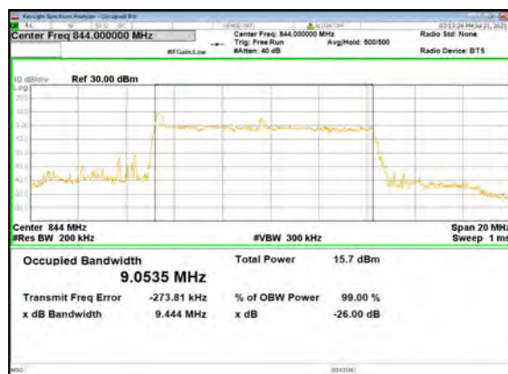
B2_N5(10M)_DFT-s-OFDM_64 QAM_Outer_Full_High_CH
