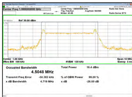
B13_N2(5M)_DFT-s-OFDM_64 QAM_Outer_Full_Mid_CH
