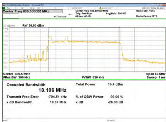
B2_N5(20M)_DFT-s-OFDM_PI_2-BPSK_Outer_F ull_Mid_CH
