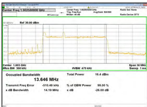
B13_N2(15M)_DFT-s-OFDM_256 QAM_Outer_Full_High_CH
