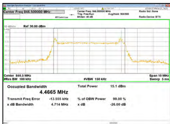
B2_N5(5M)_DFT-s-OFDM_256 QAM_Outer_Full_High_CH
