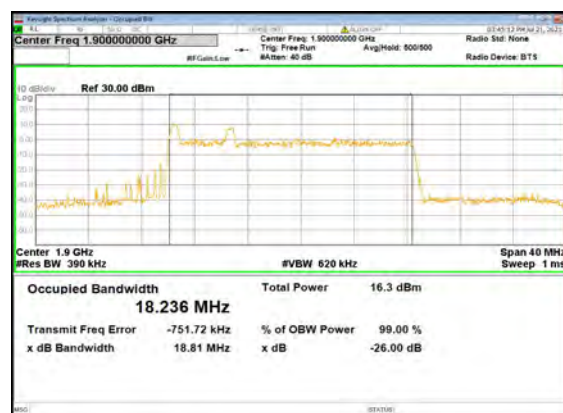
B13_N2(20M)_DFT-s-OFDM_QPSK_Outer_Full_High_CH
