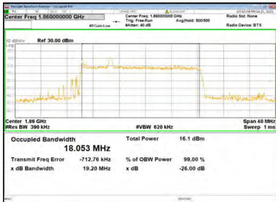
B13_N2(20M)_DFT-s-OFDM_256 QAM_Outer_Full_Low_CH
