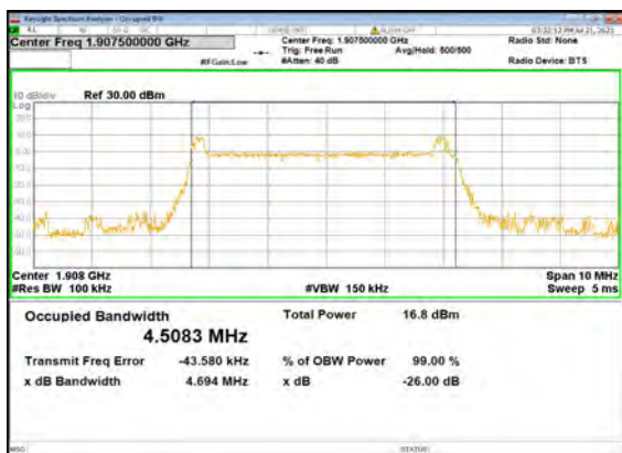
B13_N2(5M)_DFT-s-OFDM_PI_2-BPSK_Outer_F ull_High_CH
