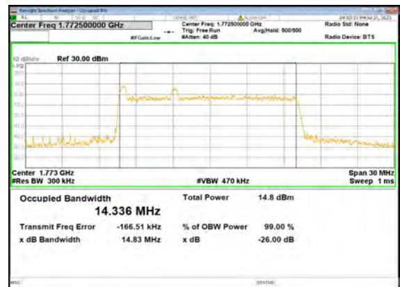
B13_N66(15M)_CP-OFDM_QPSK_Outer_Ful I_High_CH
