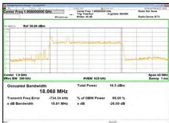
B13_N2(20M)_DFT-s-OFDM_256 QAM_Outer_Full_High_CH
