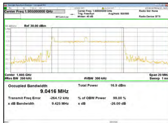
B13_N2(10M)_DFT-s-OFDM_QPSK_Outer_F ull_High_CH
