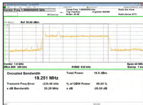
B13_N2(20M)_CP-OFDM_QPSK_Outer_Full _High_CH
