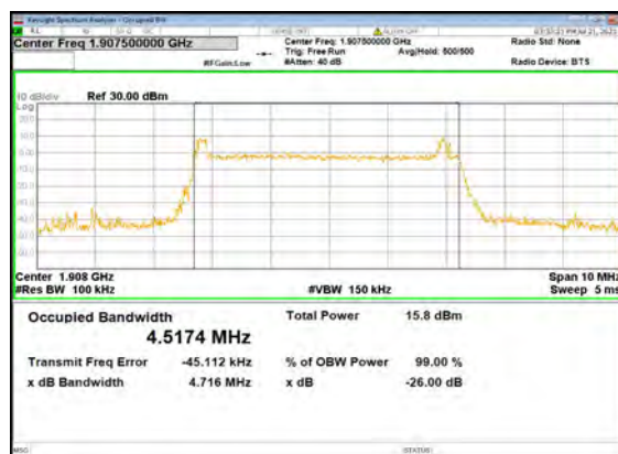
B13_N2(5M)_CP-OFDM_QPSK_Outer_Full_High_CH
