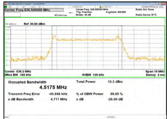
B2_N5(5M)_CP-OFDM_QPSK_Outer_Full_M id_CH
