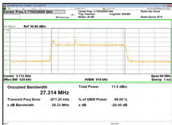
B5_N77(30M)_DFT-s-OFDM_16 QAM_Outer_Full_Low_CH
