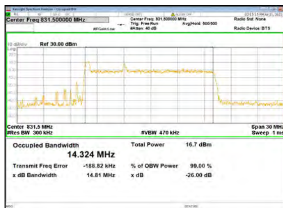
B2_N5(15M)_CP-OFDM_QPSK_Outer_Full_ Low_CH
