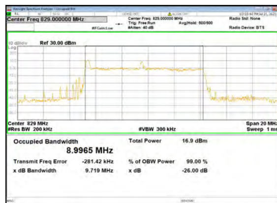
B2_N5(10M)_DFT-s-OFDM_64 QAM_Outer_Full_Low_CH
