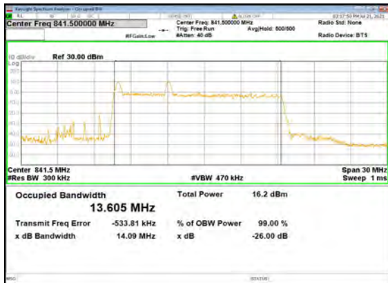
B2_N5(15M)_DFT-s-OFDM_256 QAM_Outer_Full_High_CH
