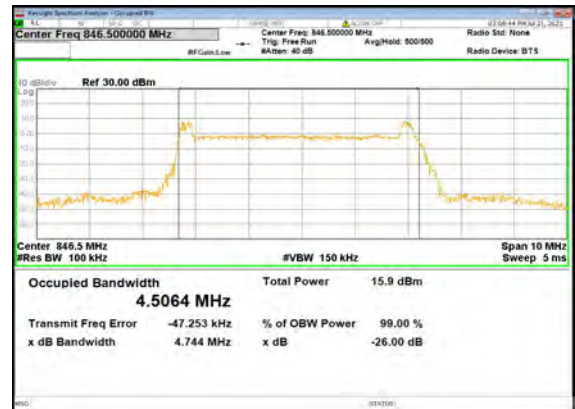
B2_N5(5M)_DFT-s-OFDM_QPSK_Outer_Full _High_CH
