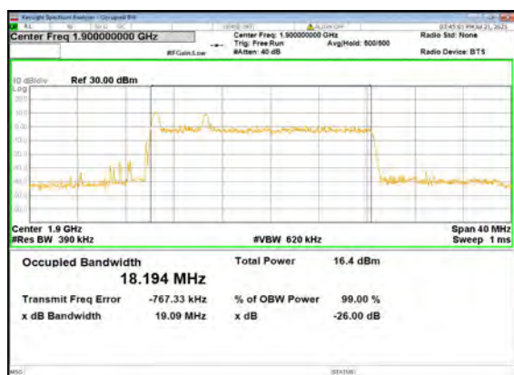
B13_N2(20M)_DFT-s-OFDM_PI_2-BPSK_Outer_Full_High_CH
