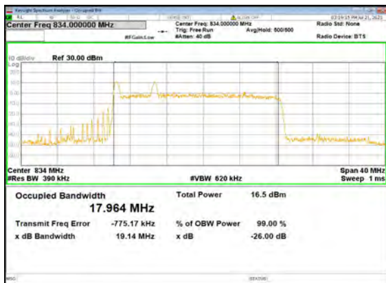
B2_N5(20M)_DFT-s-OFDM_256 QAM_Outer_Full_Low_CH
