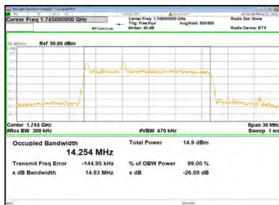
B13_N66(15M)_CP-OFDM_QPSK_Outer_Ful I_Mid_CH
