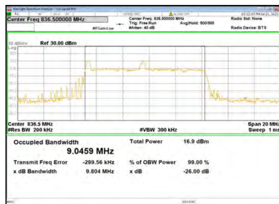
B2_N5(10M)_DFT-s-OFDM_64 QAM_Outer_Full_Mid_CH
