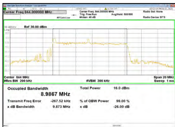
B2_N5(10M)_DFT-s-OFDM_16 QAM_Outer_Full_High_CH
