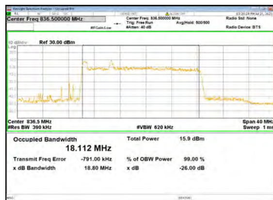
B2_N5(20M)_DFT-s-OFDM_64 QAM_Outer_Full_Mid_CH
