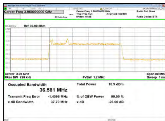
B5_N77(40M)_DFT-s-OFDM_QPSK_Outer_F ull_High_CH
