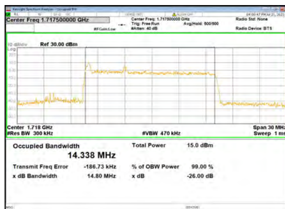
B13_N66(15M)_CP-OFDM_QPSK_Outer_Ful I_Low_CH
