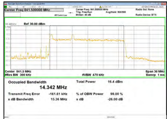
B2_N5(15M)_CP-OFDM_QPSK_Outer_Full High_CH
