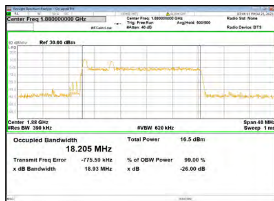
B13_N2(20M)_DFT-s-OFDM_64 QAM_Outer_Full_Mid_CH
