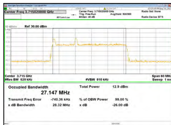
B5_N77(30M)_DFT-s-OFDM_64 QAM_Outer_Full_Low_CH
