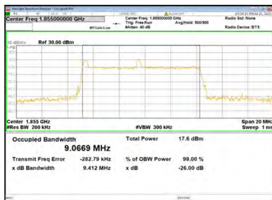
B13_N2(10M)_DFT-s-OFDM_64 QAM_Outer_Full_Low_CH
