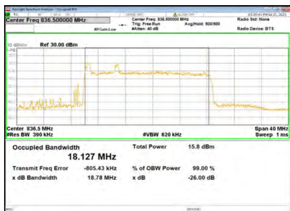
B2_N5(20M)_DFT-s-OFDM_256 QAM_Outer_Full_Mid_CH
