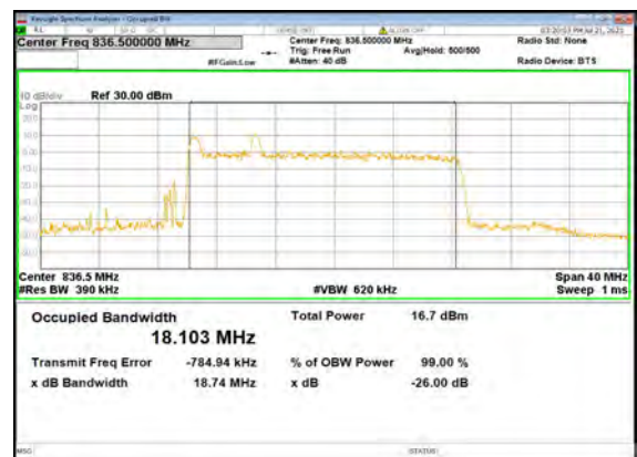
B2_N5(20M)_DFT-s-OFDM_QPSK_Outer_Fu ll_Mid_CH
