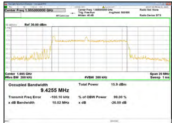
B13_N2(10M)_CP-OFDM_QPSK_Outer_Full _High_CH
