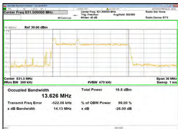
B2_N5(15M)_DFT-s-OFDM_256 QAM_Outer_Full_Low_CH
