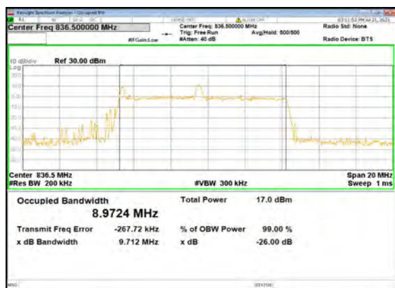
B2_N5(10M)_DFT-s-OFDM_16 QAM_Outer_Full_Mid_CH
