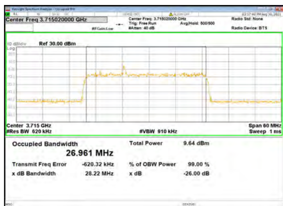
B5_N77(30M)_DFT-s-OFDM_256 QAM_Outer_Full_Low_CH
