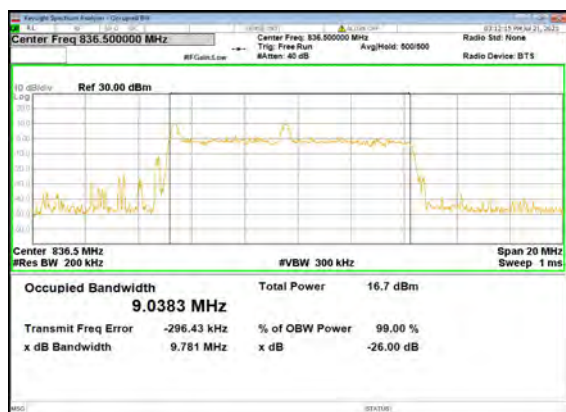
B2_N5(10M)_DFT-s-OFDM_256 QAM_Outer_Full_Mid_CH
