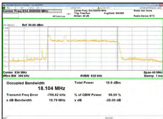
B2_N5(20M)_DFT-s-OFDM_PI_2-BPSK_Outer_F ull_Low_CH
