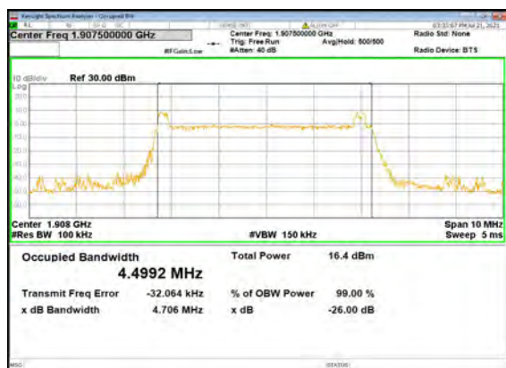
B13_N2(5M)_DFT-s-OFDM_256 QAM_Outer_Full_High_CH
