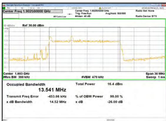
B13_N2(15M)_DFT-s-OFDM_PI_2-BPSK_Outer_ Full_High_CH
