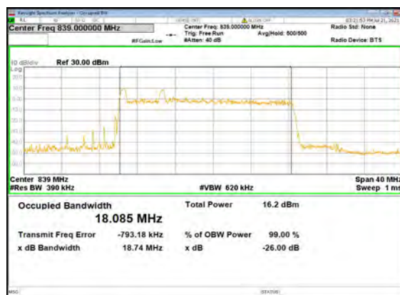
B2_N5(20M)_DFT-s-OFDM_64 QAM_Outer_Full_High_CH
