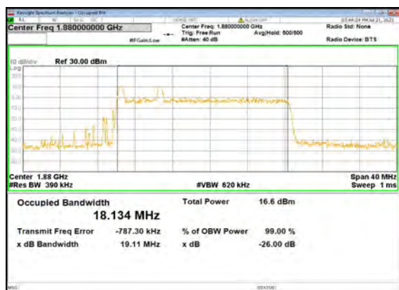
B13_N2(20M)_DFT-s-OFDM_256 QAM_Outer_Full_Mid_CH
