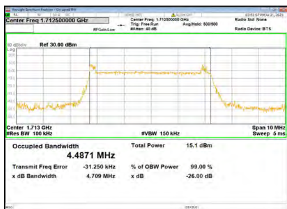
B13_N66(5M)_DFT-s-OFDM_PI_2-BPSK_Outer_Full_Low_CH
