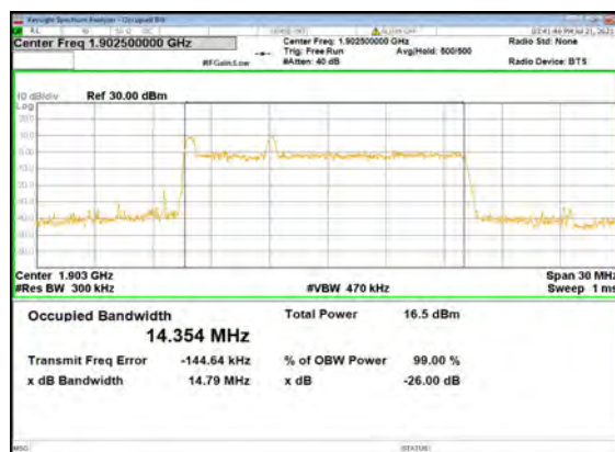
B13_N2(15M)_CP-OFDM_QPSK_Outer_Full _High_CH
