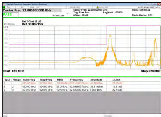
B2_N5(5M)_DFT-s-OFDM_BPSK_Edge_1RB_ Left_Low_CH
