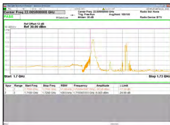
B13_N66(5M)_DFT-s-OFDM_QPSK_Edge_1R B_Left_Low_CH
