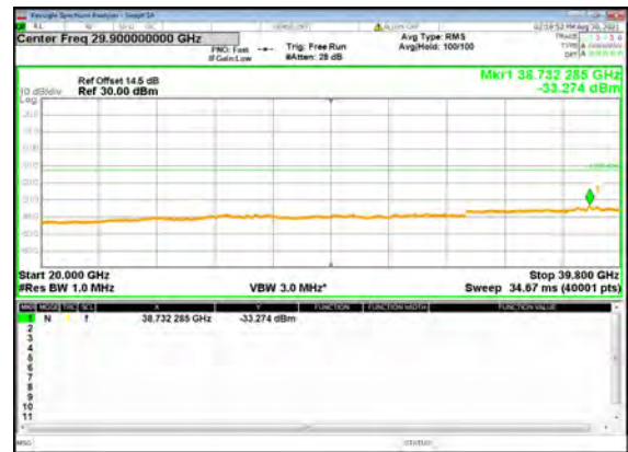
B5_N77(30M)_DFT-s-OFDM_BPSK_Edge_1R B_Left_Low_CH
