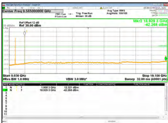
B13_N2(10M)_DFT-s-OFDM_BPSK_Edge_1R B_Left_High_CH
