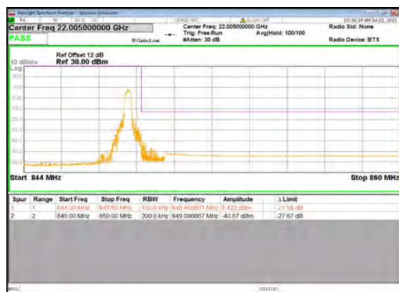
B2_N5(20M)_DFT-s-OFDM_QPSK_Edge_1RB _Right_High_CH
