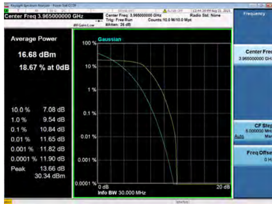
B5_N77(30M)_DFT-s-OFDM_PI_2-BPSK_Outer_Full_High_CH
