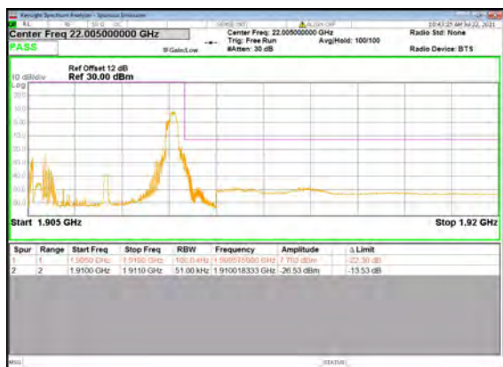
B13_N2(5M)_DFT-s-OFDM_BPSK_Edge_1RB _Right_High_CH
