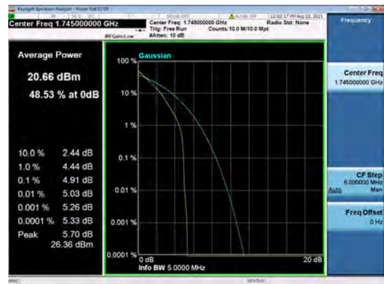
B13_N66(5M)_DFT-s-OFDM_QPSK_Outer_Full_Mid_CH
