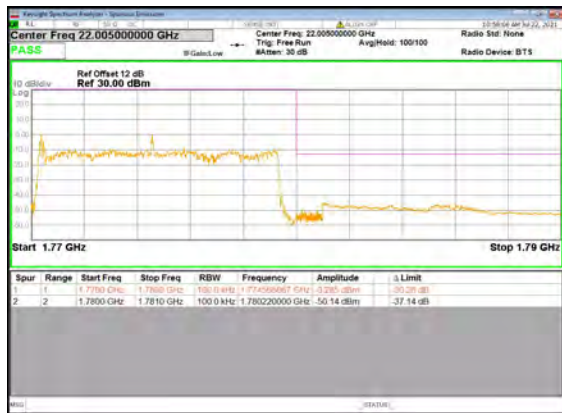
B13_N66(10M)_DFT-s-OFDM_BPSK_Outer_F ull_High_CH
