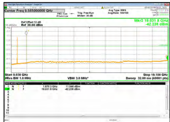
B13_N2(20M)_DFT-s-OFDM_QPSK_Edge_1R B_Left_Mid_CH
