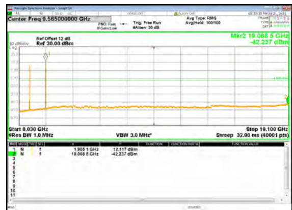
B13_N2(5M)_DFT-s-OFDM_QPSK_Edge_1RB _Left_High_CH
