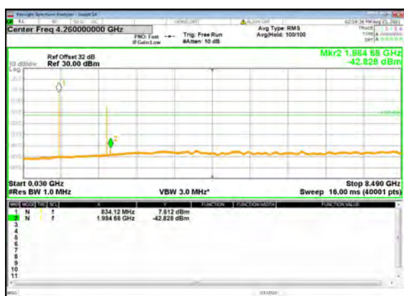
B2_N5(5M)_DFT-s-OFDM_BPSK_Edge_1RB_ Left_Mid_CH
