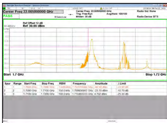
B13_N66(15M)_DFT-s-OFDM_BPSK_Edge_1 RB_Left_Low_CH
