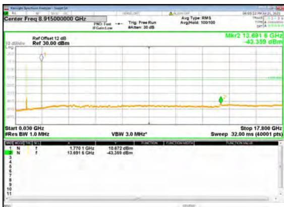
B13_N66(10M)_DFT-s-OFDM_BPSK_Edge_1 RB_Left_High_CH
