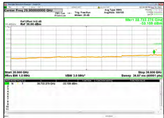
B5_N77(30M)_DFT-s-OFDM_BPSK_Edge_1R B_Left_High_CH
