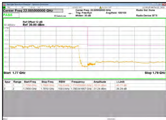
B13_N66(15M)_DFT-s-OFDM_BPSK_Outer_F ull_High_CH
