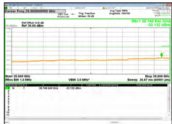
B5_N77(100M)_DFT-s-OFDM_QPSK_Edge_1 RB_Left_High_CH
