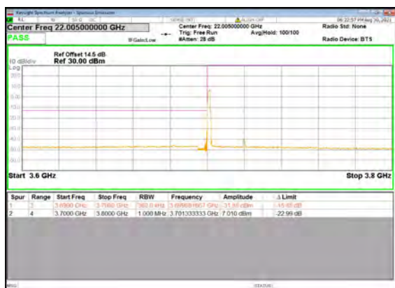
B5_N77(40M)_DFT-s-OFDM_BPSK_Edge_1R B_Left_Low_CH
