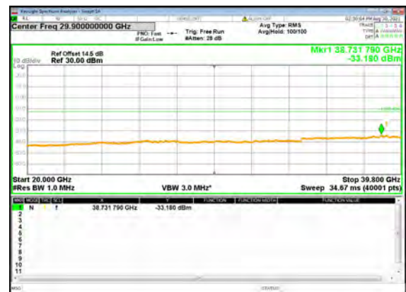
B5_N77(40M)_DFT-s-OFDM_BPSK_Edge_1R B_Left_Mid_CH
