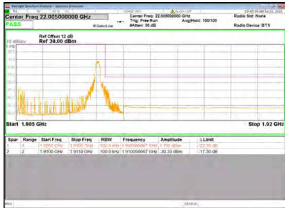
B13_N2(10M)_DFT-s-OFDM_BPSK_Edge_1R B_Right_High_CH
