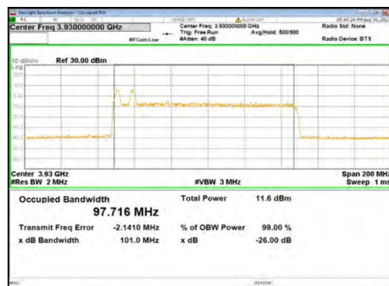
B5_N77(100M)_DFT-s-OFDM_64 QAM_Outer_Full_High_CH
