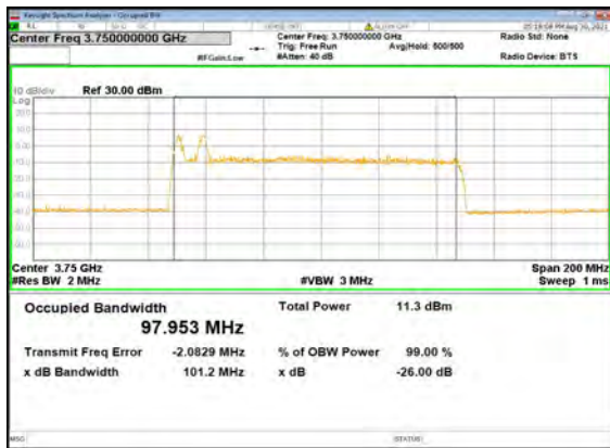
B5_N77(100M)_DFT-s-OFDM_16 QAM_Outer_Full_Low_CH
