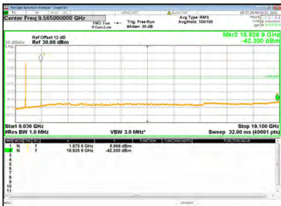
B13_N2(10M)_DFT-s-OFDM_BPSK_Edge_1R B_Left_Mid_CH
