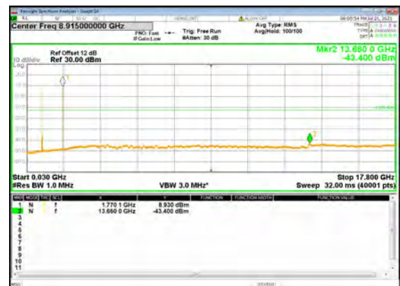
B13_N66(10M)_DFT-s-OFDM_QPSK_Edge_1 RB_Left_High_CH
