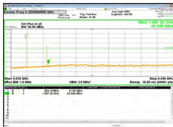
B2_N5(5M)_DFT-s-OFDM_QPSK_Edge_1RB_ Left_Low_CH
