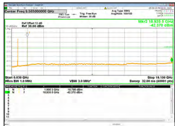
B13_N2(10M)_DFT-s-OFDM_QPSK_Edge_1R B_Left_High_CH
