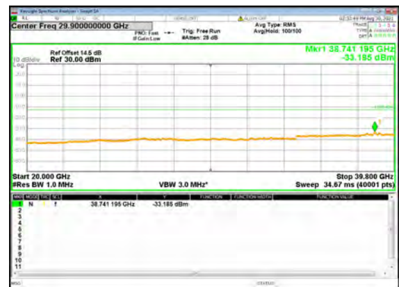
B5_N77(40M)_DFT-s-OFDM_QPSK_Edge_1R B_Left_High_CH
