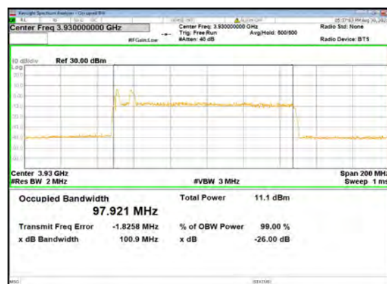
B5_N77(100M)_DFT-s-OFDM_QPSK_Outer_ Full_High_CH
