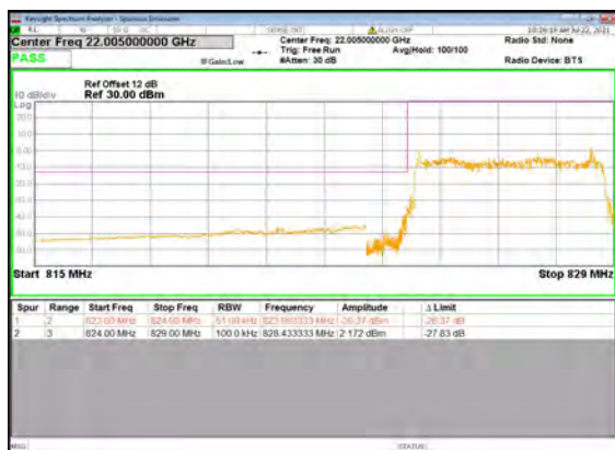
B2_N5(5M)_DFT-s-OFDM_BPSK_Outer_Full_ Low_CH
