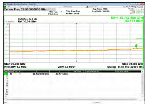
B5_N77(80M)_DFT-s-OFDM_BPSK_Edge_1R B_Left_Mid_CH
