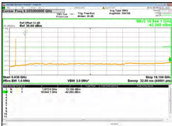
B13_N2(15M)_DFT-s-OFDM_BPSK_Edge_1R B_Left_Mid_CH
