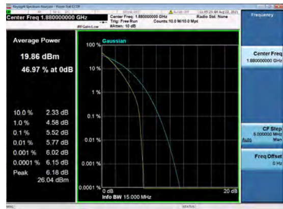
B13_N2(15M)_DFT-s-OFDM_QPSK_Outer_Full_Mid_CH
