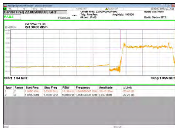
B13_N2(5M)_DFT-s-OFDM_QPSK_Outer_Full _Low_CH
