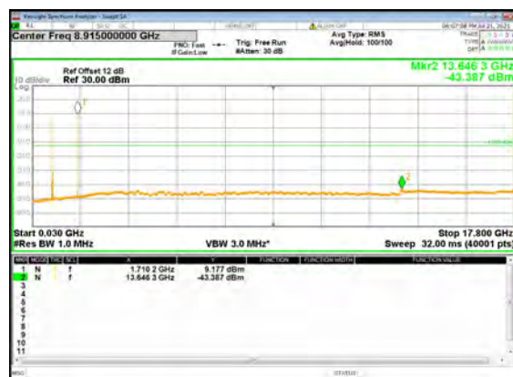
B13_N66(15M)_DFT-s-OFDM_QPSK_Edge_1 RB_Left_Low_CH
