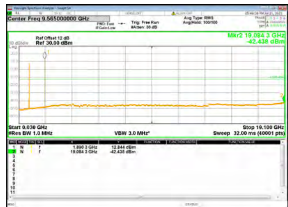
B13_N2(20M)_DFT-s-OFDM_QPSK_Edge_1R B_Left_High_CH
