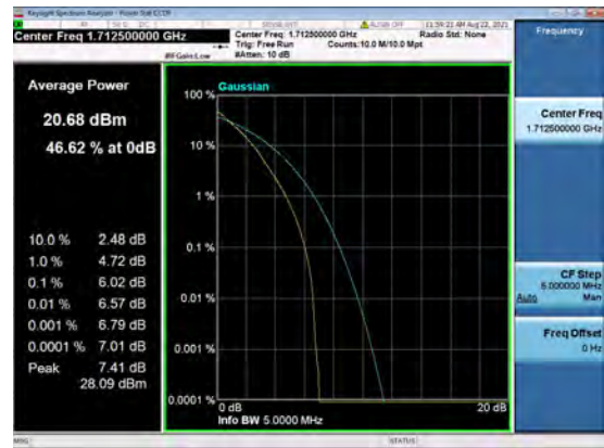
B13_N66(5M)_DFT-s-OFDM_QPSK_Outer_Full_Low_CH
