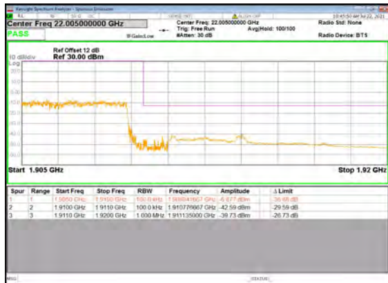
B13_N2(10M)_DFT-s-OFDM_BPSK_Outer_Ful I_High_CH
