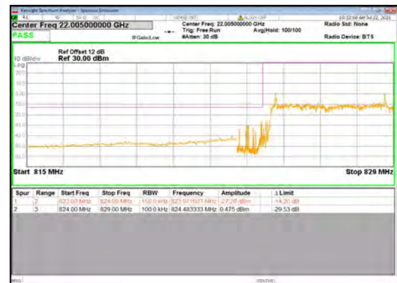
B2_N5(15M)_DFT-s-OFDM_QPSK_Outer_Full _Low_CH
