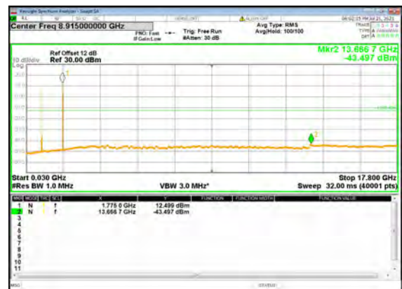
B13_N66(5M)_DFT-s-OFDM_QPSK_Edge_1R B_Left_High_CH
