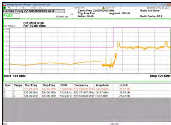
B2_N5(15M)_DFT-s-OFDM_BPSK_Outer_Full _Low_CH
