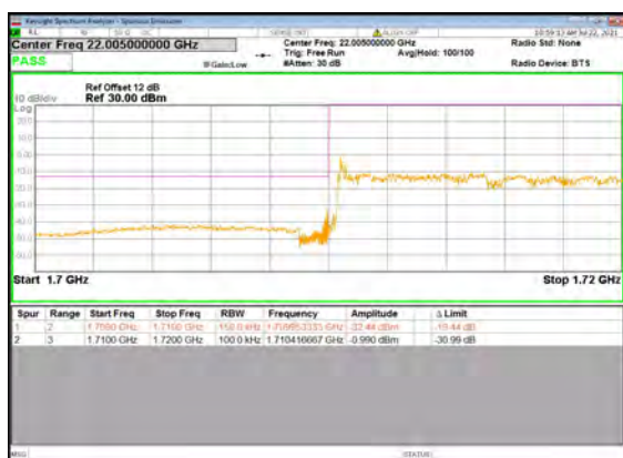
B13_N66(15M)_DFT-s-OFDM_BPSK_Outer_F ull_Low_CH
