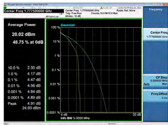
B13_N66(5M)_DFT-s-OFDM_QPSK_Outer_Full_High_CH
