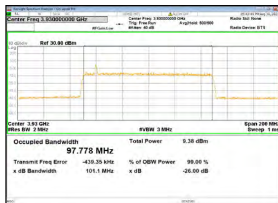
B5_N77(100M)_CP-OFDM_QPSK_Outer_Ful I_High_CH
