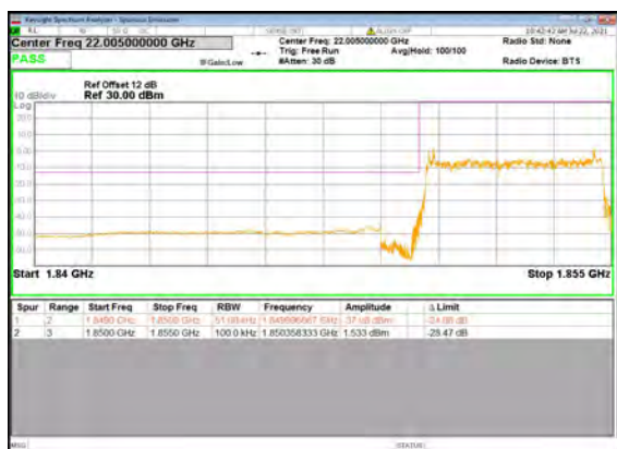
B13_N2(5M)_DFT-s-OFDM_BPSK_Outer_Full _Low_CH
