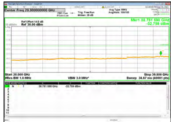
B5_N77(80M)_DFT-s-OFDM_BPSK_Edge_1R B_Left_High_CH
