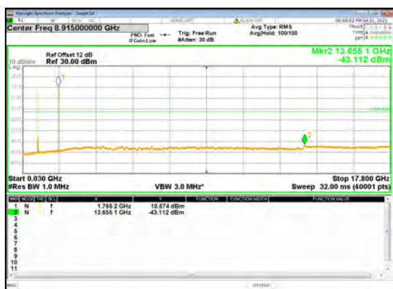
B13_N66(15M)_DFT-s-OFDM_BPSK_Edge_1 RB_Left_High_CH
