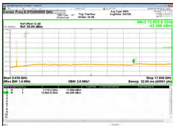
B13_N66(15M)_DFT-s-OFDM_BPSK_Edge_1 RB_Left_Low_CH
