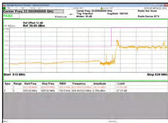
B2_N5(20M)_DFT-s-OFDM_BPSK_Outer_Full_Low_CH
