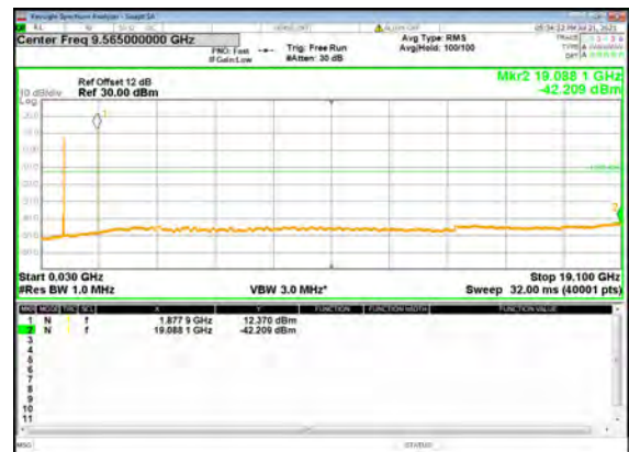
B13_N2(5M)_DFT-s-OFDM_QPSK_Edge_1RB _Left_Mid_CH
