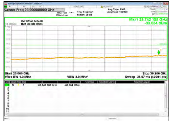
B5_N77(80M)_DFT-s-OFDM_BPSK_Edge_1R B_Left_Low_CH
