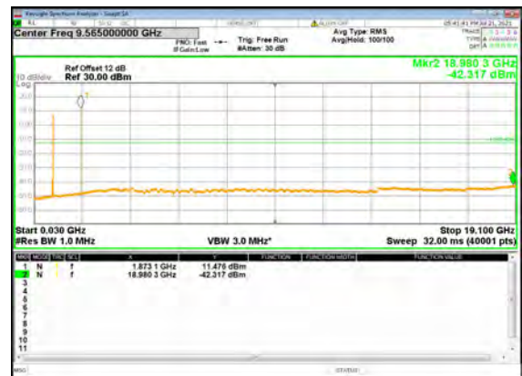
B13_N2(15M)_DFT-s-OFDM_QPSK_Edge_1R B_Left_Mid_CH
