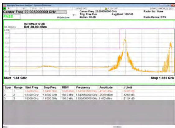
B13_N2(15M)_DFT-s-OFDM_BPSK_Edge_1R B_Left_Low_CH
