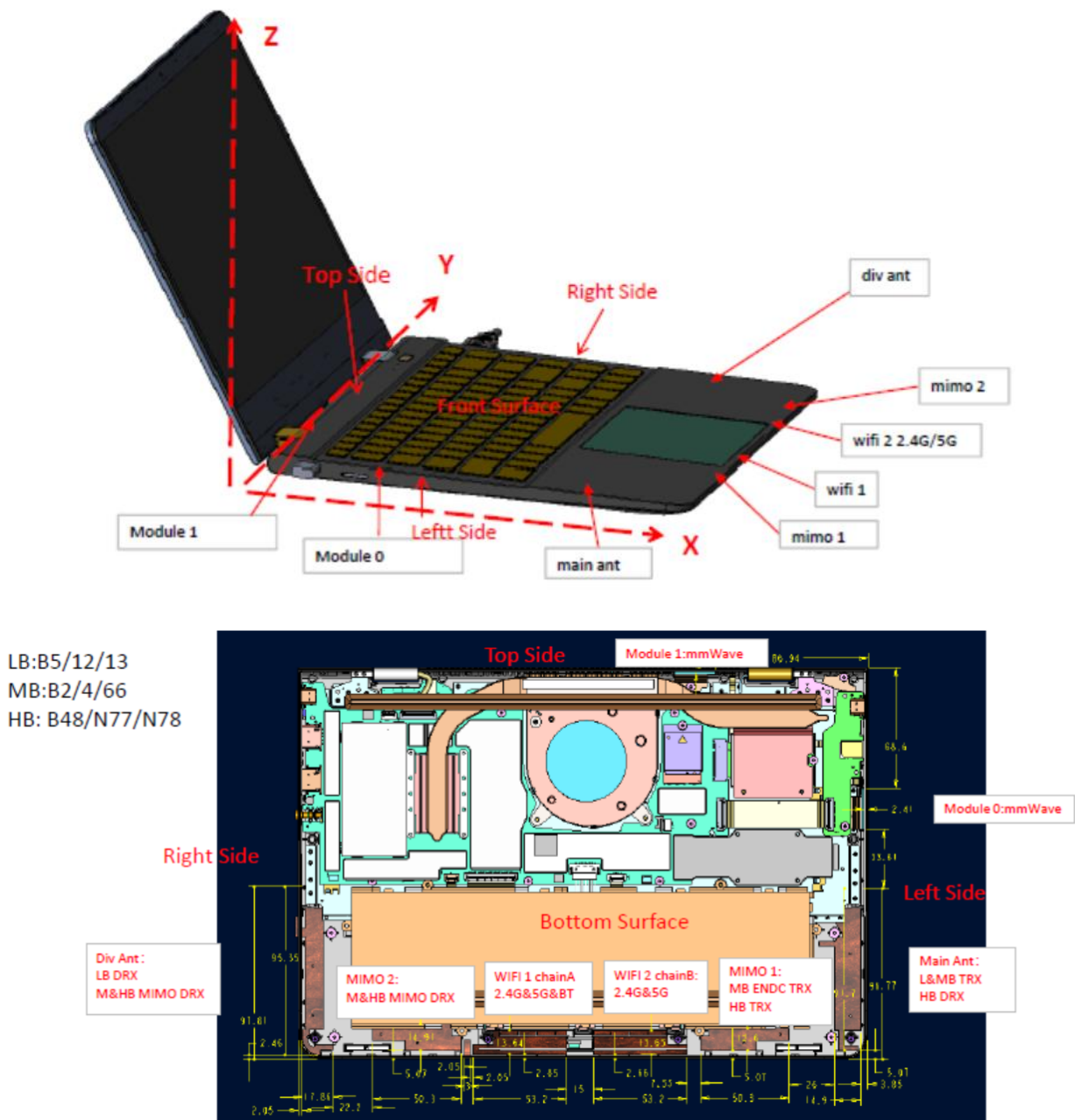
Fig.15.1 EUT Antenna Locations
