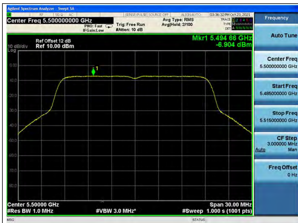
(Channel 100, 5500MHz, 802.11ax (HEW20), ANT1)
