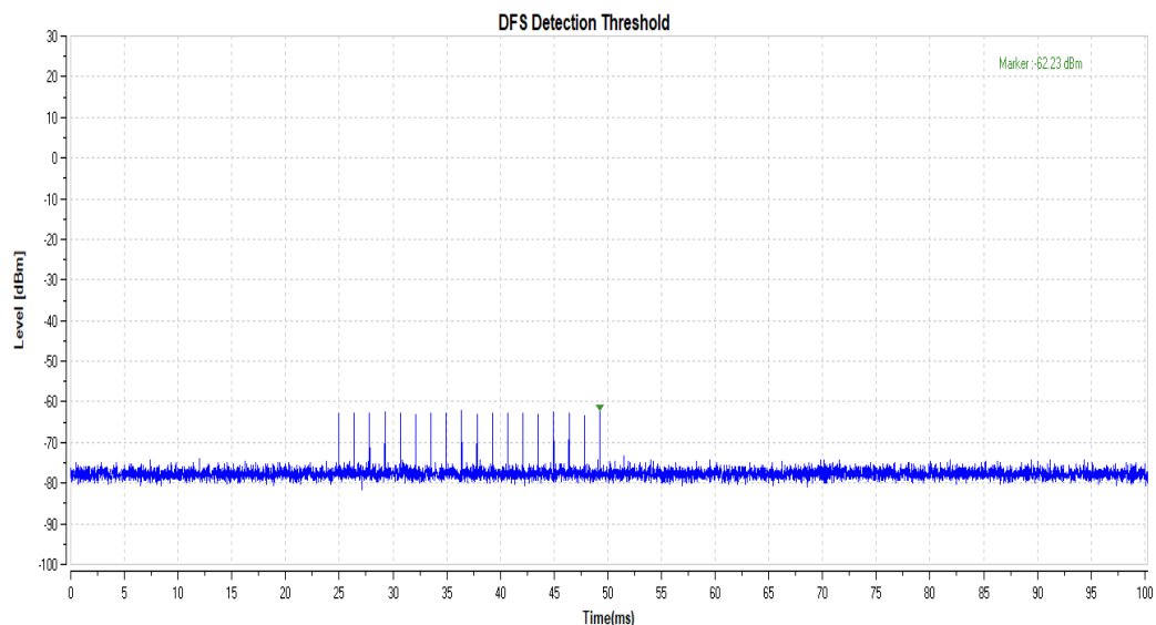
11AC20SISO_5500_Reference
