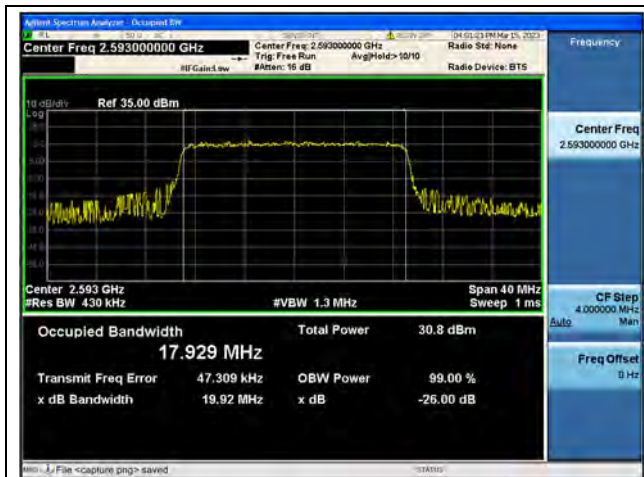
Band41 / 20MHz / QPSK/ Mid CH
