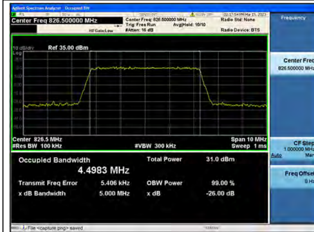
Band26 Part22 / 5MHz / 64QAM/ Low CH
