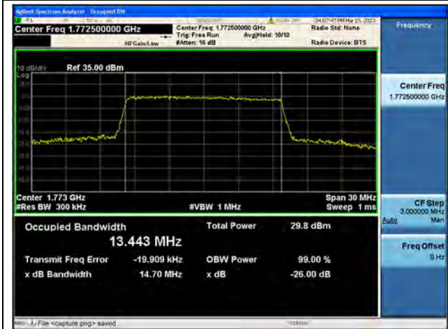
Band66 / 15MHz / 64QAM/ High CH
