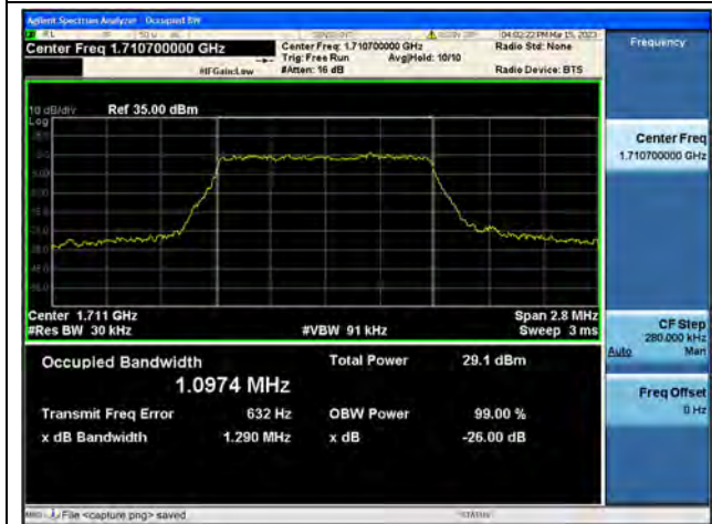
Band66 / 1.4MHz / 64QAM/ Low CH
