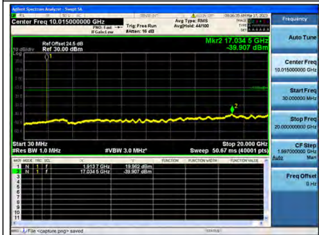
Band25 / 1.4MHz / High CH / 64QAM
