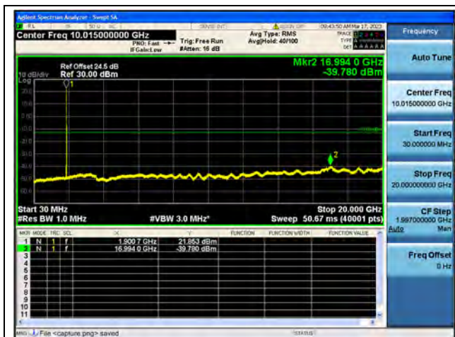
Band25 / 15MHz / High CH / QPSK
