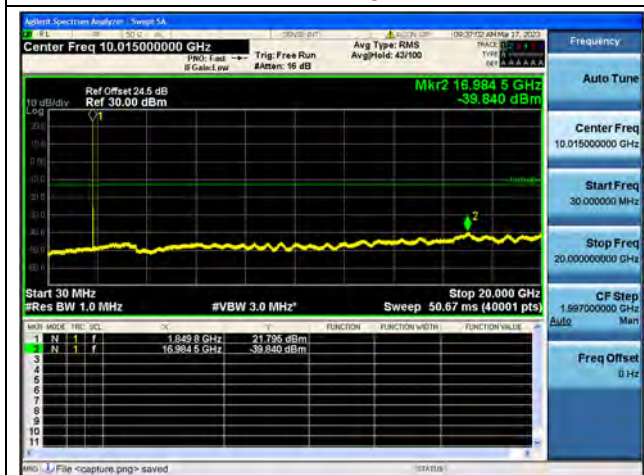
Band25 / 3MHz / Low CH / 16QAM
