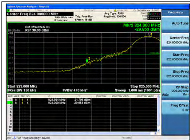
Band26 Part22 / 15MHz / Low CH / QPSK / 1 RB
