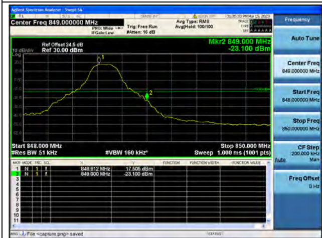
Band26 Part22 / 5MHz / High CH / QPSK / 1 RB
