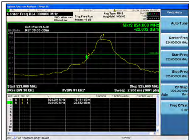
Band26 Part22 / 3MHz / Low CH / QPSK / 1 RB
