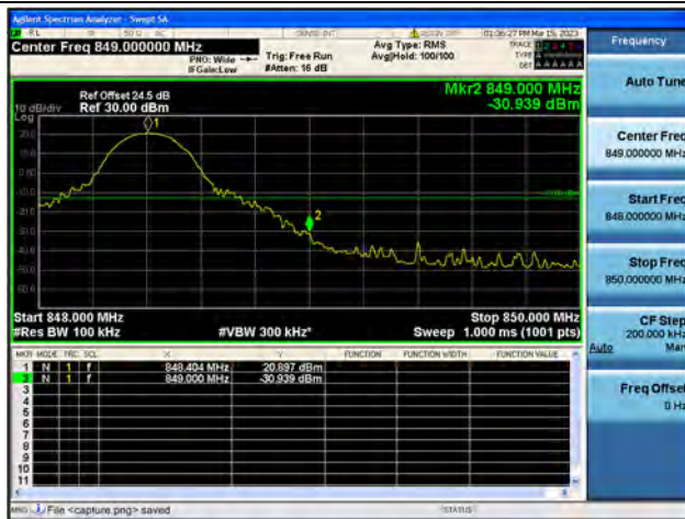
Band26 Part22 / 10MHz / High CH / QPSK / 1 RB
