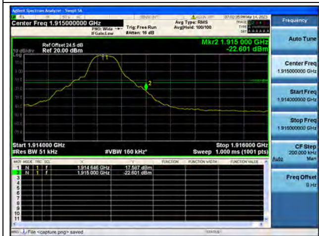
Band25 / 5MHz / High CH / QPSK / 1 RB
