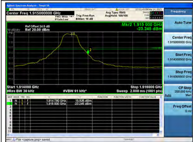
Band25 / 3MHz / High CH / QPSK / 1 RB
