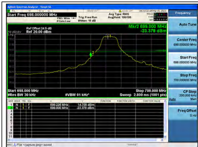
Band12 / 1.4MHz / Low CH / QPSK / 1 RB
