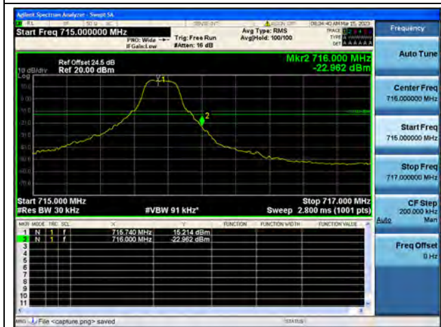
Band12 / 3MHz / High CH / QPSK / 1 RB
