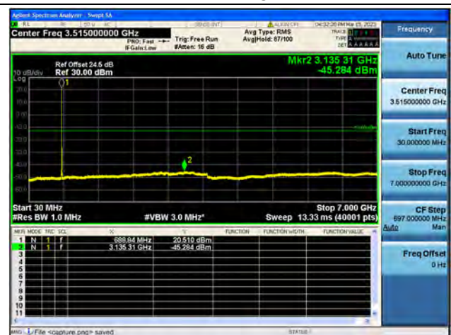
Band71 / 10MHz / High CH / 64QAM
