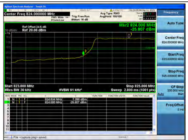
Band5 / 1.4MHz / Low CH / QPSK / FULL RB
