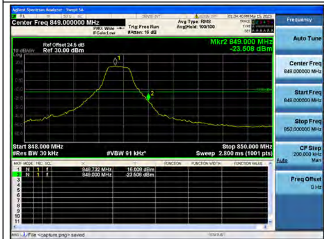
Band26 Part22 / 3MHz / High CH / QPSK / 1 RB
