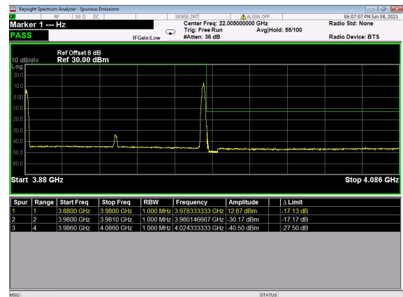
B2_N77(100M)_DFT-s-OFDM_QPSK_Edge_1 RB_Right_High_CH
