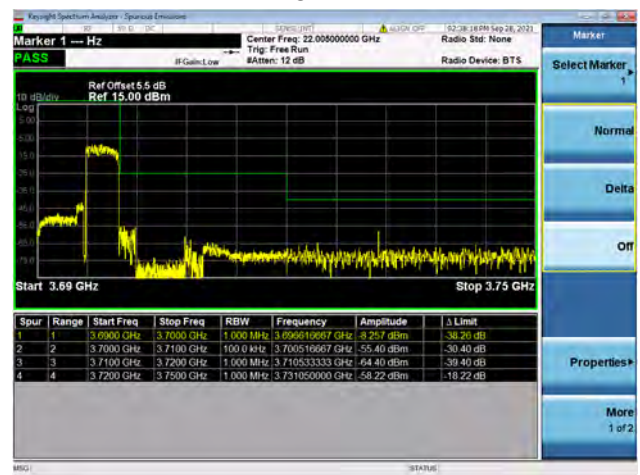
Band48 / 10MHz / High CH / QPSK / FULL RB
