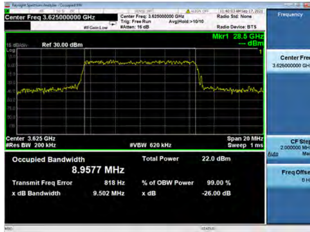
Band48 / 10MHz / Mid CH / 64QAM
