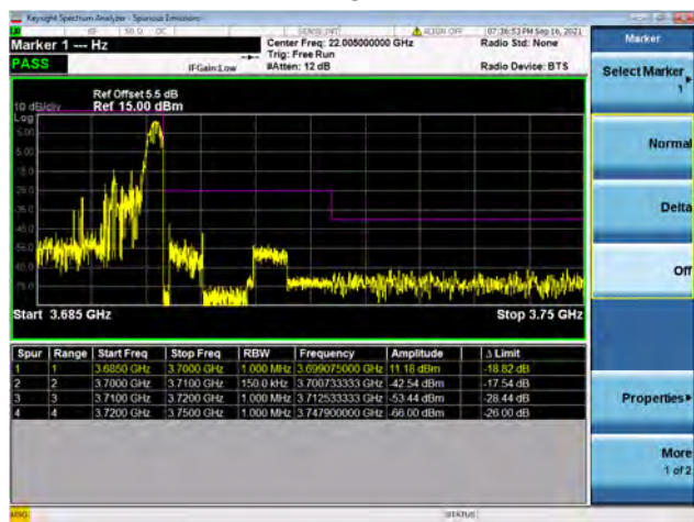
Band48 / 15MHz / High CH / QPSK / 1 RB
