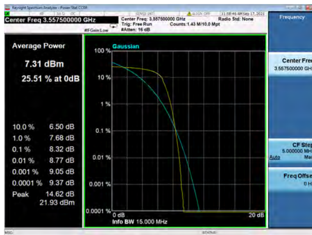
Band48 / 15MHz / Low CH / 64QAM
