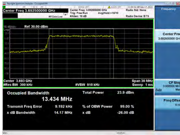
Band48 / 15MHz / High CH / 64QAM
