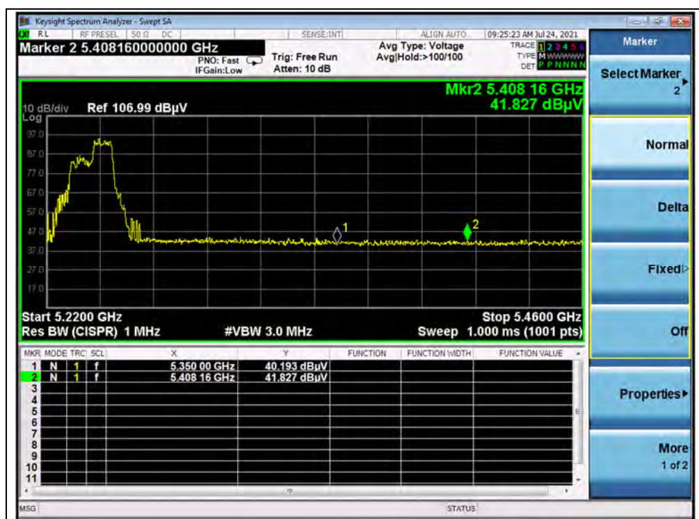
(PEAK, Channel 48, 802.11ax (HEW20) RU106)
