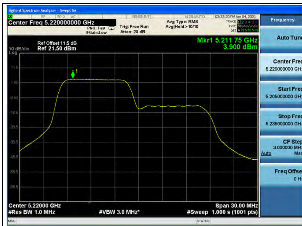
(Channel 44, 5220MHz, 802.11ax (HEW20) RU106, ANT0)
