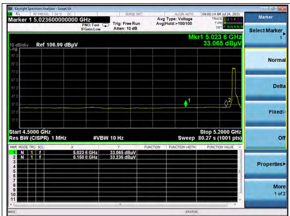
(AVERAGE, Channel 36, 802.11ax (HEW20) RU106)
