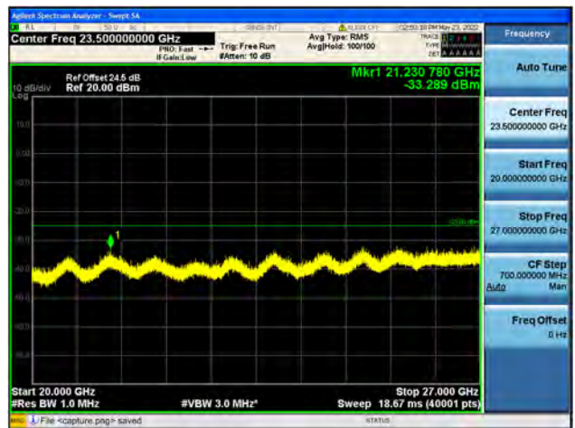
Band41-20G-27G / 10MHz / High CH / 64QAM
