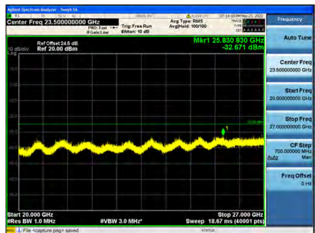
Band41-20G-27G / 15MHz / Low CH / 64QAM
