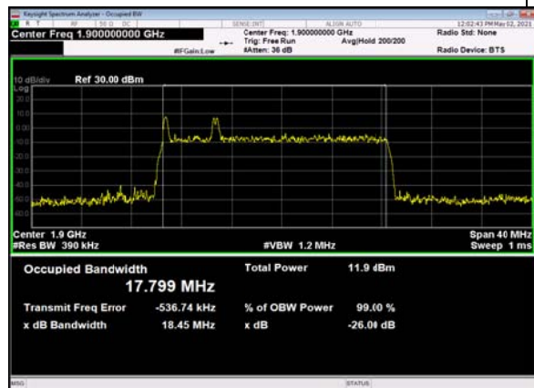
B66_n2(20M)_DFT-s-OFDM_256 QAM_Outer_Full_High_CH
