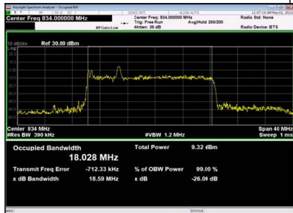
B66_n5(20M)_DFT-s-OFDM_16 QAM_Outer_Full_Low_CH
