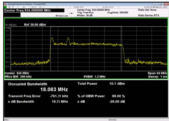
B66_n5(20M)_DFT-s-OFDM_64 QAM_Outer_Full_Low_CH
