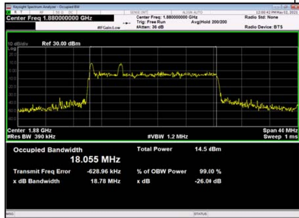
B66_n2(20M)_DFT-s-OFDM_PI_2-BPSK_ Outer_Full_Mid_CH
