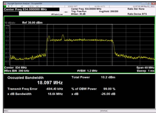
B66_n5(20M)_DFT-s-OFDM_QPSK_ Outer_Full_Low_CH
