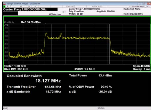
B66_n2(20M)_DFT-s-OFDM_16 QAM_Outer_Full_Mid_CH
