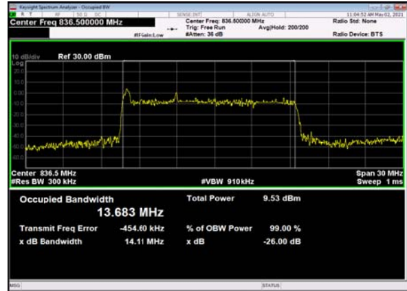
B66_n5(15M)_DFT-s-OFDM_QPSK_ Outer_Full_Mid_CH
