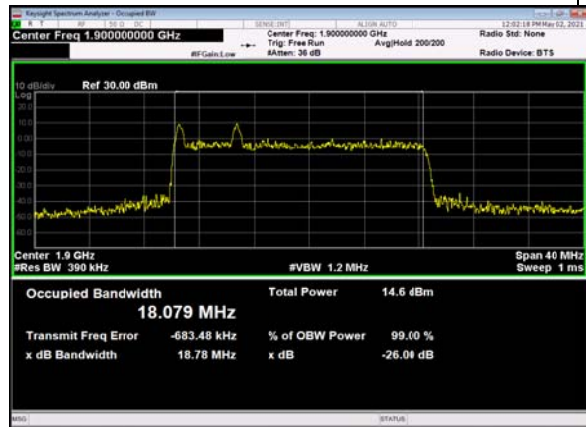
B66_n2(20M)_DFT-s-OFDM_PI_2-BPSK_ Outer_Full_High_CH
