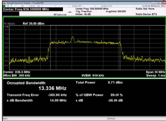
B66_n5(15M)_DFT-s-OFDM_PI_2-BPSK_ Outer_Full_Mid_CH
