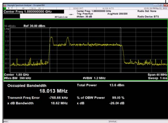
B66_n2(20M)_DFT-s-OFDM_256 QAM_Outer_Full_Mid_CH
