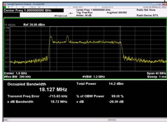
B66_n2(20M)_DFT-s-OFDM_16 QAM_Outer_Full_High_CH
