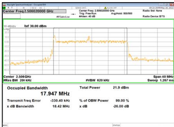
B66_n41(20M)_DFT-s-OFDM_PI_2-BPSK_Oute r_Full_Low_CH
