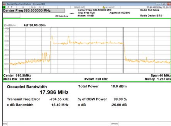
B66_n71(20M)_DFT-s-OFDM_256 QAM_Outer_Full_Mid_CH
