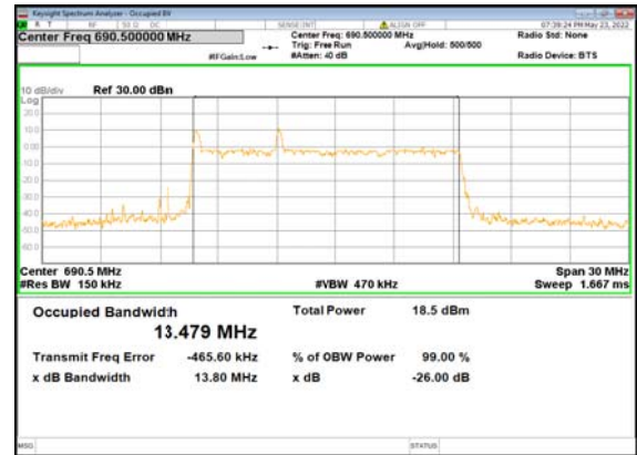
B66_n71(15M)_DFT-s-OFDM_64 QAM_Outer_Full_High_CH
