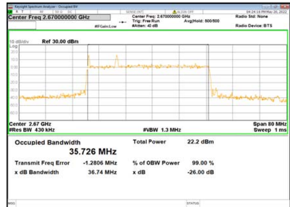
B66_n41(40M)_DFT-s-OFDM_QPSK_Outer _Full_High_CH
