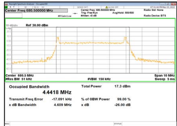
B66_n71(5M)_CP-OFDM_QPSK_Outer_Full _Mid_CH
