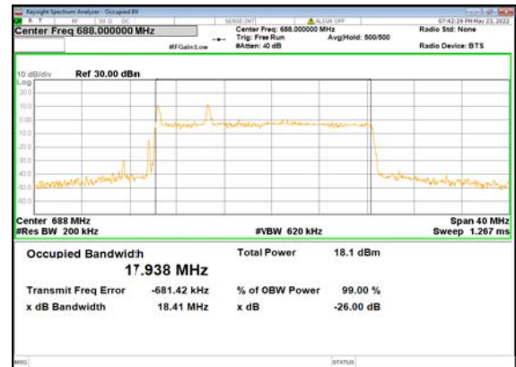
B66_n71(20M)_DFT-s-OFDM_QPSK_Outer _Full_High_CH
