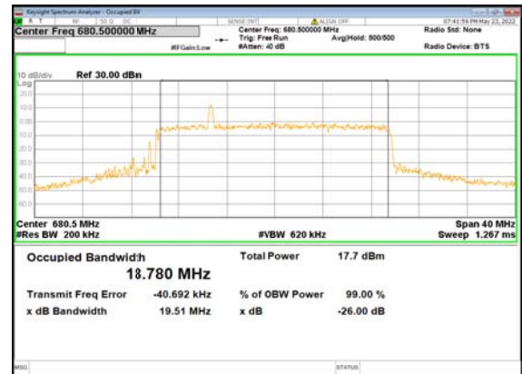
B66_n71(20M)_CP-OFDM_QPSK_Outer_Fu ll_Mid_CH
