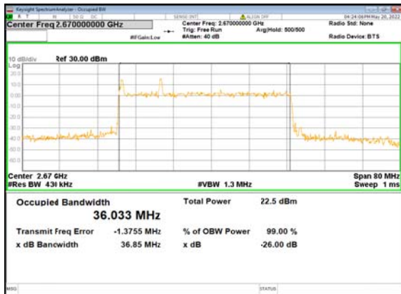
B66_n41(40M)_DFT-s-OFDM_PI_2-BPSK_Oute r_Full_High_CH
