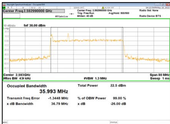
B66_n41(40M)_DFT-s-OFDM_PI_2-BPSK_Oute r_Full_Mid_CH
