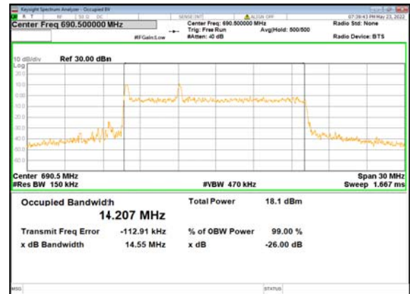
B66_n71(15M)_CP-OFDM_QPSK_Outer_Fu ll_High_CH
