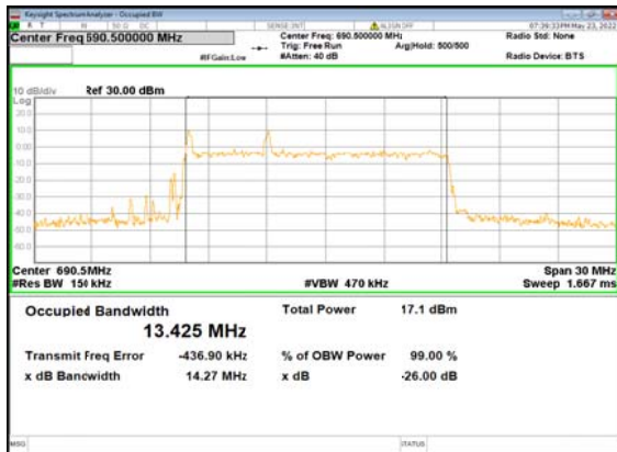
B66_n71(15M)_DFT-s-OFDM_256 QAM_Outer_Full_High_CH
