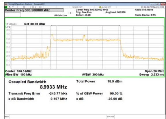
B66_n71(10M)_DFT-s-OFDM_64 QAM_Outer_Full_Mid_CH
