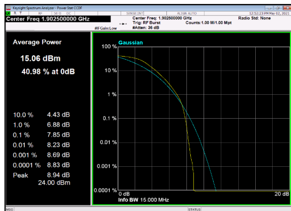
B66_n2(15M)_DFT-s-OFDM_PI_2-BPSK_Ou ter_Full_High_CH
