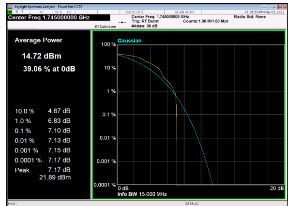
B13_n66(15M)_DFT-s-OFDM_PI_2-BPSK_Edge _1RB_Left_Mid_CH
