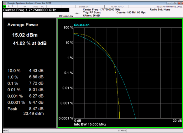
B13_n66(15M)_DFT-s-OFDM_PI_2-BPSK_O uter_Full_Low_CH
