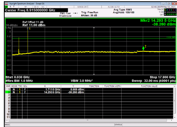
B13_n66(15M)_DFT-s-OFDM_QPSK_Edge_ 1RB_Left_Low_CH
