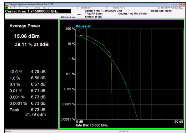
B13_n66(10M)_DFT-s-OFDM_PI_2-BPSK_Edge _1RB_Left_Mid_CH
