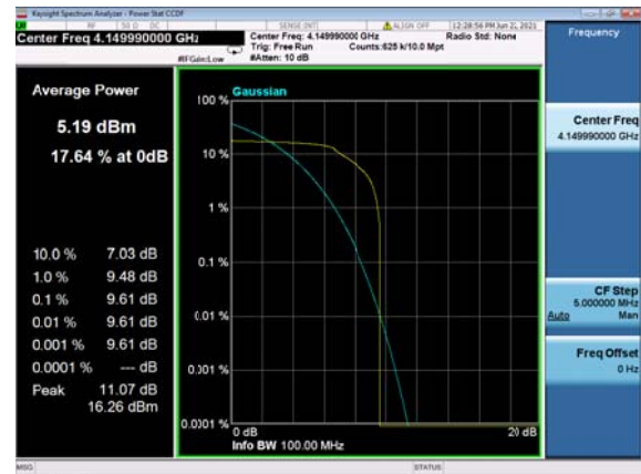
B2_n77(100M)_DFT-s-OFDM_QPSK_Outer_Full _High_CH
