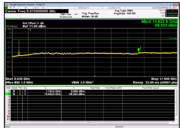
B13_n66(5M)_DFT-s-OFDM_QPSK_Edge_ 1RB_Left_Mid_CH
