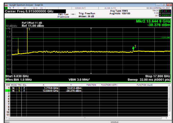
B13_n66(5M)_DFT-s-OFDM_QPSK_Edge_ 1RB_Left_High_CH
