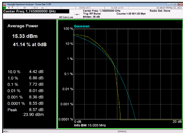
B13_n66(15M)_DFT-s-OFDM_PI_2-BPSK_O uter_Full_Mid_CH
