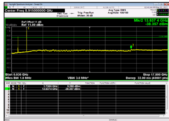
B13_n66(15M)_DFT-s-OFDM_QPSK_Edge_ 1RB_Left_Mid_CH
