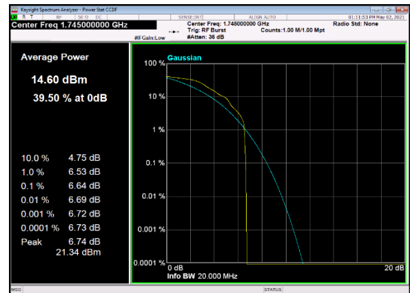
B13_n66(20M)_DFT-s-OFDM_PI_2-BPSK_Edge _1RB_Left_Mid_CH
