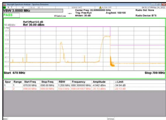
B66_n71(15M)_DFT-s-OFDM_BPSK_Edge_1R B_Right_High_CH
