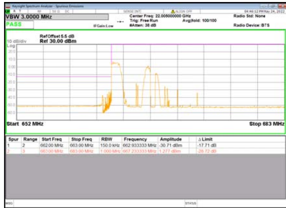
B66_n71(15M)_DFT-s-OFDM_BPSK_Edge_1R B_Left_Low_CH
