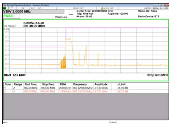
B66_n71(20M)_DFT-s-OFDM_BPSK_Edge_1R B_Left_Low_CH
