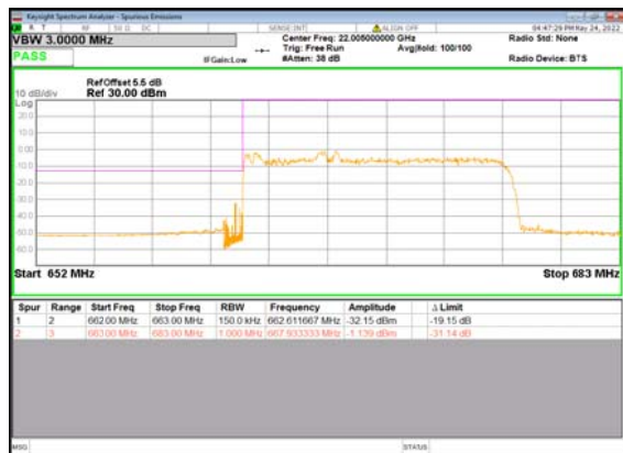
B66_n71(15M)_DFT-s-OFDM_BPSK_Outer_F ull_Low_CH
