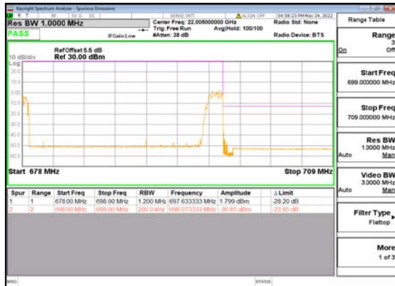
B66_n71(20M)_DFT-s-OFDM_BPSK_Edge_1R B_Right_High_CH
