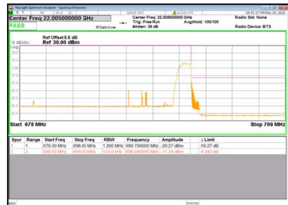
B66_n71(15M)_DFT-s-OFDM_QPSK_Edge_1 RB_Right_High_CH
