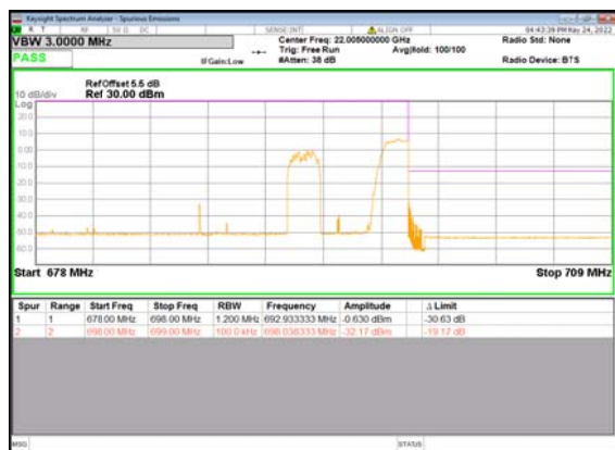
B66_n71(10M)_DFT-s-OFDM_BPSK_Edge_1R B_Right_High_CH
