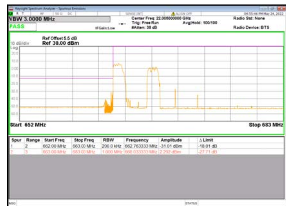
B66_n71(20M)_DFT-s-OFDM_QPSK_Edge_1 RB_Left_Low_CH
