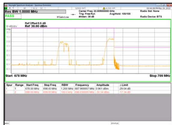
B66_n71(10M)_DFT-s-OFDM_QPSK_Edge_1 RB_Right_High_CH
