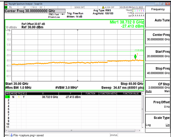
5A_n77(3700-3980MHz) (20GHz-40GHz) 30M DFT-s-OFDM BPSK Edge_1RB_Left Low
