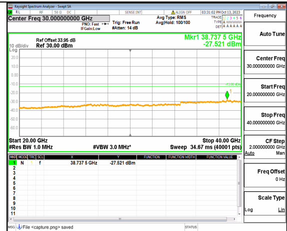
5A_n77(3700-3980MHz) (20GHz-40GHz) 20M DFT-s-OFDM QPSK Edge_1RB_Left High
