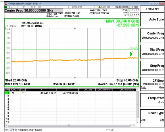
5A_n77(3700-3980MHz) (20GHz-40GHz) 10M DFT-s-OFDM QPSK Edge_1RB_Left High
