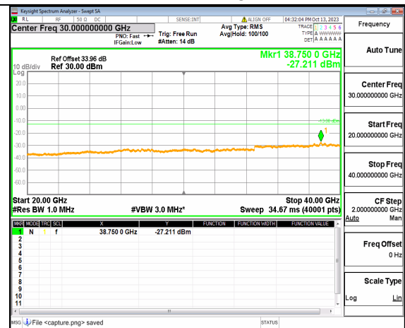
5A_n77(3700-3980MHz) (20GHz-40GHz) 50M DFT-s-OFDM BPSK Edge_1RB_Right Mid
