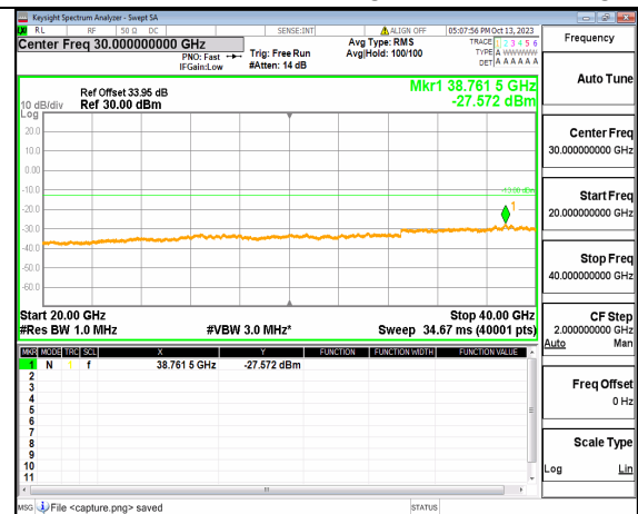
5A_n77(3700-3980MHz) (20GHz-40GHz) 60M DFT-s-OFDM QPSK Edge_1RB_Right High
