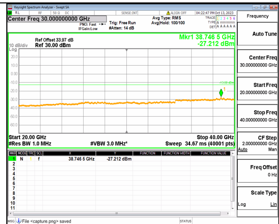
5A_n77(3700-3980MHz) (20GHz-40GHz) 50M DFT-s-OFDM BPSK Edge_1RB_Left Low
