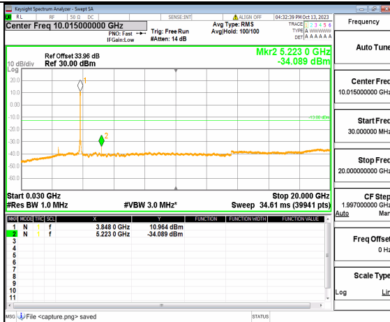
5A_n77(3700-3980MHz) (30MHz-20GHz) 50M DFT-s-OFDM QPSK Outer_Full Mid
