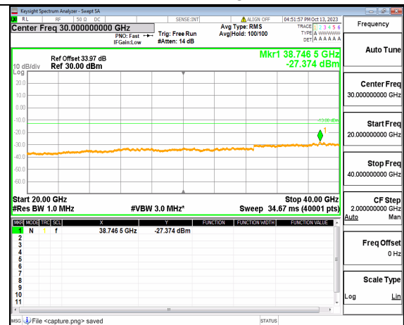
5A_n77(3700-3980MHz) (20GHz-40GHz) 60M DFT-s-OFDM QPSK Edge_1RB_Right Low
