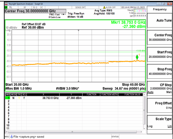
5A_n77(3700-3980MHz) (20GHz-40GHz) 70M DFT-s-OFDM QPSK Edge_1RB_Left Low
