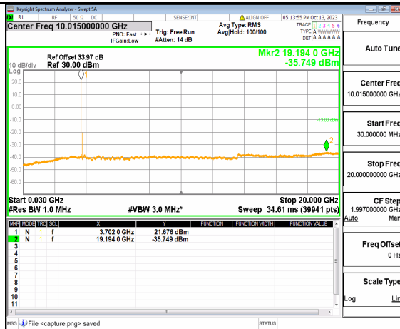
5A_n77(3700-3980MHz) (30MHz-20GHz) 70M DFT-s-OFDM QPSK Edge_1RB_Left Low
