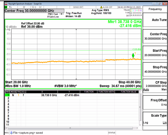
5A_n77(3700-3980MHz) (20GHz-40GHz) 50M DFT-s-OFDM QPSK Outer_Full High
