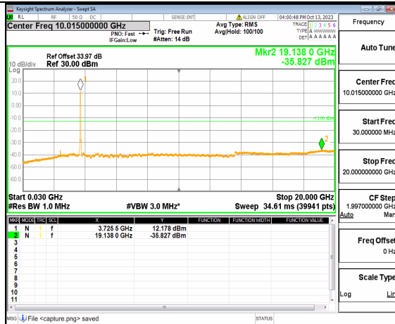
5A_n77(3700-3980MHz) (30MHz-20GHz) 40M DFT-s-OFDM QPSK Outer_Full Low
