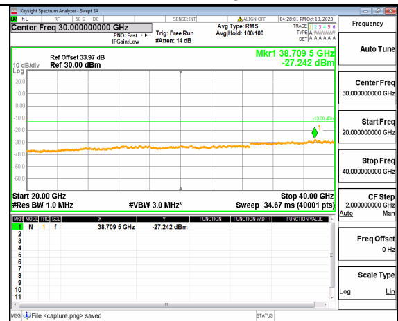
5A_n77(3700-3980MHz) (20GHz-40GHz) 50M DFT-s-OFDM QPSK Edge_1RB_Right Low
