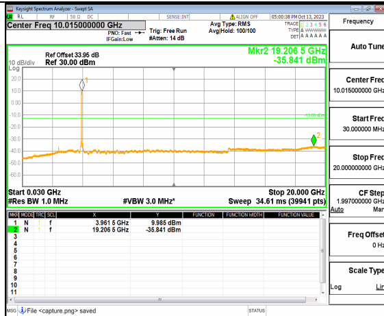
5A_n77(3700-3980MHz) (30MHz-20GHz) 60M DFT-s-OFDM BPSK Outer_Full High
