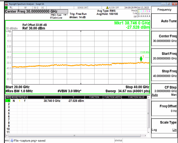
5A_n77(3700-3980MHz) (20GHz-40GHz) 40M DFT-s-OFDM QPSK Outer_Full Mid
