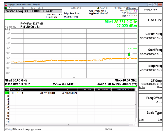
5A_n77(3700-3980MHz) (20GHz-40GHz) 60M DFT-s-OFDM BPSK Edge_1RB_Right Low
