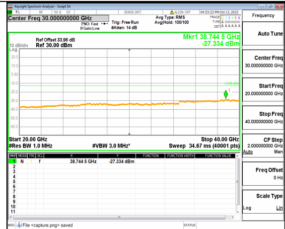
5A_n77(3700-3980MHz) (20GHz-40GHz) 60M DFT-s-OFDM BPSK Outer_Full Mid
