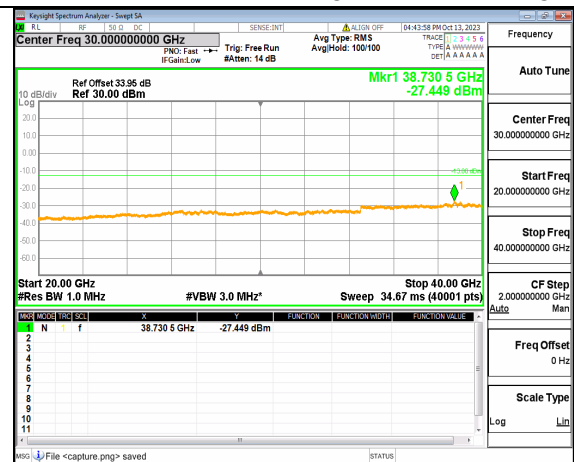
5A_n77(3700-3980MHz) (20GHz-40GHz) 50M DFT-s-OFDM QPSK Edge_1RB_Right High
