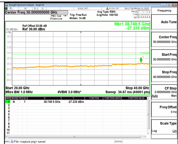
5A_n77(3700-3980MHz) (20GHz-40GHz) 40M DFT-s-OFDM QPSK Outer_Full High
