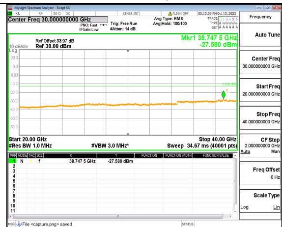
5A_n77(3700-3980MHz) (20GHz-40GHz) 70M DFT-s-OFDM QPSK Edge_1RB_Right Low
