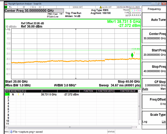
5A_n77(3700-3980MHz) (20GHz-40GHz) 30M DFT-s-OFDM QPSK Outer_Full High
