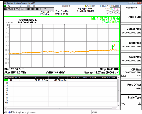
5A_n77(3700-3980MHz) (20GHz-40GHz) 50M DFT-s-OFDM BPSK Outer_Full High
