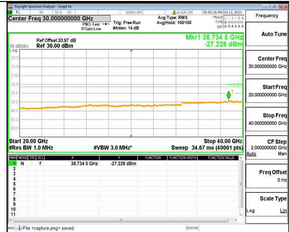
5A_n77(3700-3980MHz) (20GHz-40GHz) 60M DFT-s-OFDM BPSK Outer_Full Low
