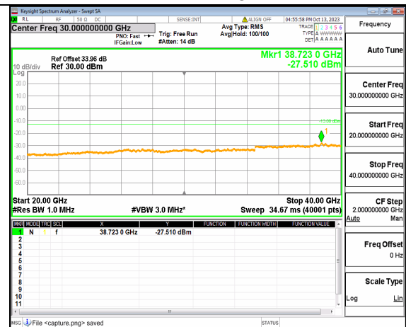
5A_n77(3700-3980MHz) (20GHz-40GHz) 60M DFT-s-OFDM BPSK Edge_1RB_Right Mid
