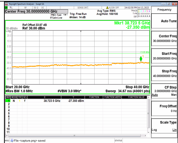
5A_n77(3700-3980MHz) (20GHz-40GHz) 40M DFT-s-OFDM QPSK Edge_1RB_Left Low
