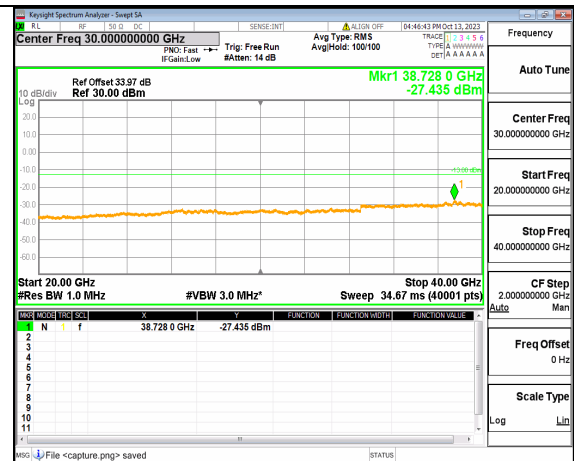
5A_n77(3700-3980MHz) (20GHz-40GHz) 60M DFT-s-OFDM BPSK Edge_1RB_Left Low
