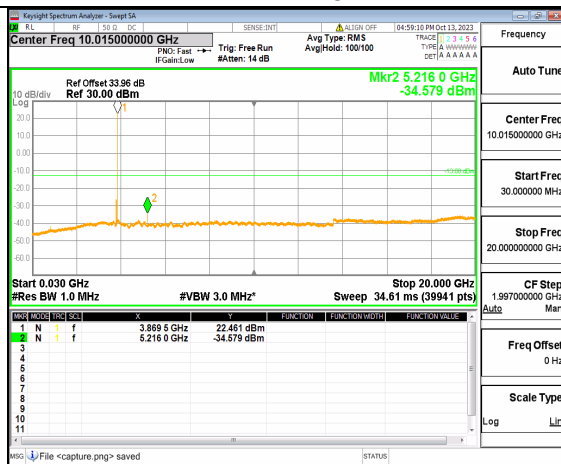
5A_n77(3700-3980MHz) (30MHz-20GHz) 60M DFT-s-OFDM QPSK Edge_1RB_Right Mid
