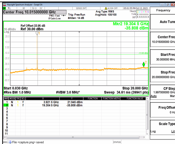
5A_n77(3700-3980MHz) (30MHz-20GHz) 60M DFT-s-OFDM BPSK Edge_1RB_Left High
