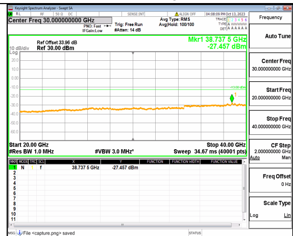
5A_n77(3700-3980MHz) (20GHz-40GHz) 40M DFT-s-OFDM BPSK Edge_1RB_Right Mid
