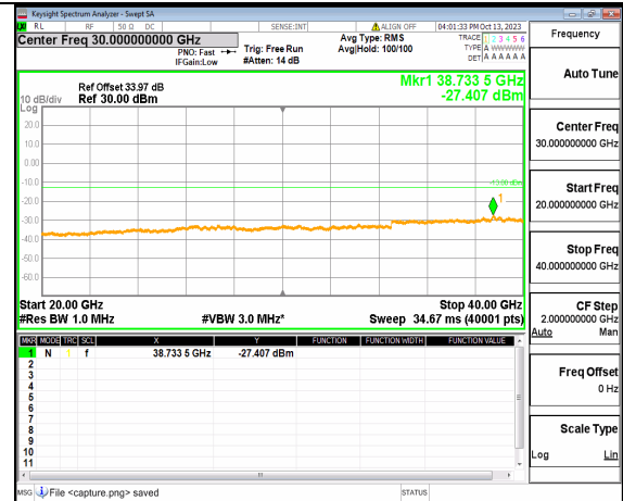
5A_n77(3700-3980MHz) (20GHz-40GHz) 40M DFT-s-OFDM QPSK Outer_Full Low
