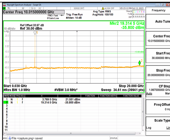
5A_n77(3700-3980MHz) (30MHz-20GHz) 70M DFT-s-OFDM QPSK Edge_1RB_Right Low
