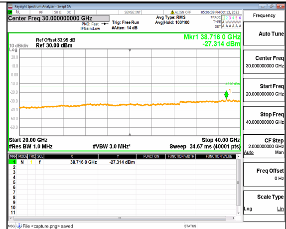
5A_n77(3700-3980MHz) (20GHz-40GHz) 60M DFT-s-OFDM QPSK Edge_1RB_Left High
