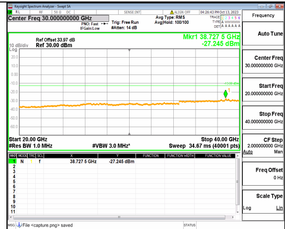
5A_n77(3700-3980MHz) (20GHz-40GHz) 50M DFT-s-OFDM QPSK Edge_1RB_Left Low
