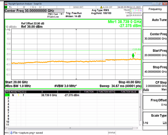
5A_n77(3700-3980MHz) (20GHz-40GHz) 40M DFT-s-OFDM BPSK Outer_Full Mid
