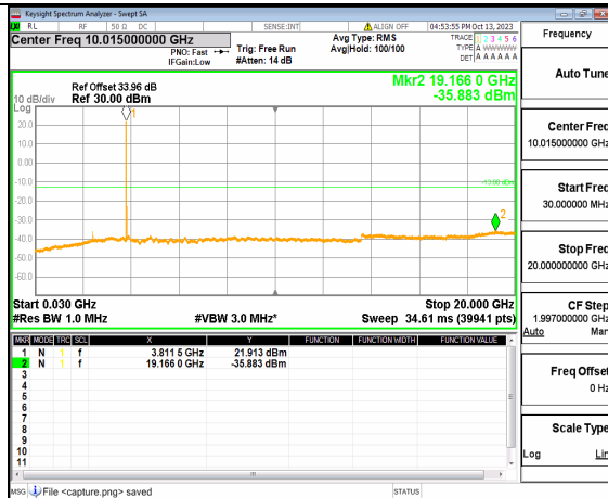
5A_n77(3700-3980MHz) (30MHz-20GHz) 60M DFT-s-OFDM BPSK Edge_1RB_Left Mid
