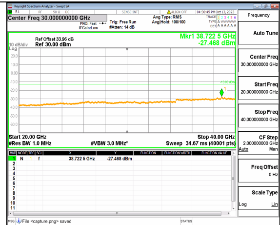
5A_n77(3700-3980MHz) (20GHz-40GHz) 50M DFT-s-OFDM BPSK Edge_1RB_Left Mid
