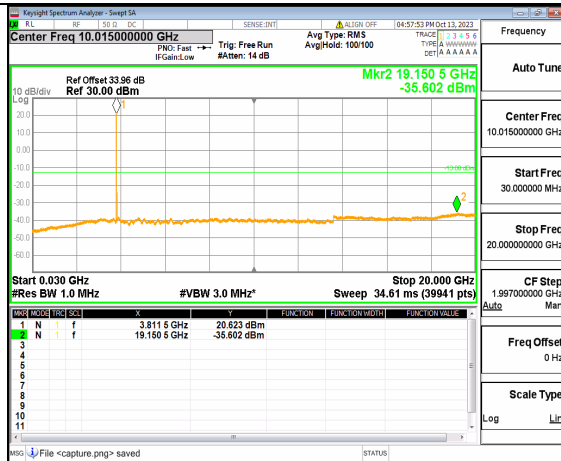
5A_n77(3700-3980MHz) (30MHz-20GHz) 60M DFT-s-OFDM QPSK Edge_1RB_Left Mid
