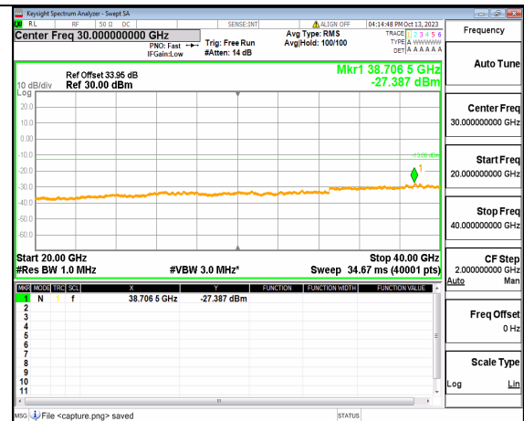
5A_n77(3700-3980MHz) (20GHz-40GHz) 40M DFT-s-OFDM BPSK Edge_1RB_Left High
