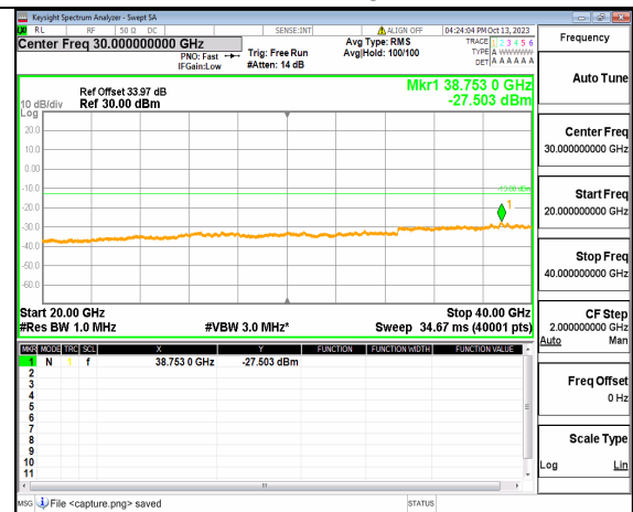
5A_n77(3700-3980MHz) (20GHz-40GHz) 50M DFT-s-OFDM BPSK Edge_1RB_Right Low
