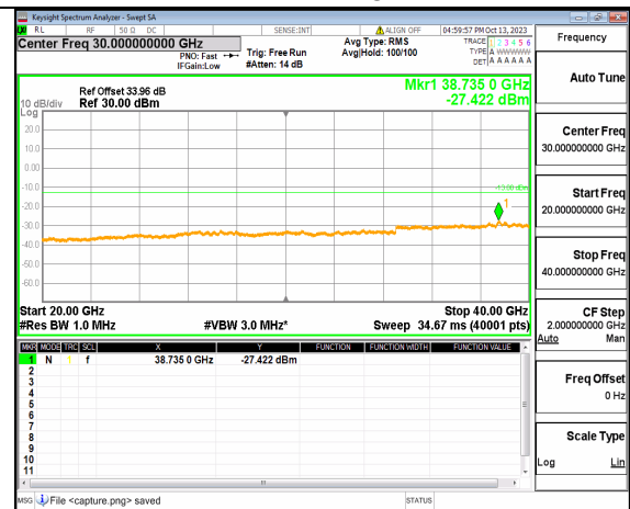
5A_n77(3700-3980MHz) (20GHz-40GHz) 60M DFT-s-OFDM QPSK Edge_1RB_Right Mid
