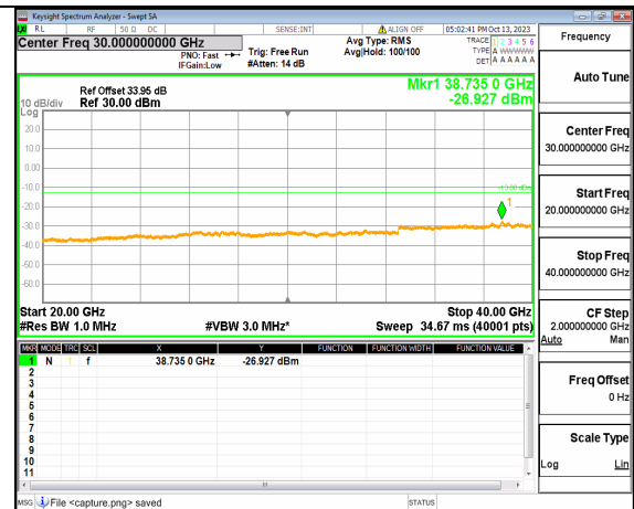
5A_n77(3700-3980MHz) (20GHz-40GHz) 60M DFT-s-OFDM BPSK Edge_1RB_Left High
