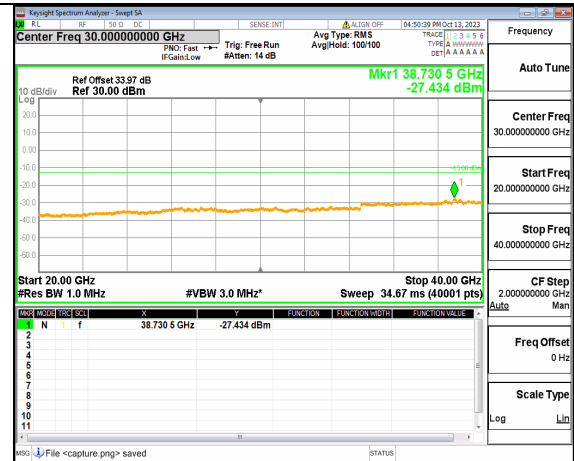
5A_n77(3700-3980MHz) (20GHz-40GHz) 60M DFT-s-OFDM QPSK Edge_1RB_Left Low
