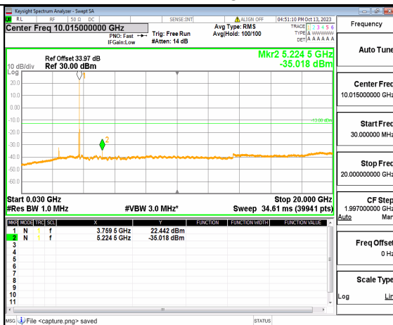
5A_n77(3700-3980MHz) (30MHz-20GHz) 60M DFT-s-OFDM QPSK Edge_1RB_Right Low
