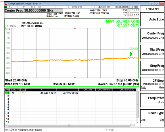
5A_n77(3700-3980MHz) (20GHz-40GHz) 60M DFT-s-OFDM QPSK Edge_1RB_Left Mid
