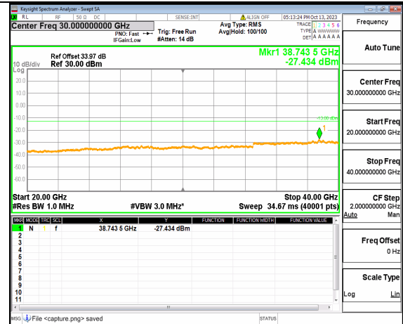
5A_n77(3700-3980MHz) (20GHz-40GHz) 70M DFT-s-OFDM QPSK Outer_Full Low
