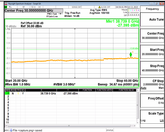
5A_n77(3700-3980MHz) (20GHz-40GHz) 60M DFT-s-OFDM BPSK Edge_1RB_Left Mid
