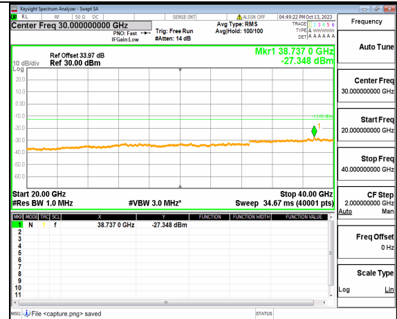
5A_n77(3700-3980MHz) (20GHz-40GHz) 60M DFT-s-OFDM QPSK Outer_Full Low
