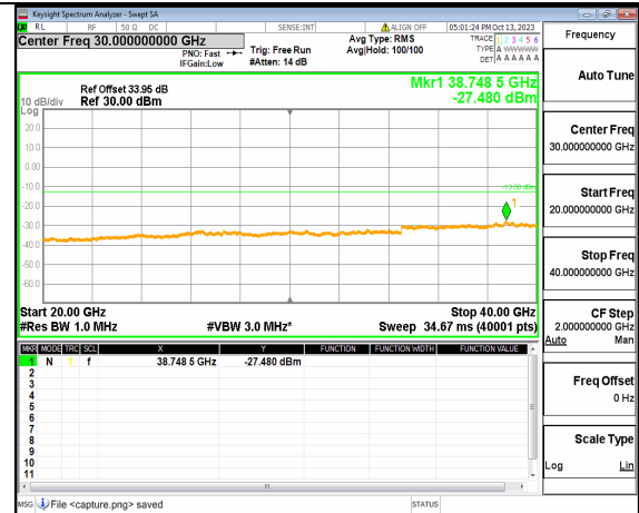
5A_n77(3700-3980MHz) (20GHz-40GHz) 60M DFT-s-OFDM BPSK Outer_Full High
