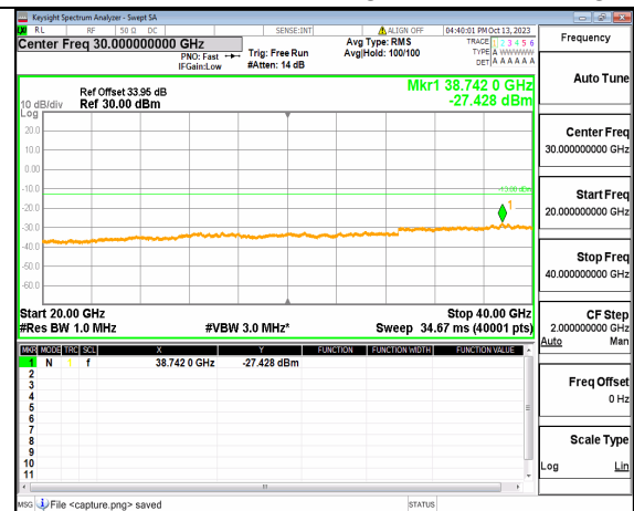
5A_n77(3700-3980MHz) (20GHz-40GHz) 50M DFT-s-OFDM BPSK Edge_1RB_Right High
