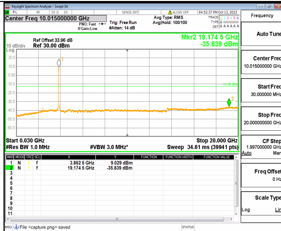
5A_n77(3700-3980MHz) (30MHz-20GHz) 60M DFT-s-OFDM BPSK Outer_Full Mid
