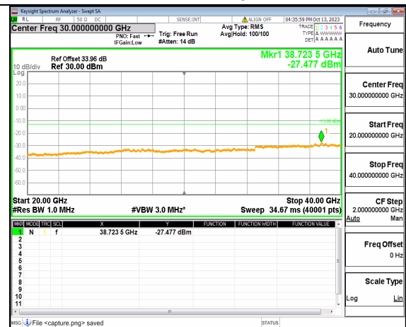
5A_n77(3700-3980MHz) (20GHz-40GHz) 50M DFT-s-OFDM QPSK Edge_1RB_Right Mid
