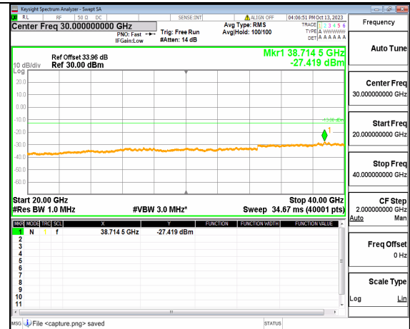
5A_n77(3700-3980MHz) (20GHz-40GHz) 40M DFT-s-OFDM BPSK Edge_1RB_Left Mid
