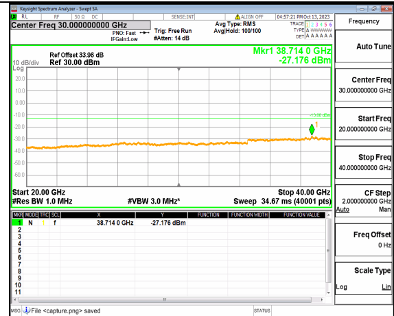
5A_n77(3700-3980MHz) (20GHz-40GHz) 60M DFT-s-OFDM QPSK Outer_Full Mid
