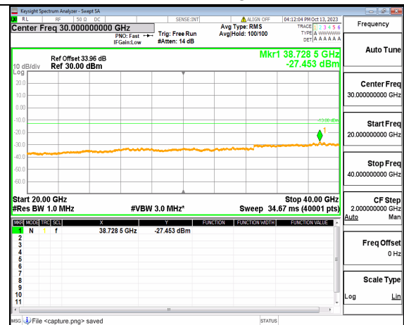
5A_n77(3700-3980MHz) (20GHz-40GHz) 40M DFT-s-OFDM QPSK Edge_1RB_Right Mid
