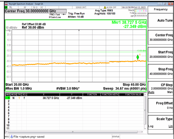
5A_n77(3700-3980MHz) (20GHz-40GHz) 90M DFT-s-OFDM QPSK Edge_1RB_Left Mid
