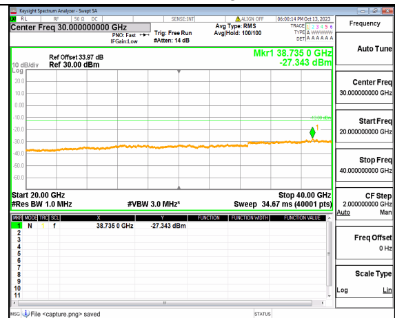
5A_n77(3700-3980MHz) (20GHz-40GHz) 90M DFT-s-OFDM BPSK Edge 1RB Right Low
