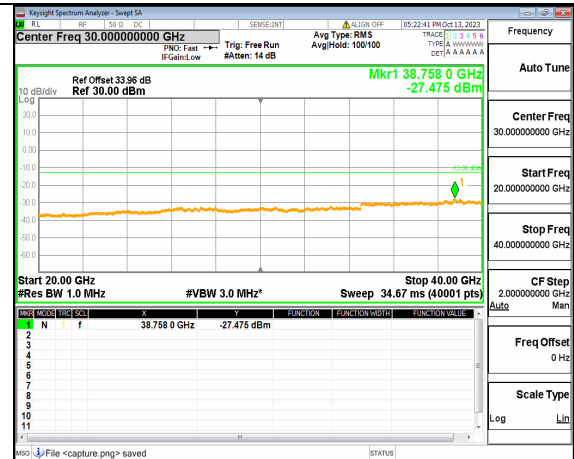
5A_n77(3700-3980MHz) (20GHz-40GHz) 70M DFT-s-OFDM QPSK Edge_1RB_Left Mid
