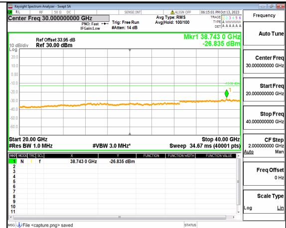
5A_n77(3700-3980MHz) (20GHz-40GHz) 90M DFT-s-OFDM BPSK Edge_1RB_Left High
