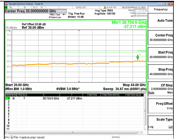
5A_n77(3700-3980MHz) (20GHz-40GHz) 100M DFT-s-OFDM QPSK Edge_1RB_Left Mid
