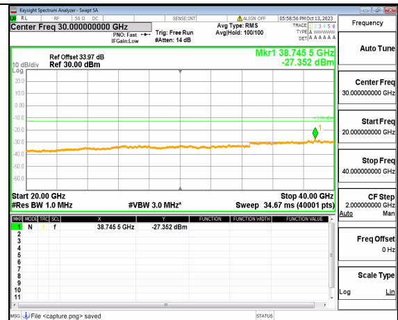
5A_n77(3700-3980MHz) (20GHz-40GHz) 90M DFT-s-OFDM BPSK Edge_1RB Left Low
