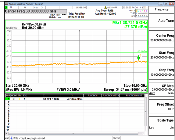
5A_n77(3700-3980MHz) (20GHz-40GHz) 80M DFT-s-OFDM BPSK Edge_1RB_Left High
