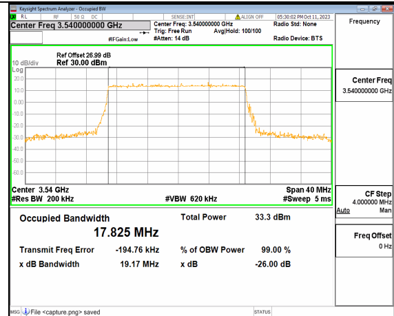
5A_n77(3450-3550MHz) 20M DFT-s-OFDM QPSK Outer_Full High
