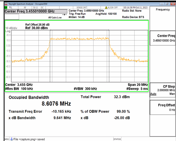
5A_n77(3450-3550MHz) 10M DFT-s-OFDM QPSK Outer_Full Low
