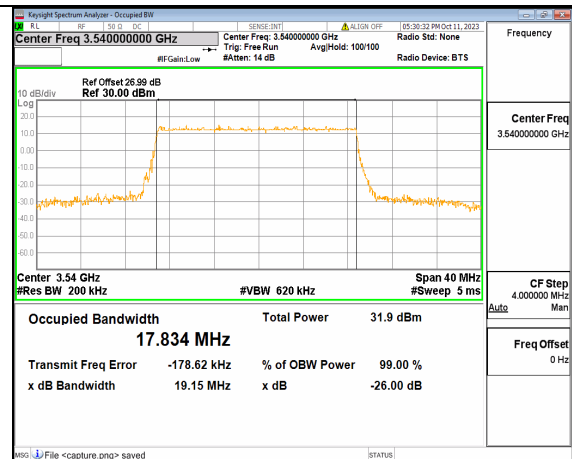
5A_n77(3450-3550MHz) 20M DFT-s-OFDM 64QAM Outer_Full High
