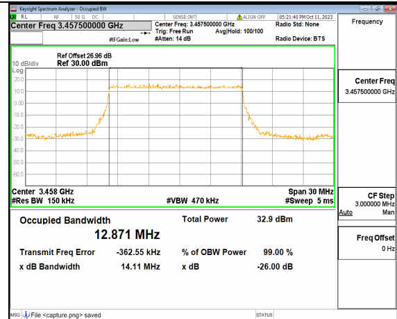
5A_n77(3450-3550MHz) 15M DFT-s-OFDM QPSK Outer_Full Low
