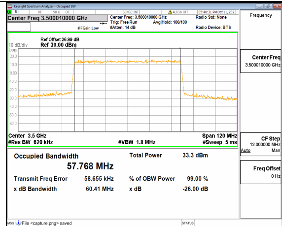
5A_n77(3450-3550MHz) 60M DFT-s-OFDM QPSK Outer_Full Mid
