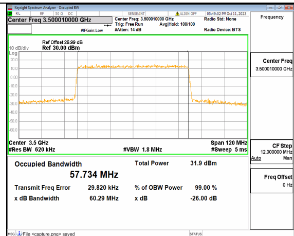
5A_n77(3450-3550MHz) 60M DFT-s-OFDM 64QAM Outer_Full Mid
