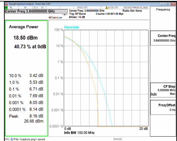
5A_n77(3700-3980MHz) 100M DFT-s-OFDM 256QAM Outer_Full Mid
