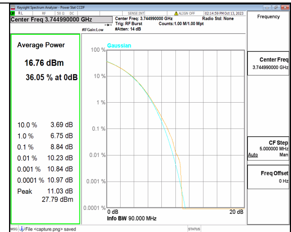
5A_n77(3700-3980MHz) 90M CP-OFDM 256QAM Outer_Full Low
