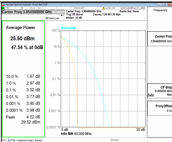
5A_n77(3700-3980MHz) 50M DFT-s-OFDM BPSK Outer_Full High
