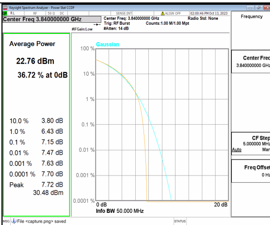
5A_n77(3700-3980MHz) 50M CP-OFDM QPSK Outer_Full Mid
