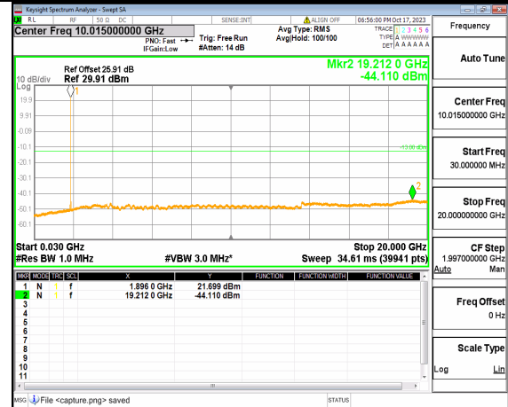
5A_n2 (30MHz-20GHz) 15M DFT-s-OFDM BPSK Edge_1RB_Left High
