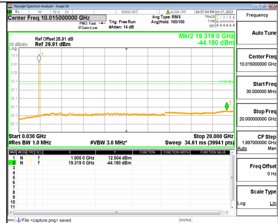
5A_n2 (30MHz-20GHz) 15M DFT-s-OFDM QPSK Outer_Full High
