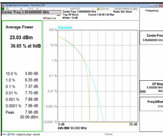
5A_n77(3700-3980MHz) 50M CP-OFDM QPSK Outer_Full High
