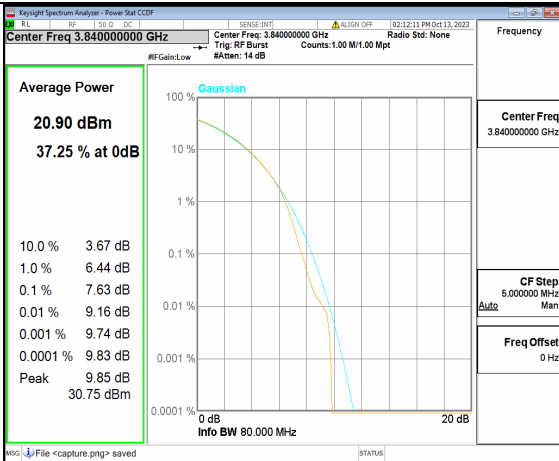
5A_n77(3700-3980MHz) 80M CP-OFDM QPSK Outer_Full Mid
