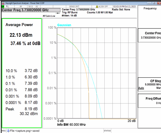
5A_n77(3700-3980MHz) 60M CP-OFDM QPSK Outer_Full Low
