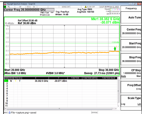
5A_n77(3450-3550MHz) (20GHz-36GHz) 70M DFT-s-OFDM QPSK Edge_1RB_Right High
