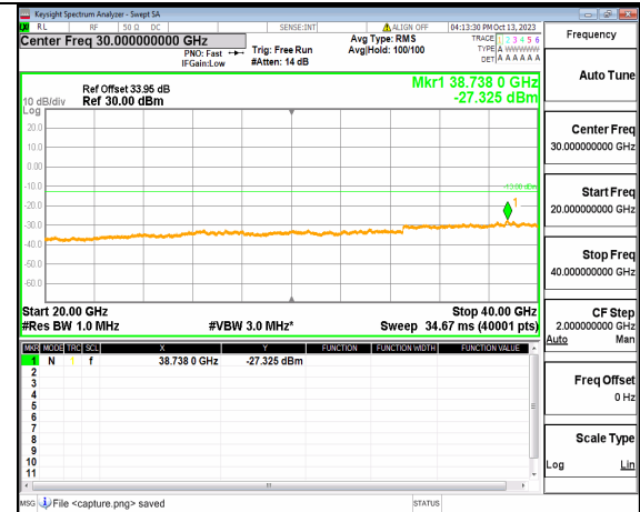
5A_n77(3700-3980MHz) (20GHz-40GHz) 40M DFT-s-OFDM BPSK Outer_Full High
