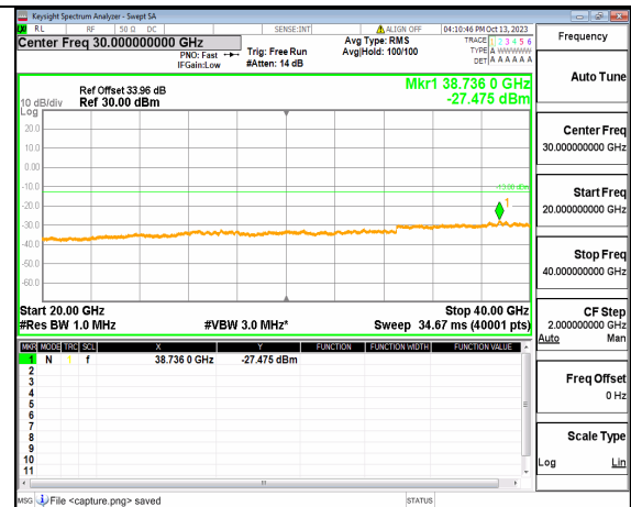
5A_n77(3700-3980MHz) (20GHz-40GHz) 40M DFT-s-OFDM QPSK Edge_1RB_Left Mid
