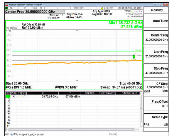
5A_n77(3700-3980MHz) (20GHz-40GHz) 40M DFT-s-OFDM BPSK Edge_1RB_Right High
